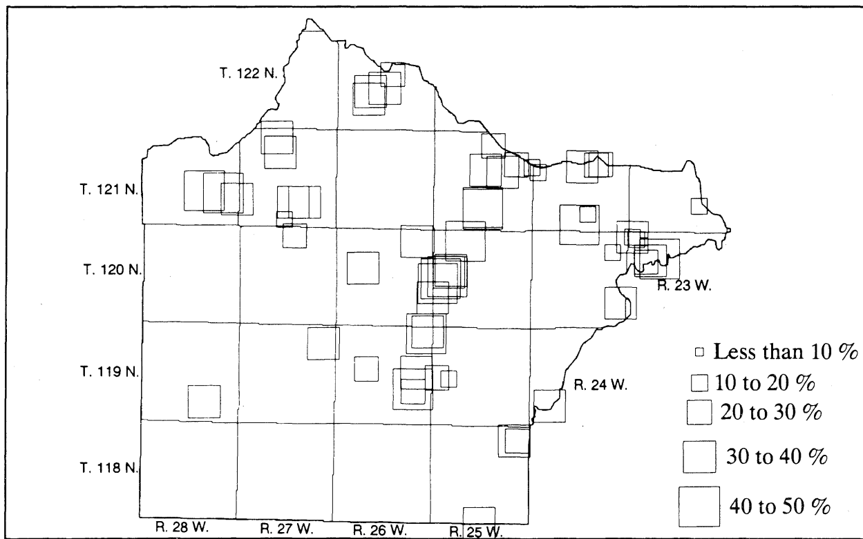
Figure 7. Average percent gravel (+ 4 mesh) for MN/DOT-identified aggregate sources
