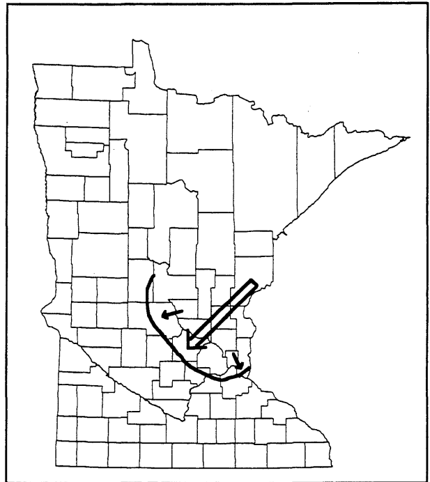
Figure 2. Maximum extent and generalized flow direction of the late Wisconsinan Superior lobe
