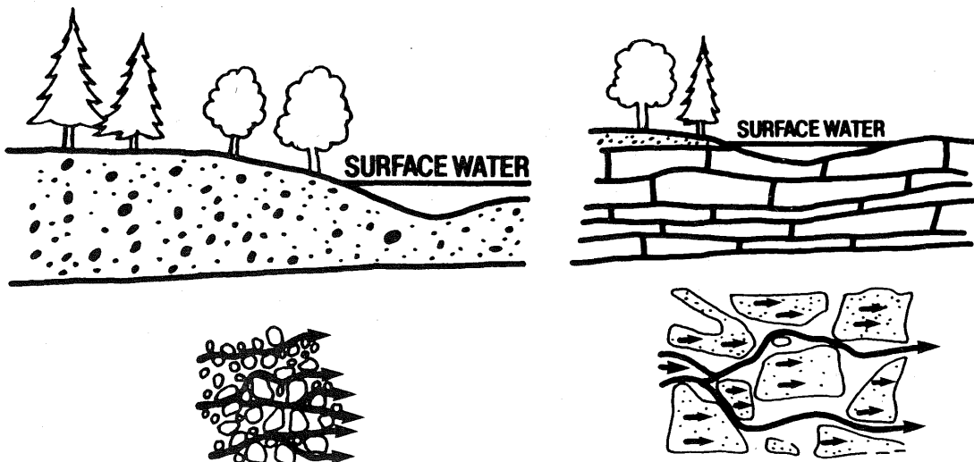
Figure 2: Storage and movement of ground water.
