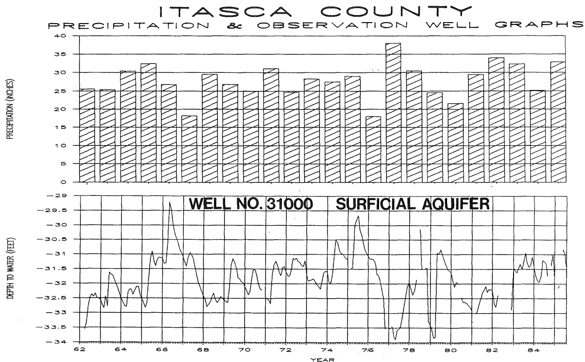
Hydrograph No. 10
