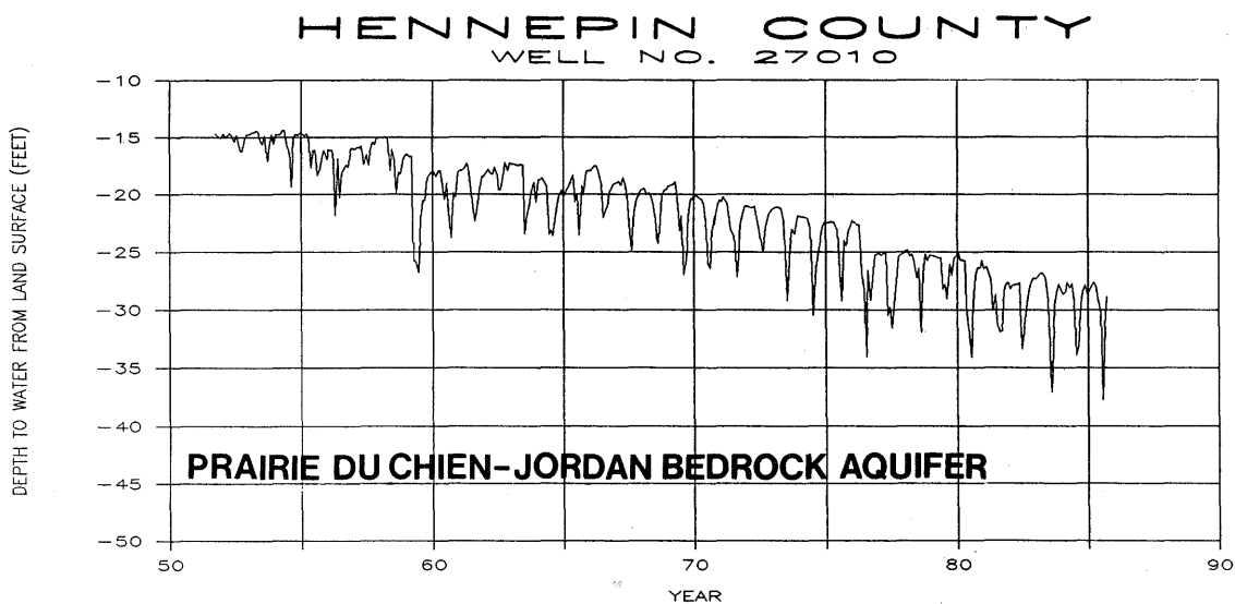
Hydrograph No. 12
