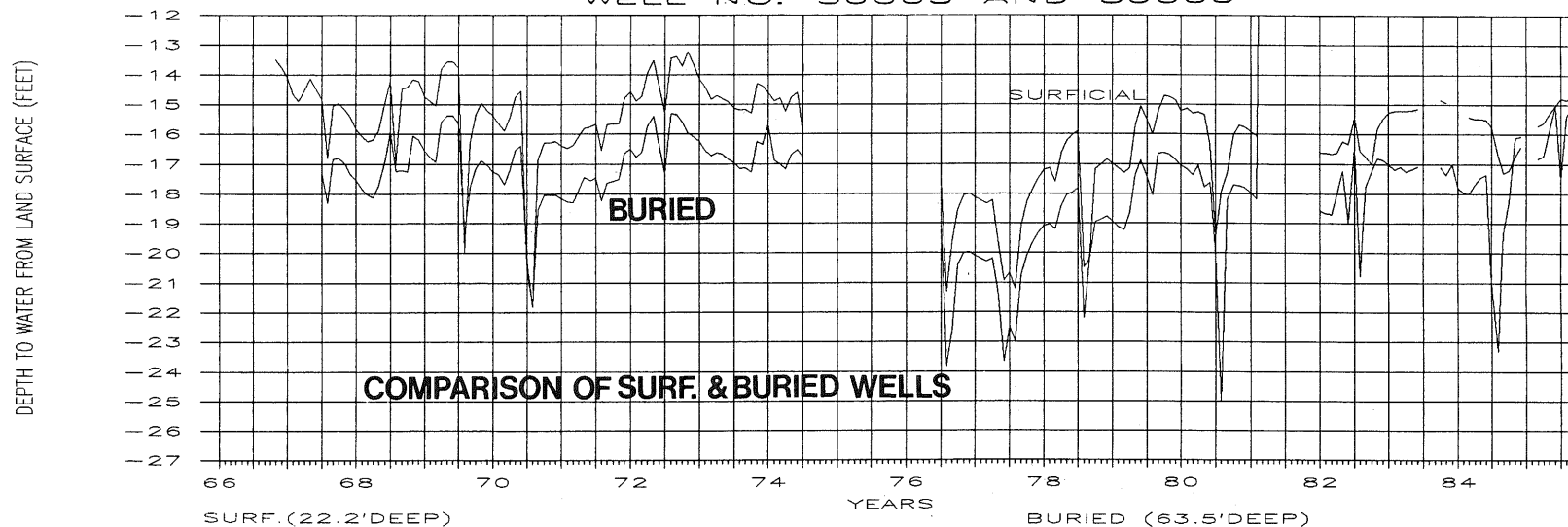
Hydrograph No. 6
