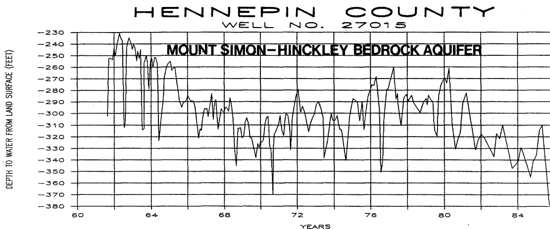
Hydrograph No. 11
