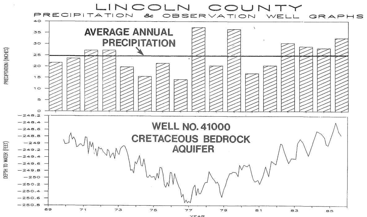
Hydrograph No. 8
