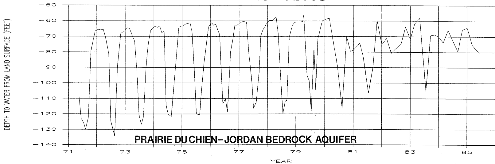
Hydrograph No. 5
