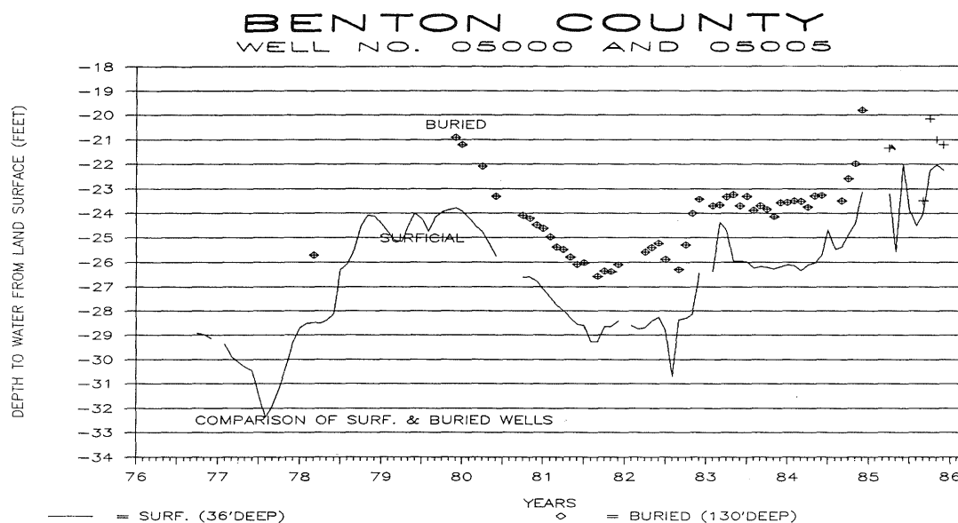
Hydrograph No. 7
