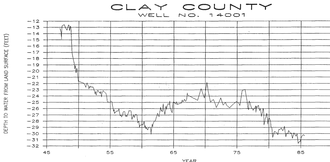
Hydrograph No. 13
