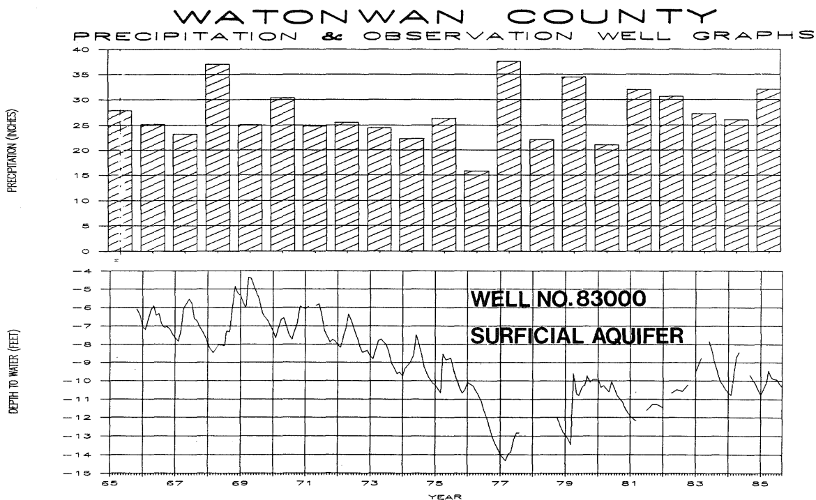
Hydrograph No. 9
