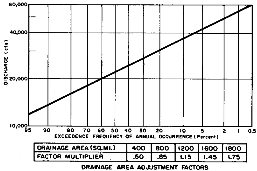
FIGURE 2-32 Peak Discharge Frequency Curve, Planning Sub-area 5.1, Genesee River at Portageville, N.Y. (961 Sq. Mi. Drainage Area)
