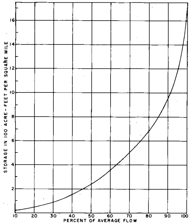
FIGURE 2-78 Generalized Storage Yield Relationship, Planning Subarea 5.2, Fall Creek Near Ithaca, N.Y. (126 Sq. Mi. Drainage Area)
