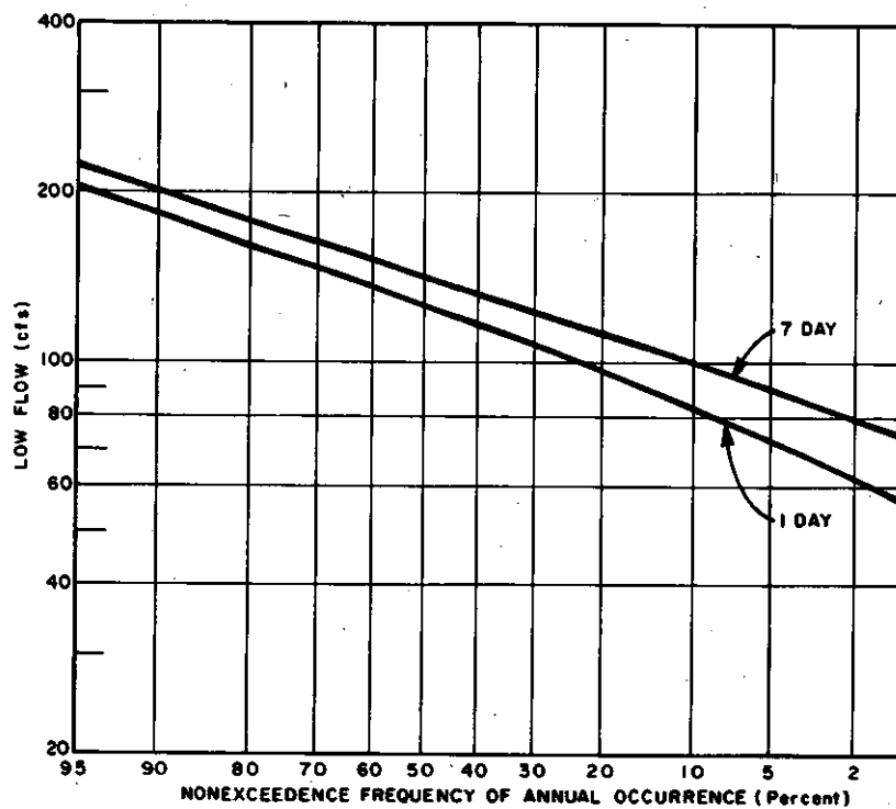
FIGURE 2-37 Low Flow Discharge Frequency Curves, Planning Subarea 2.1, Little Wolf River at Royalton, Wis. (514 Sq. Mi. Drainage Area)
