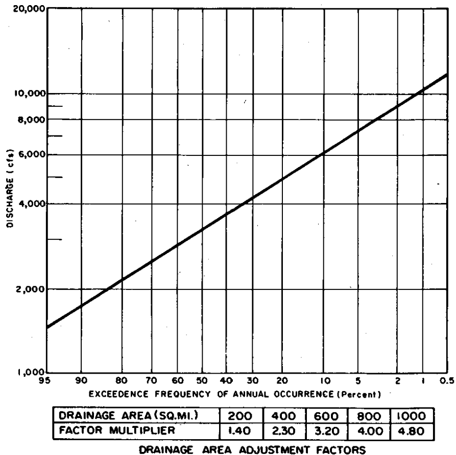
FIGURE 2-33 Peak Discharge Frequency Curve, Planning Sub-area 5.2, Fall Creek Near Ithaca, N.Y. (126 Sq. Mi. Drainage Area)
