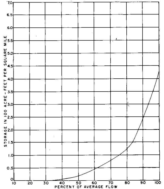
FIGURE 2-70 Generalized Storage Yield Relationship, Planning Subarea 2.4, Muskegon River at Evart, Mich. (1,450 Sq. Mi. Drainage Area)
