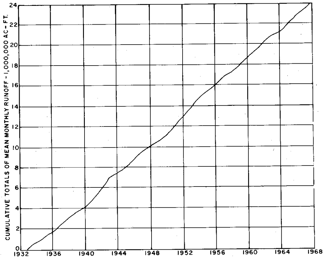
FIGURE 2-55 Mass Curve of Runoff, Planning Subarea 2.4, Muskegon River at Evart, Mich.
