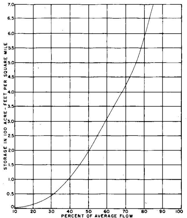
FIGURE 2-72 Generalized Storage Yield Relationship, Planning Subarea 3.2, Flint River at Fosters, Mich. (1,120 Sq. Mi. Drainage Area)
