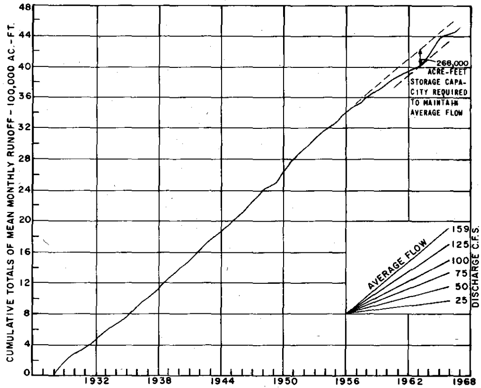
FIGURE 2-50 Mass Curve of Runoff, Planning Subarea 1.1, Baptism River at Beaver Bay, Minn.
