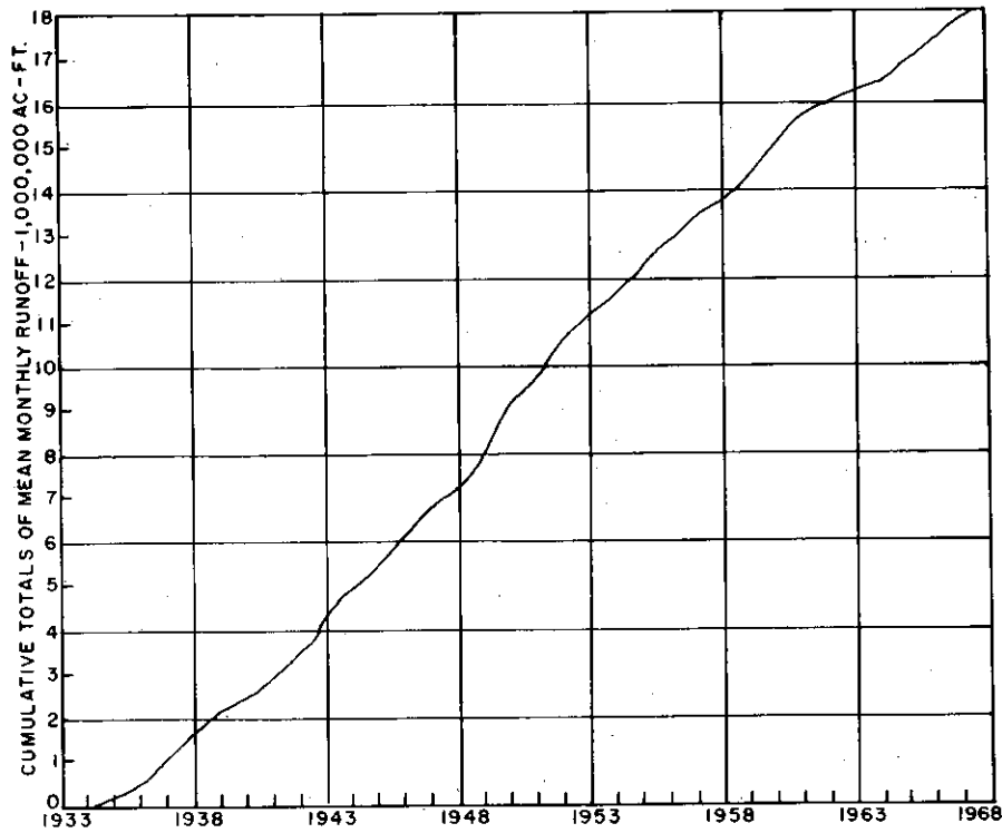
FIGURE 2-54 Mass Curve of Runoff, Planning Subarea 2.3, Grand River at Lansing, Mich.
