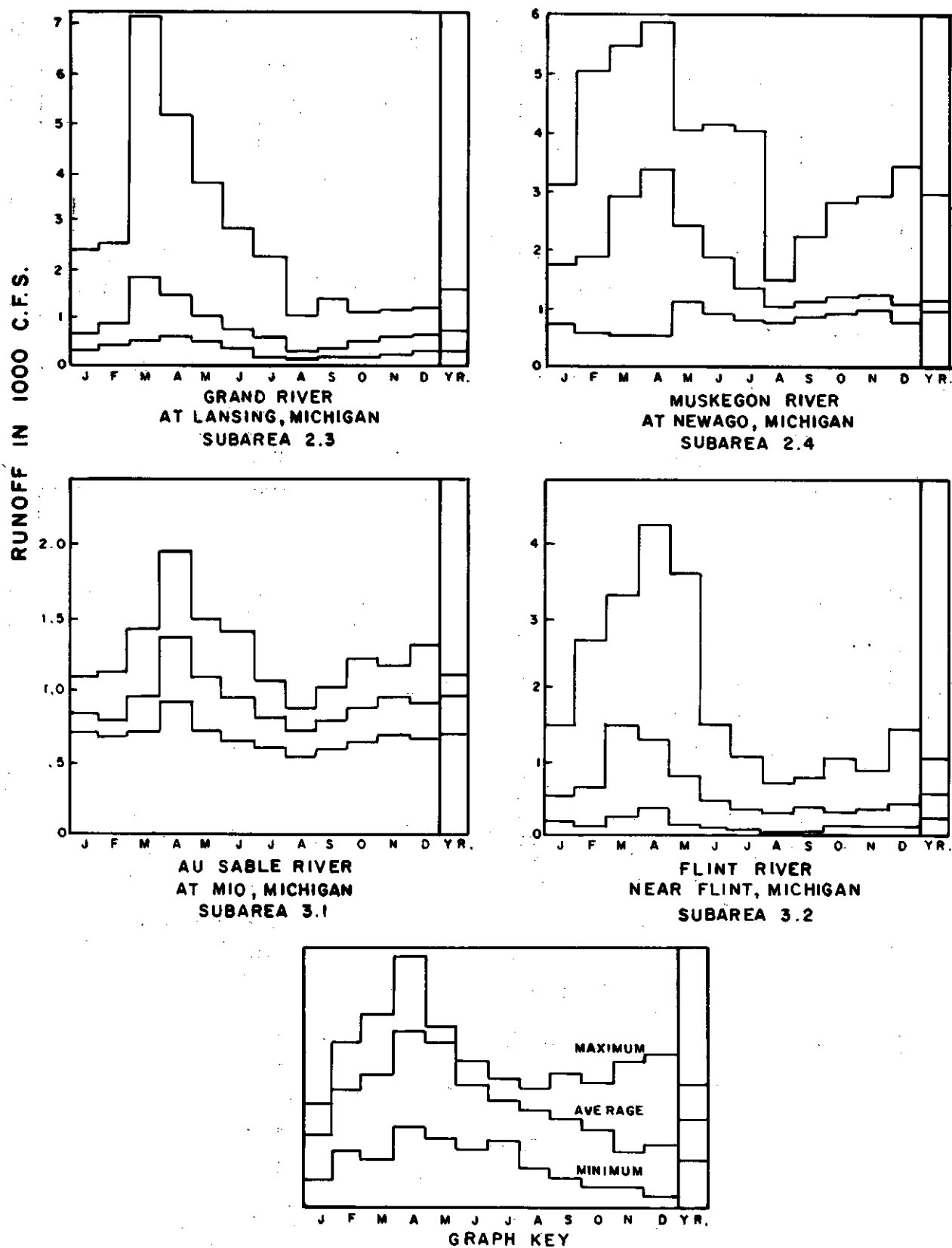
FIGURE 2-17 Monthly Distribution of Runoff, Planning Subareas 2.3, 2.4, 3.1, and 3.2
