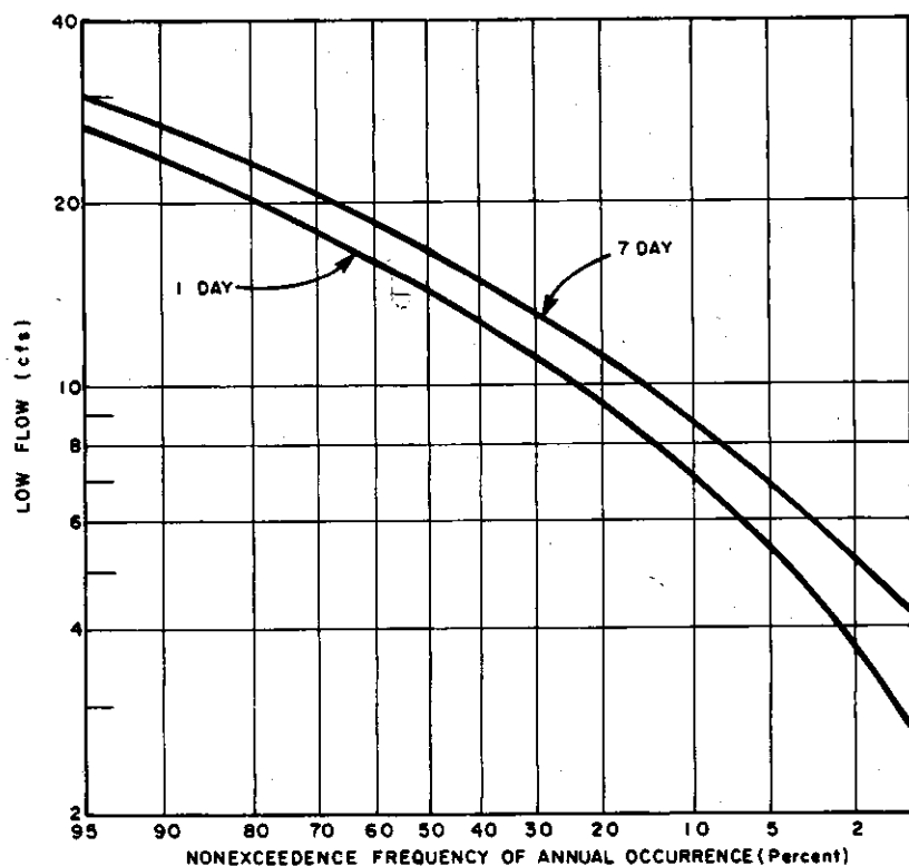
FIGURE 2-48 Low Flow Discharge Frequency Curves, Planning Subarea 5.2, Fall Creek Near Ithaca, N.Y. (126 Sq. Mi. Drainage Area)
