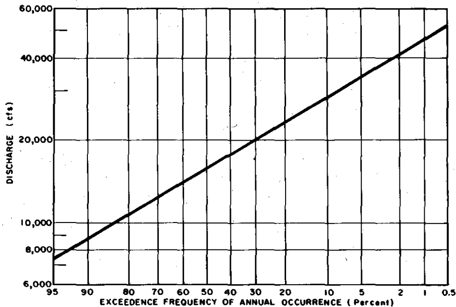
FIGURE 2-30 Peak Discharge Frequency Curve, Planning Sub-area 4.3, Grand River at Madison, Ohio (581 Sq. Mi. Drainage Area)
