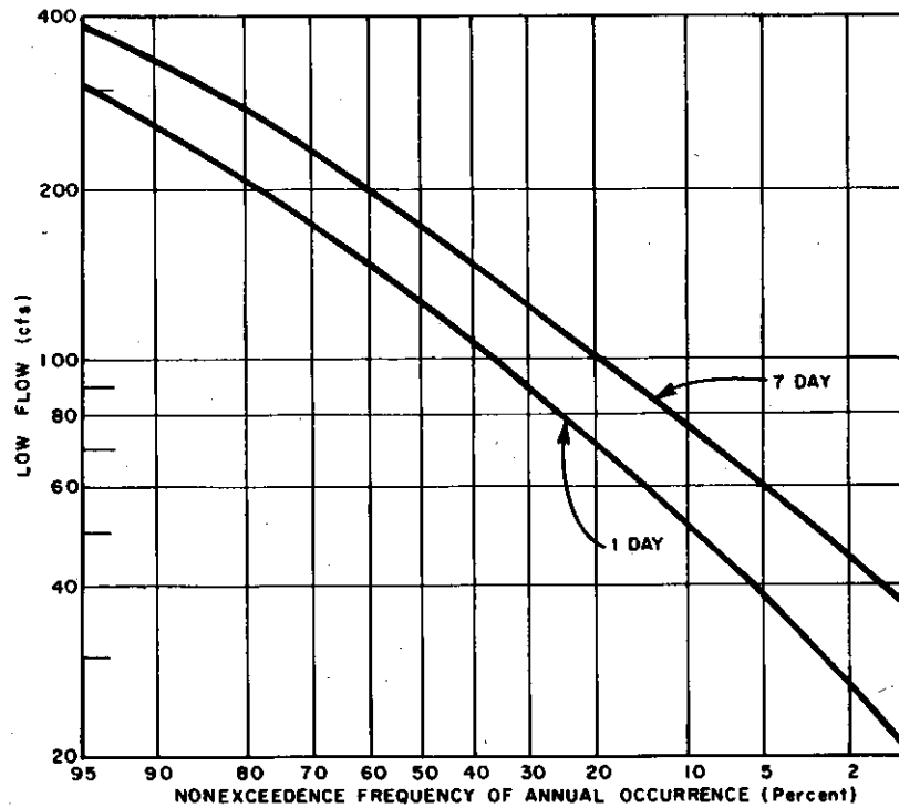
FIGURE 2-44 Low Flow Discharge Frequency Curves, Planning Subarea 4.2, Maumee River at Waterville, Ohio (6,329 Sq. Mi. Drainage Area)
