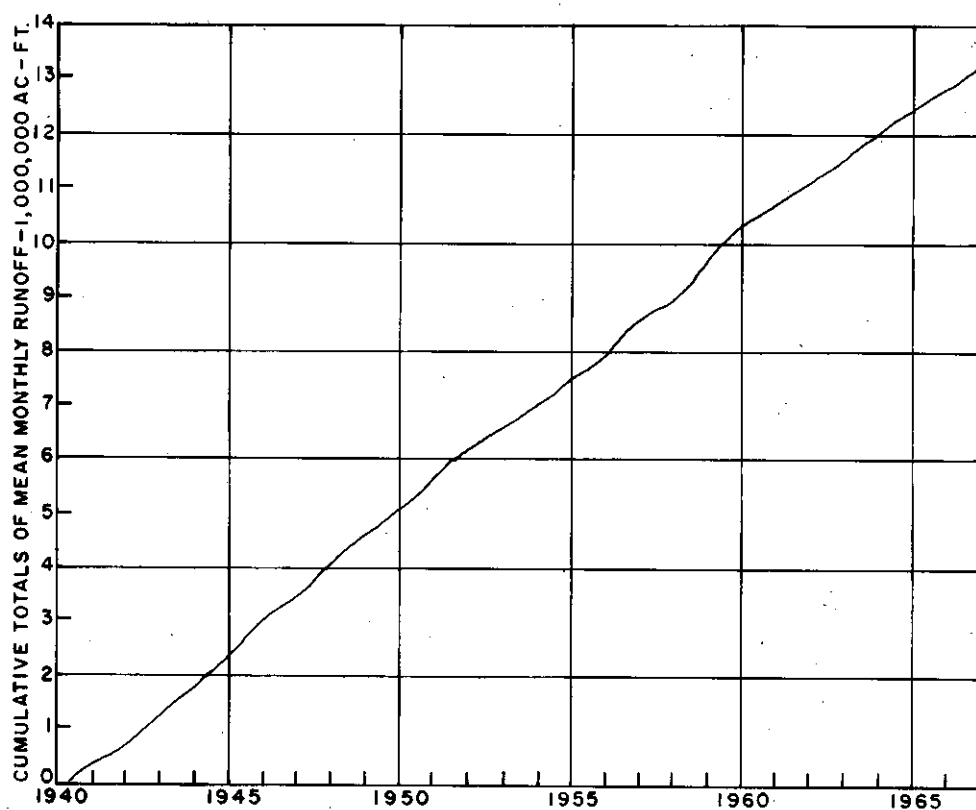
FIGURE 2-61 Mass Curve of Runoff, Planning Subarea 4.4, Cattaraugus Creek at Gowanda, N.Y.
