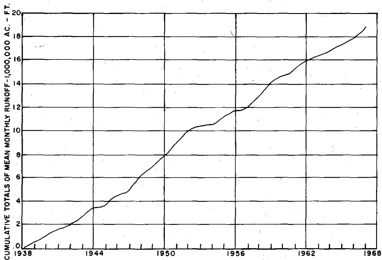
FIGURE 2-59 Mass Curve of Runoff, Planning Subarea 4.2, Sandusky River at Fremont, Ohio
