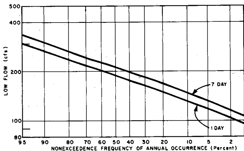
FIGURE 2-49 Low Flow Discharge Frequency Curves, Planning Subarea 5.3, St. Regis River at Brasher Center, N.Y. (616 Sq. Mi. Drainage Area)
