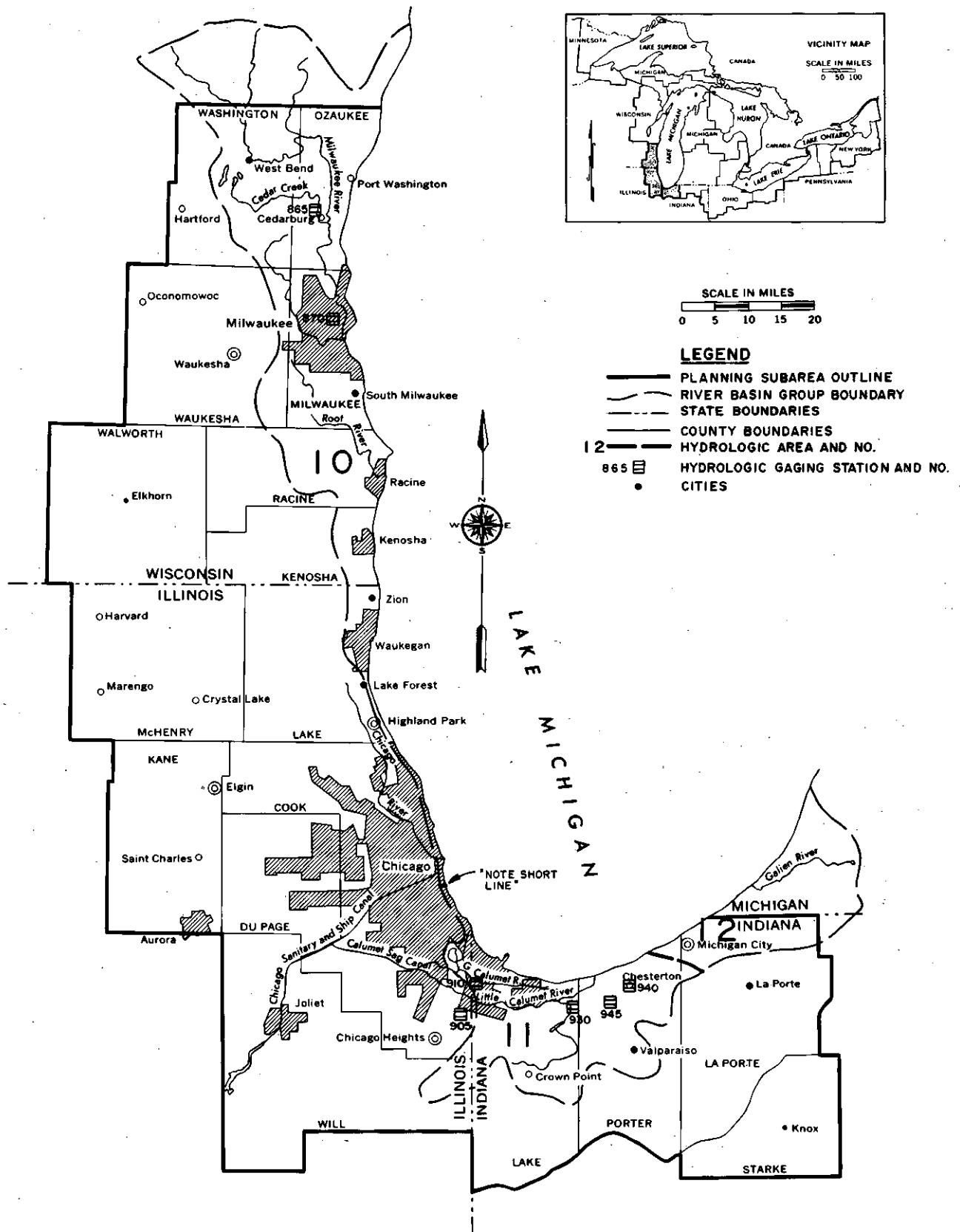
FIGURE 2-4 Hydrologic Gaging Stations, Planning Subarea 2.2
