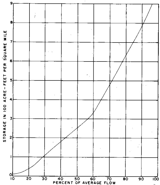
FIGURE 2-66 Generalized Storage Yield Relationship, Planning Subarea 1.2 Sturgeon River Near Sidnaw, Mich. (171 Sq. Mi. Drainage Area)
