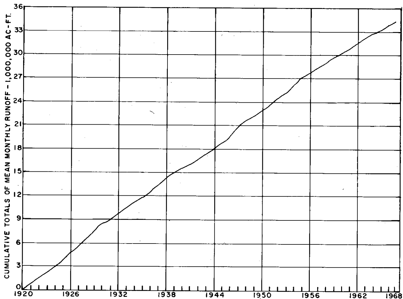
FIGURE 2-64 Mass Curve of Runoff, Planning Subarea 5.3, St. Regis River at Brasher Center, N.Y.
