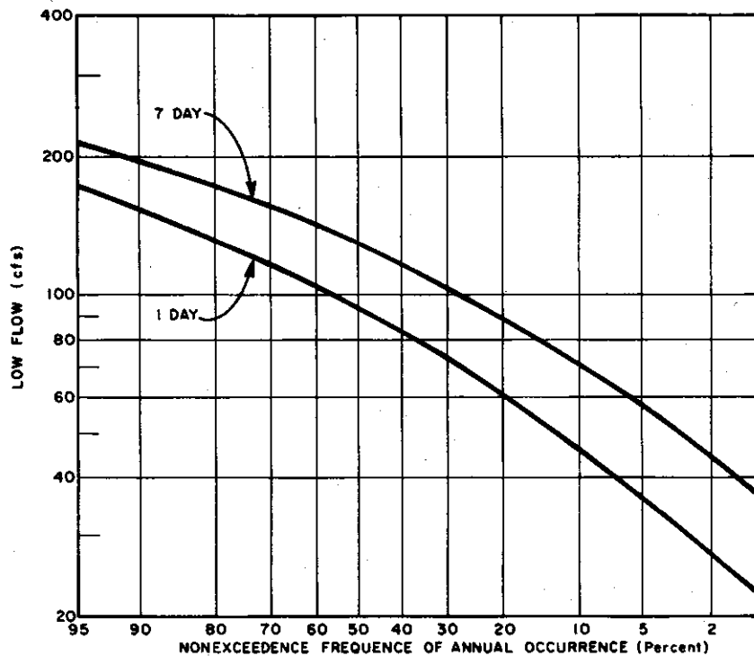
FIGURE 2-39 Low Flow Discharge Frequency Curves, Planning Subarea 2.3, Grand River at Lansing, Mich. (1,230 Sq. Mi. Drainage Area)
