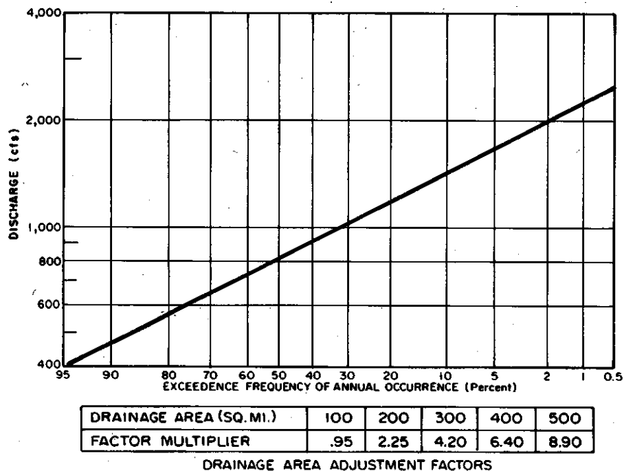
FIGURE 2-20 Peak Discharge Frequency Curve, Planning Sub-area 1.1, Poplar River at Lutsen, Minn. (114 Sq. Mi. Drainage Area)
