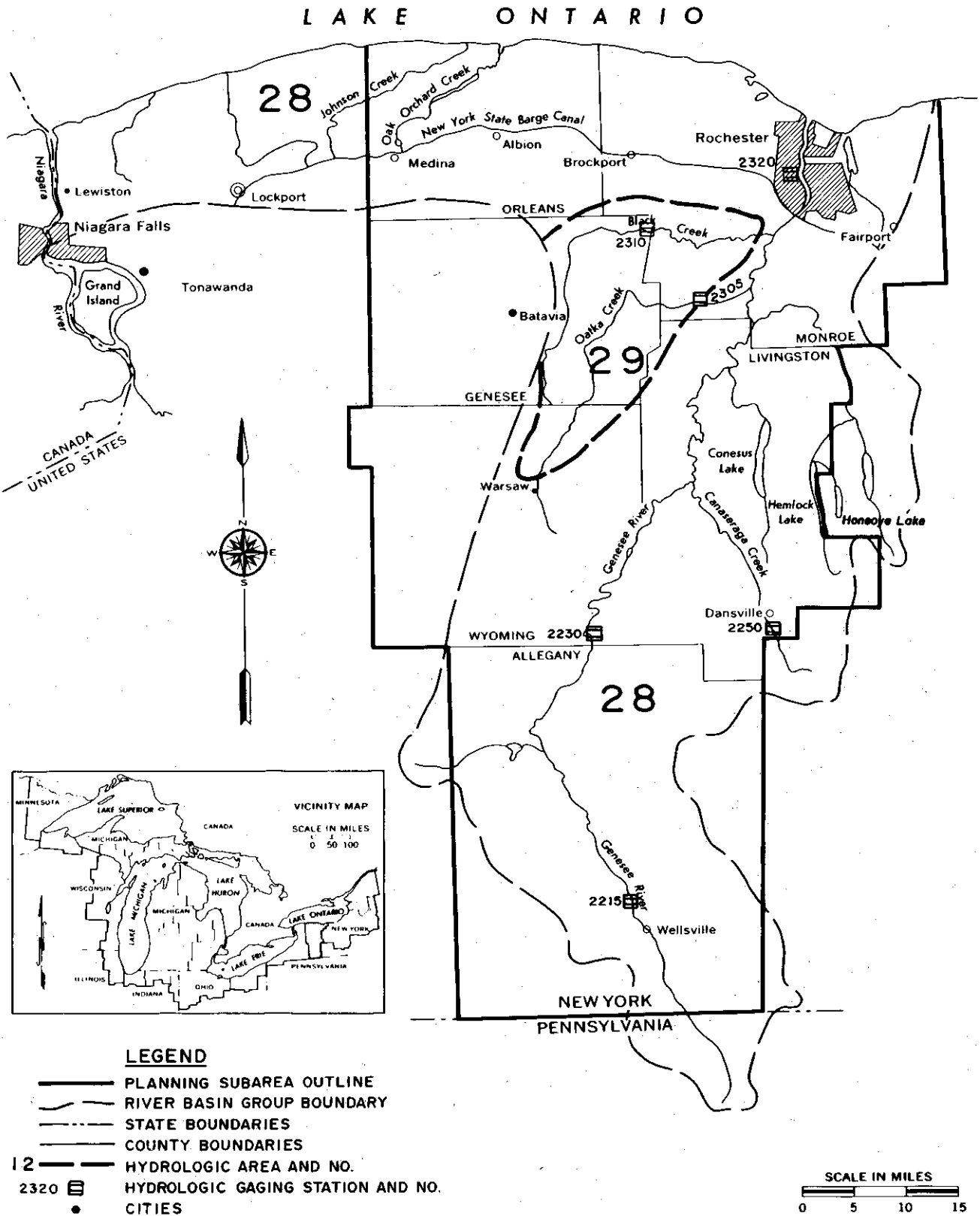
FIGURE 2-13 Hydrologic Gaging Stations, Planning Subarea 5.1
