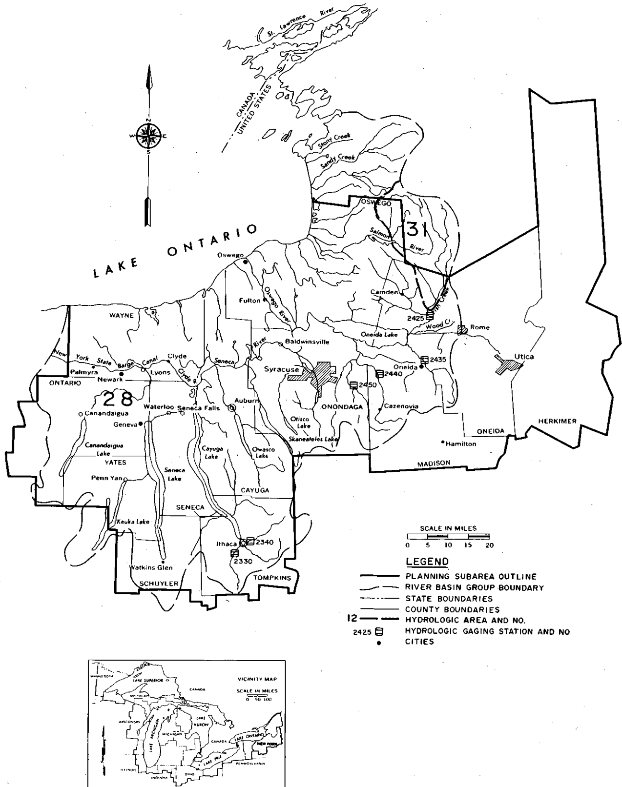
FIGURE 2-14 Hydrologic Gaging Stations, Planning Subarea 5.2
