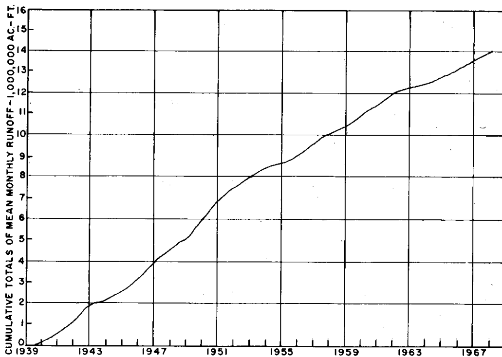
FIGURE 2-57 Mass Curve of Runoff, Planning Subarea 3.2, Flint River at Fosters, Mich.
