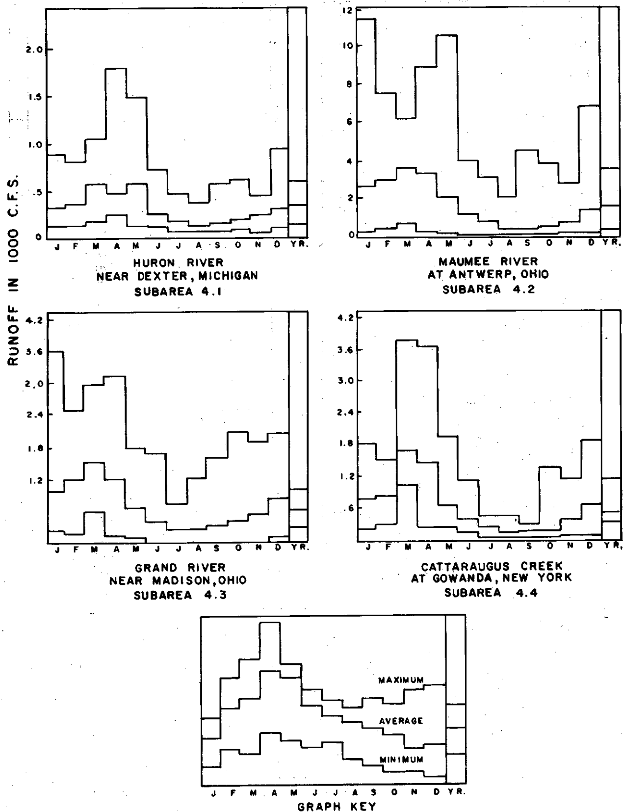
FIGURE 2-18 Monthly Distribution of Runoff, Planning Subareas 4.1, 4.2, 4.3, and 4.4
