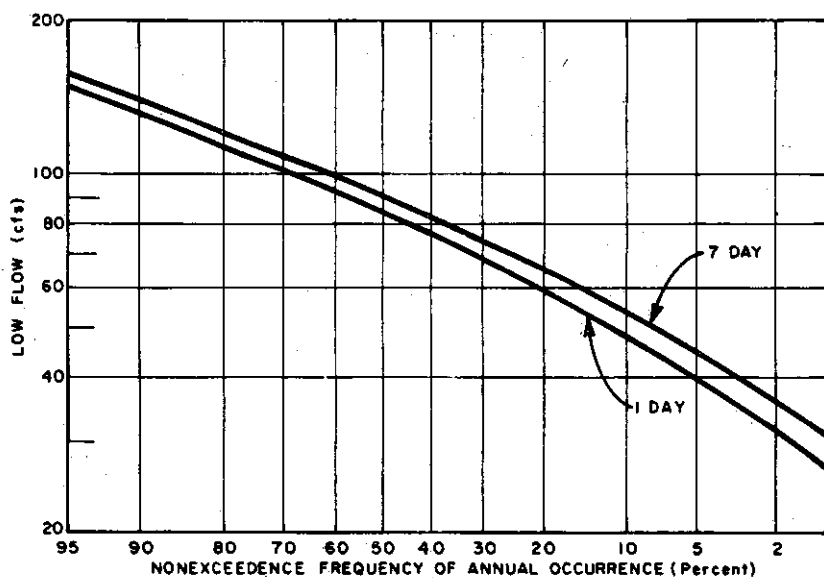
FIGURE 2-43 Low Flow Discharge Frequency Curves, Planning Subarea 4.1, Huron River Near Dexter, Mich. (506 Sq. Mi. Drainage Area)
