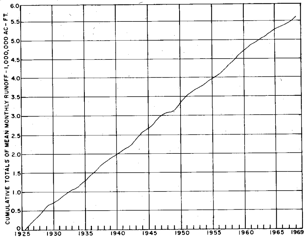
FIGURE 2-63 Mass Curve of Runoff, Planning Subarea 5.2, Fall Creek Near Ithaca, N.Y.
