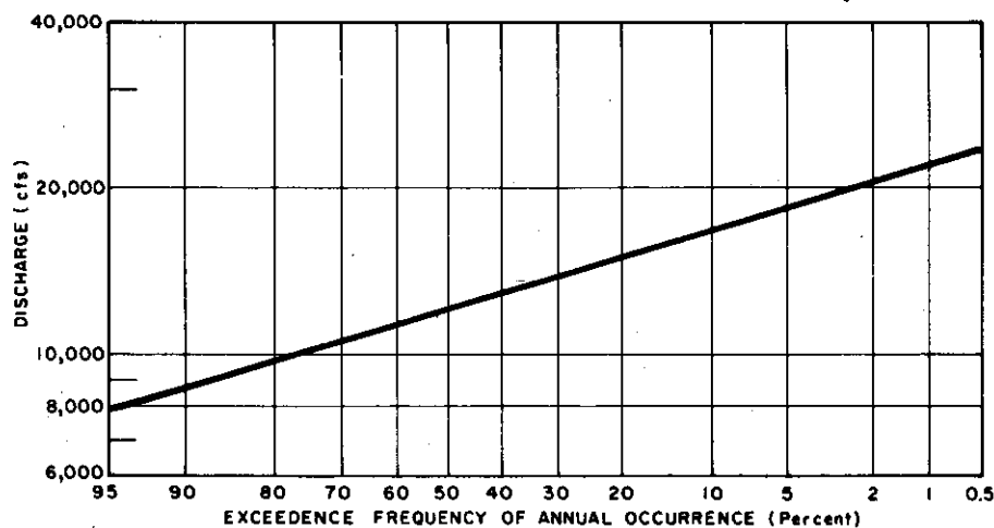
FIGURE 2-28 Peak Discharge Frequency Curve, Planning Sub-area 4.1, Clinton River at Mt. Clemens, Mich. (734 Sq. Mi. Drainage Area)
