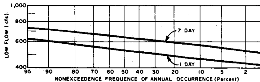
FIGURE 2-41 Low Flow Discharge Frequency Curves, Planning Subarea 3.1, Au Sable River at Mio, Mich. (1,100 Sq. Mi. Drainage Area)
