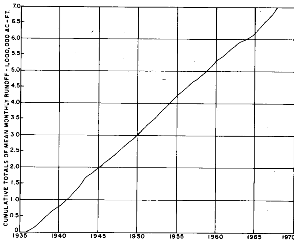
FIGURE 2-56 Mass Curve of Runoff, Planning Subarea 3.1, Rifle River at Sterling, Mich.
