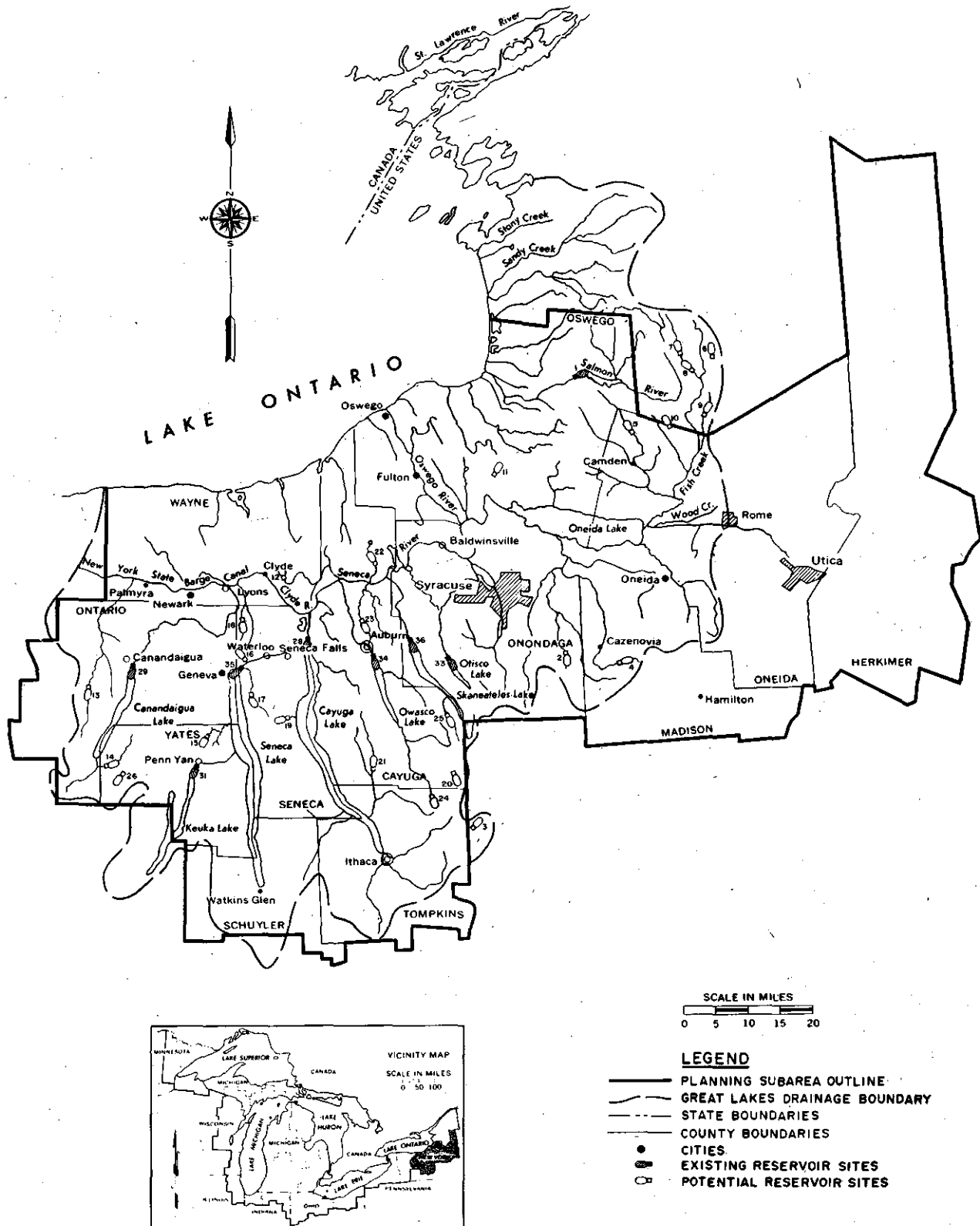
FIGURE 2-93 Reservoir Site Map, Planning Subarea 5.2
