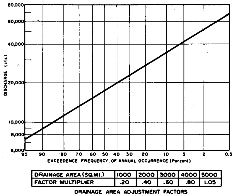
FIGURE 2-24 Peak Discharge Frequency Curve, Planning Sub-area 2.3, Grand River at Grand Rapids, Mich. (4,900 Sq. Mi. Drainage Area)
