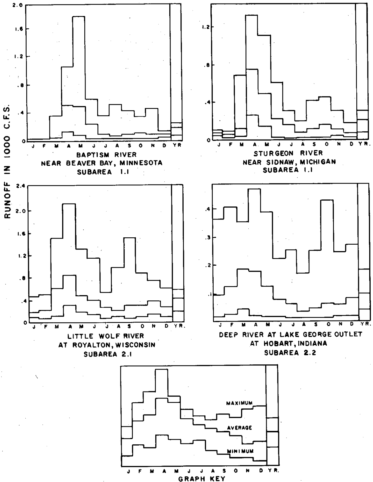
FIGURE 2-16 Monthly Distribution of Runoff, Planning Subareas 1.1, 1.2, 2.1, and 2.2
