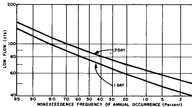
FIGURE 2-46 Low Flow Discharge Frequency Curves, Planning Subarea 4.4, Cattaraugus Creek at Gowanda, N.Y. (432 Sq. Mi. Drainage Area)
