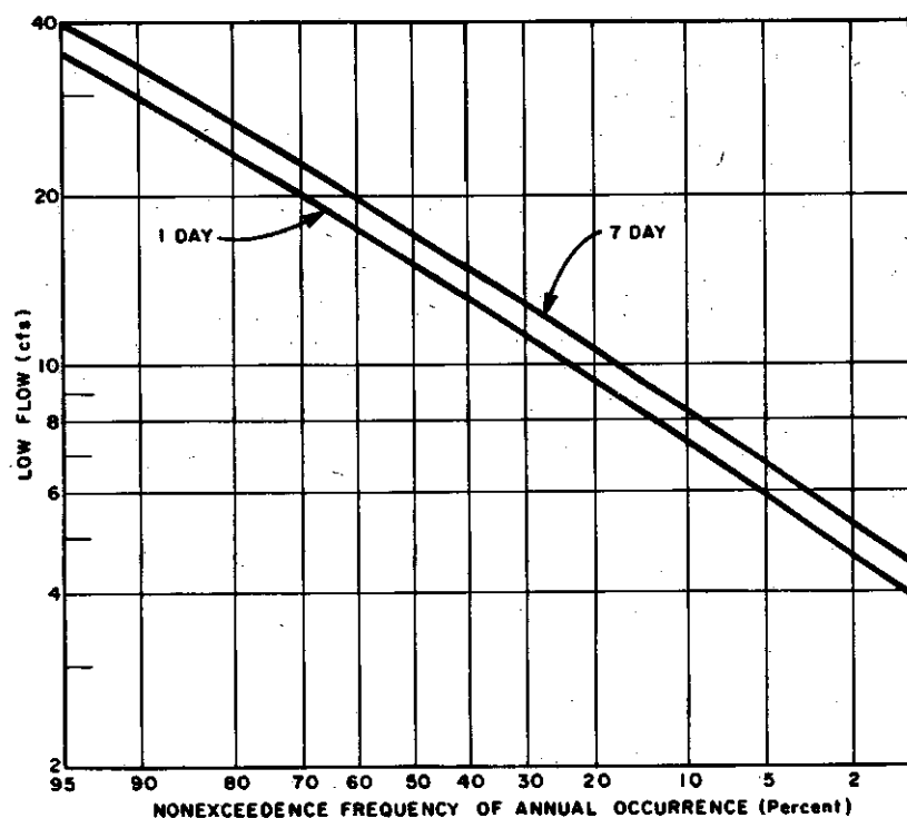
FIGURE 2-36 Low Flow Discharge Frequency Curves, Planning Subarea 1.2, Sturgeon River near Sidnaw, Mich. (171 Sq. Mi. Drainage Area)
