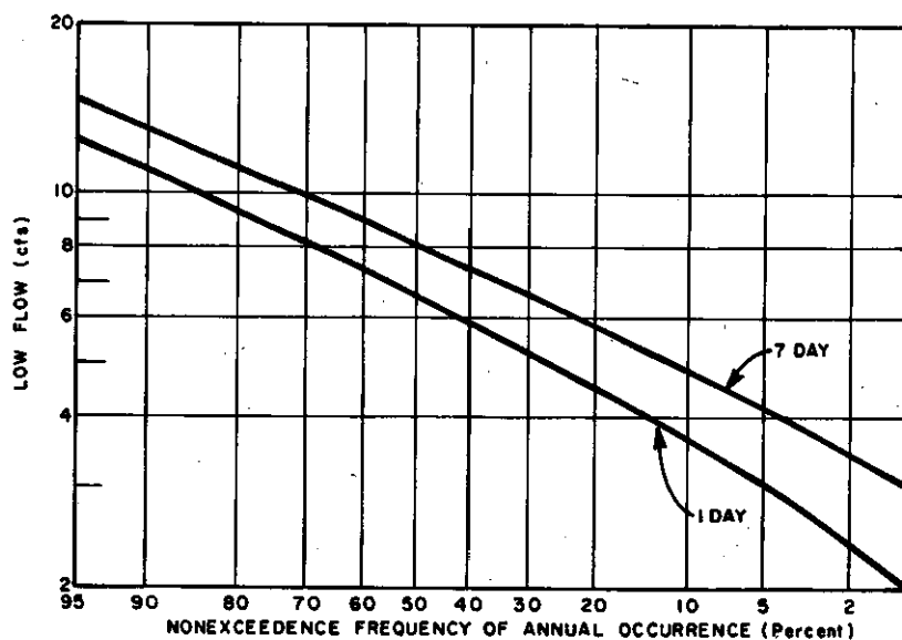
FIGURE 2-38 Low Flow Discharge Frequency Curves, Planning Subarea 2.2, Deep River at Lake George Outlet at Hobart, Ind. (125 Sq. Mi. Drainage Area)
