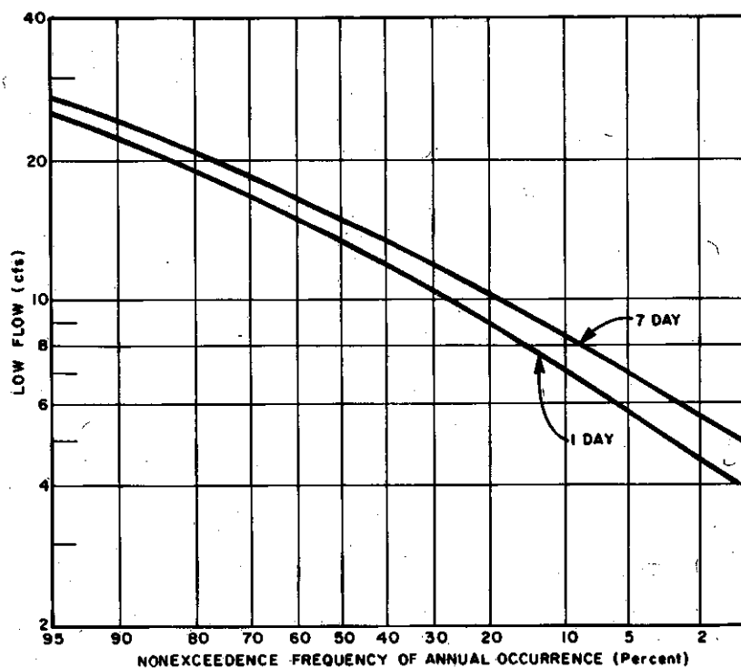
FIGURE 2-35 Low Flow Discharge Frequency Curves, Planning Subarea 1.1, Poplar River at Lutsen, Minn. (114 Sq. Mi. Drainage Area)
