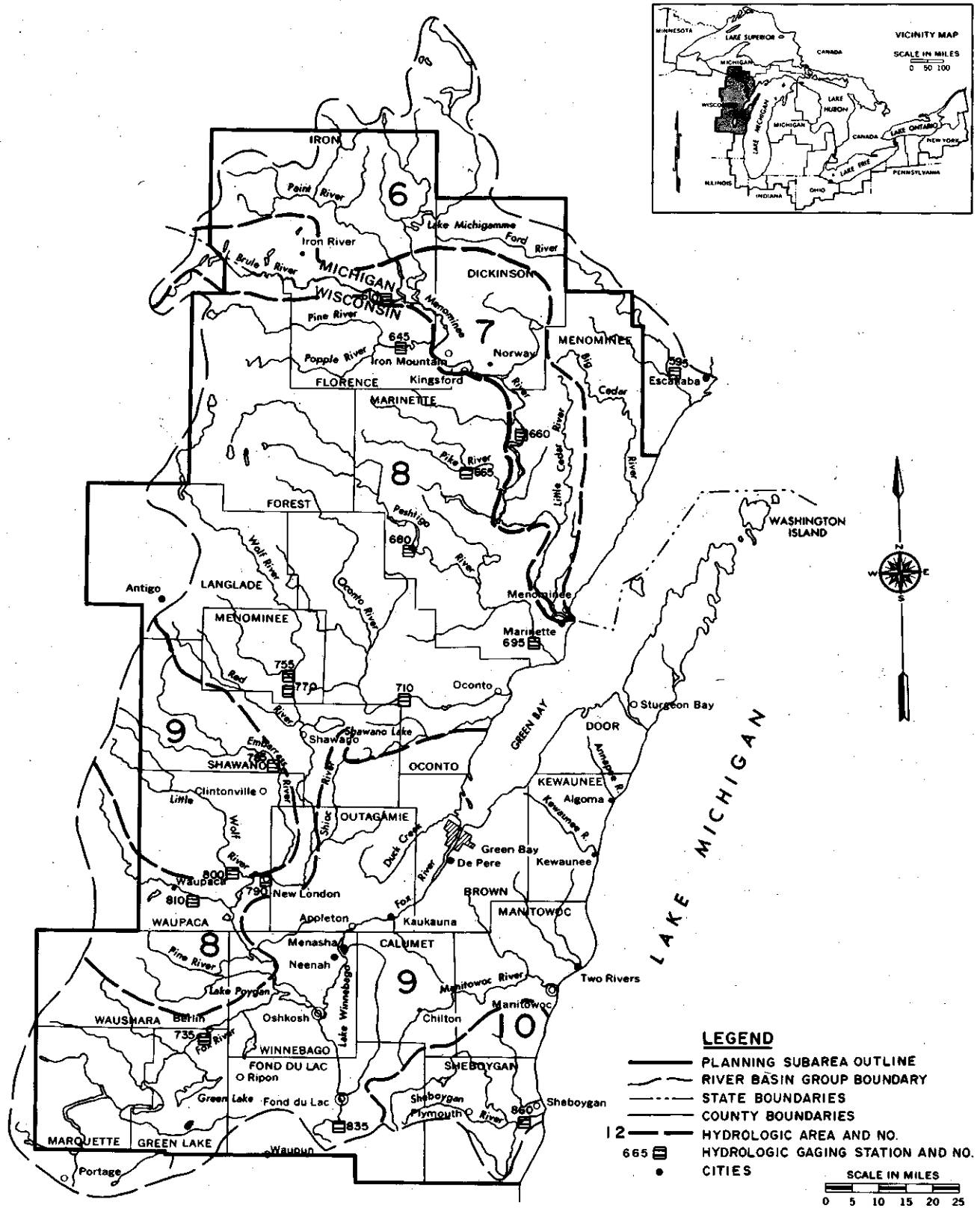
FIGURE 2-3 Hydrologic Gaging Stations, Planning Subarea 2.1
