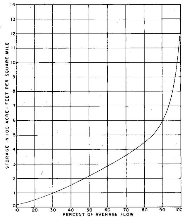
FIGURE 2-76 Generalized Storage Yield Relationship, Planning Subarea 4.4, Cattaraugus Creek at Gowanda, N.Y. (432 Sq. Mi. Drainage Area)
