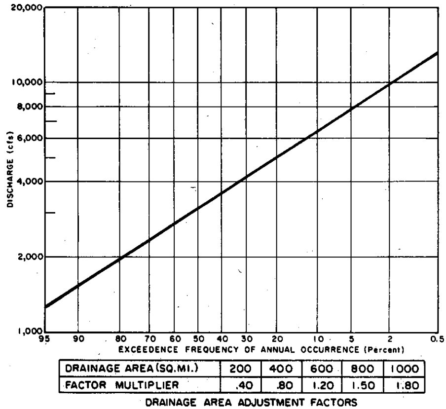
FIGURE 2-22 Peak Discharge Frequency Curve, Planning Sub-area 2.1, Little Wolf River at Royalton, Wis. (514 Sq. Mi. Drainage Area)
