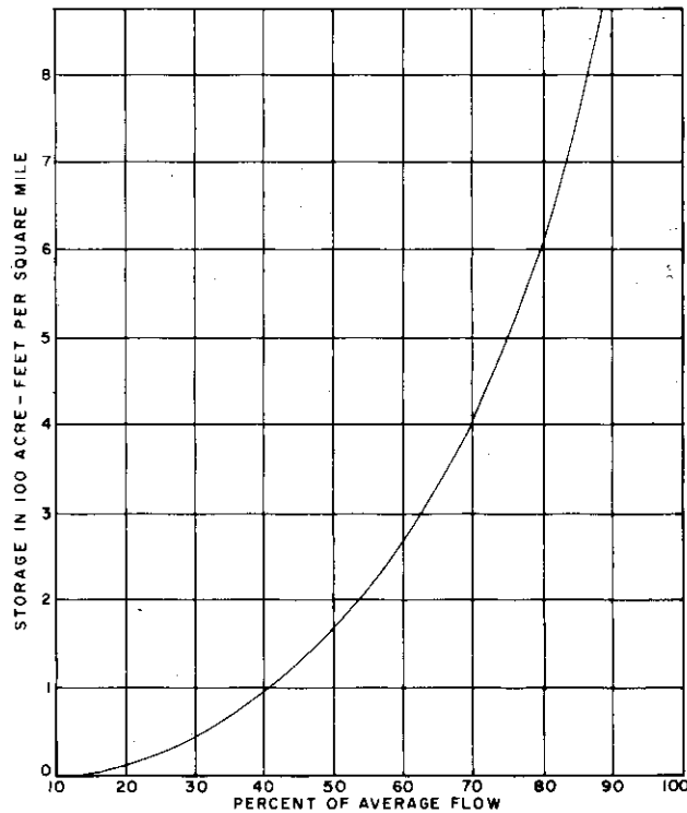
FIGURE 2-69 Generalized Storage Yield Relationship, Planning Subarea 2.3, Grand River at Lansing, Mich. (1,230 Sq. Mi. Drainage Area)
