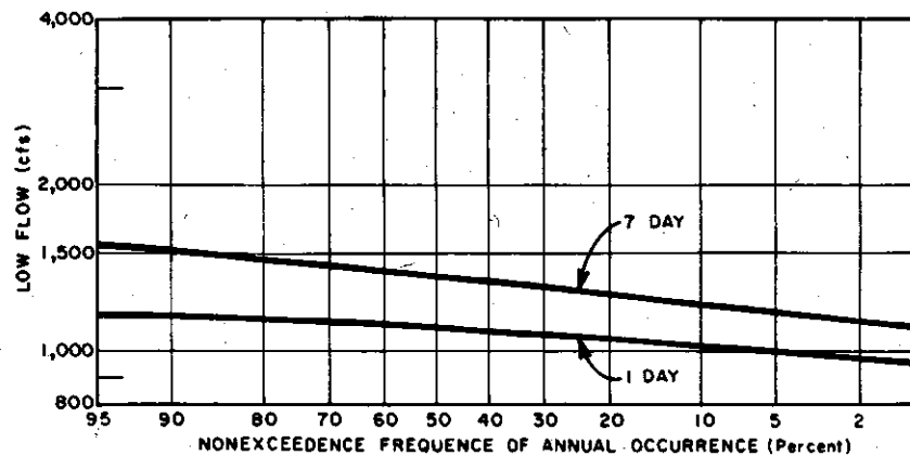
FIGURE 2-40 Low Flow Discharge Frequency Curves, Planning Subarea 2.4, Manistee River Near Manistee, Mich. (1,780 Sq. Mi. Drainage Area)
