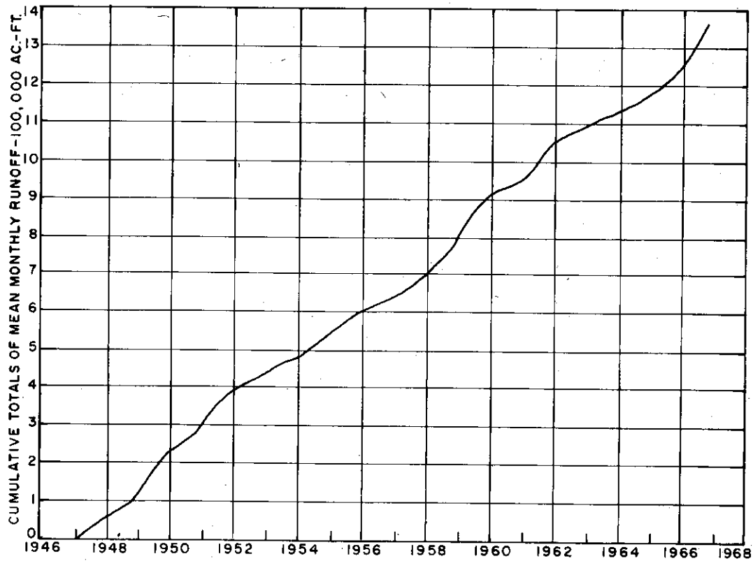
FIGURE 2-52 Mass Curve of Runoff, Planning Subarea 2.1, Pine River Powerplant, Wis.
