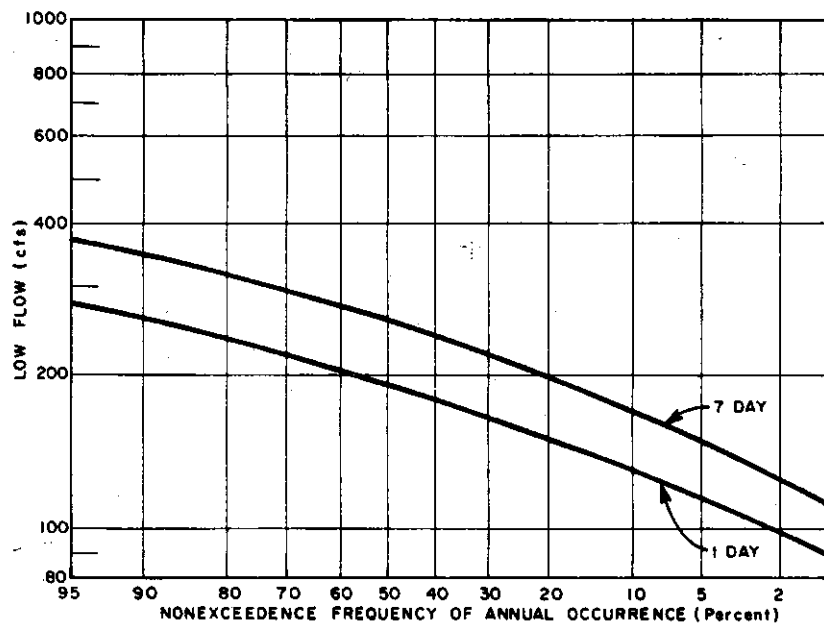
FIGURE 2-42 Low Flow Discharge Frequency Curves, Planning Subarea 3.2, Tittabawassee River at Midland, Mich. (2,400 Sq. Mi. Drainage Area)
