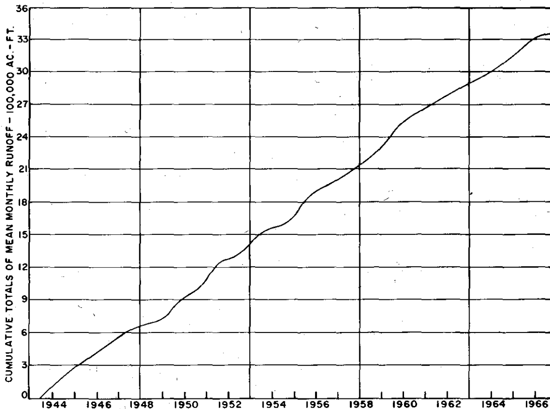
FIGURE 2-51 Mass Curve of Runoff, Planning Subarea 1.2, Sturgeon River Near Sidnaw, Mich.
