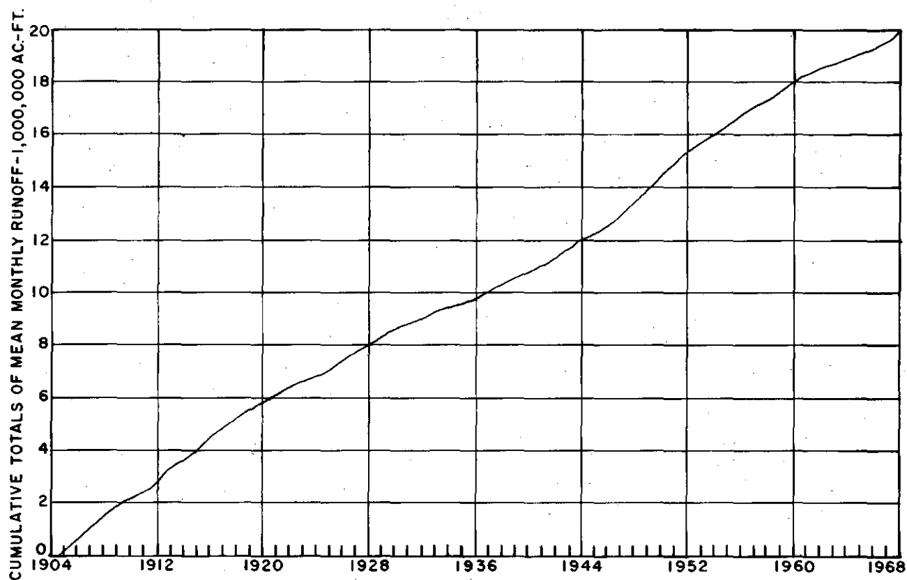
FIGURE 2-58 Mass Curve of Runoff, Planning Subarea 4.1, Huron River at Ann Arbor, Mich.
