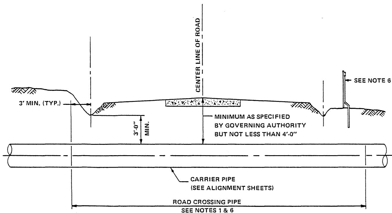
FIGURE 6 ROAD CROSSINGS WITHOUT CASING
