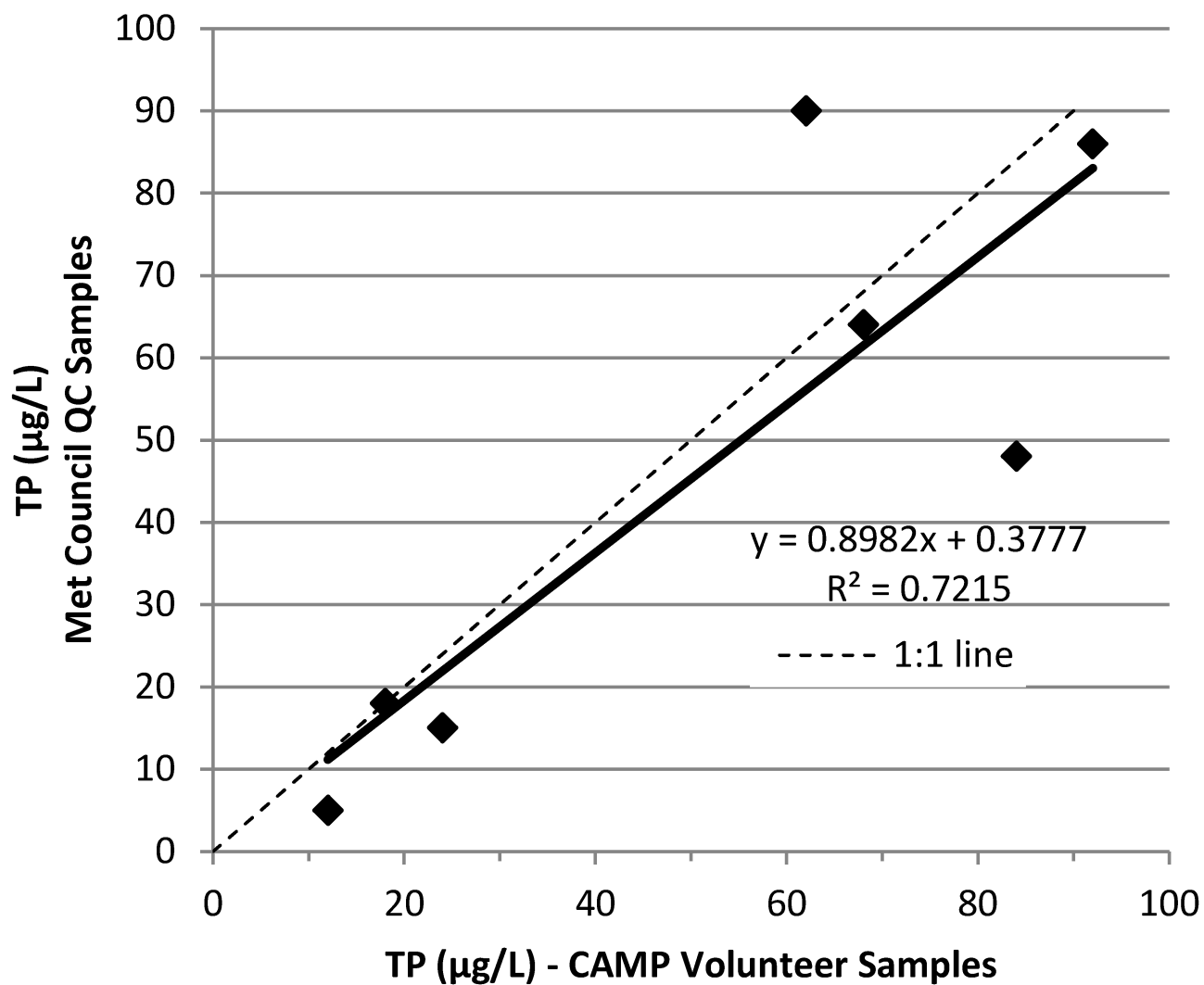
Figure 3. Total Phosphorus Quality Control Data
