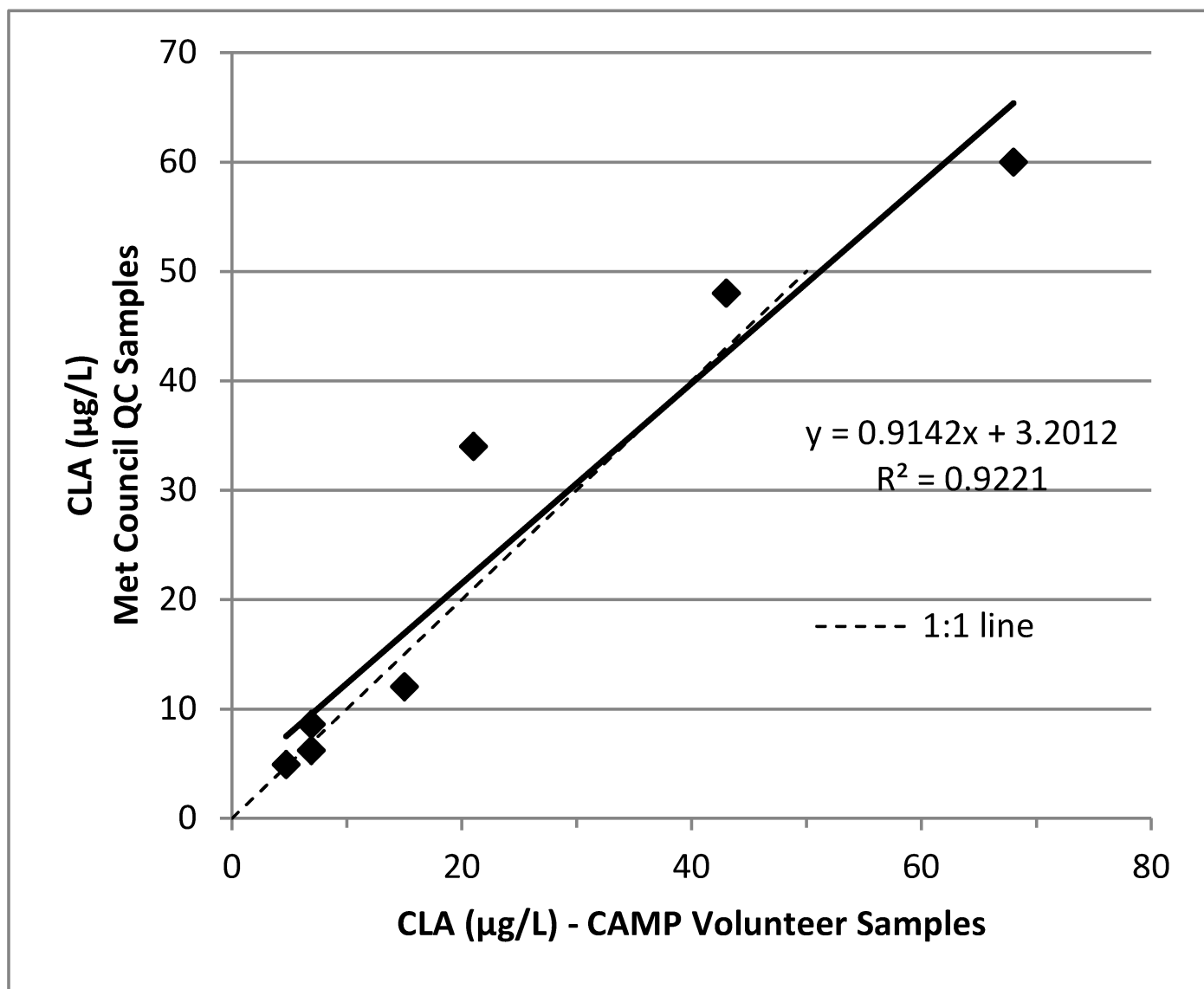
Figure 4. Chlorophyll-a Quality Control Data
