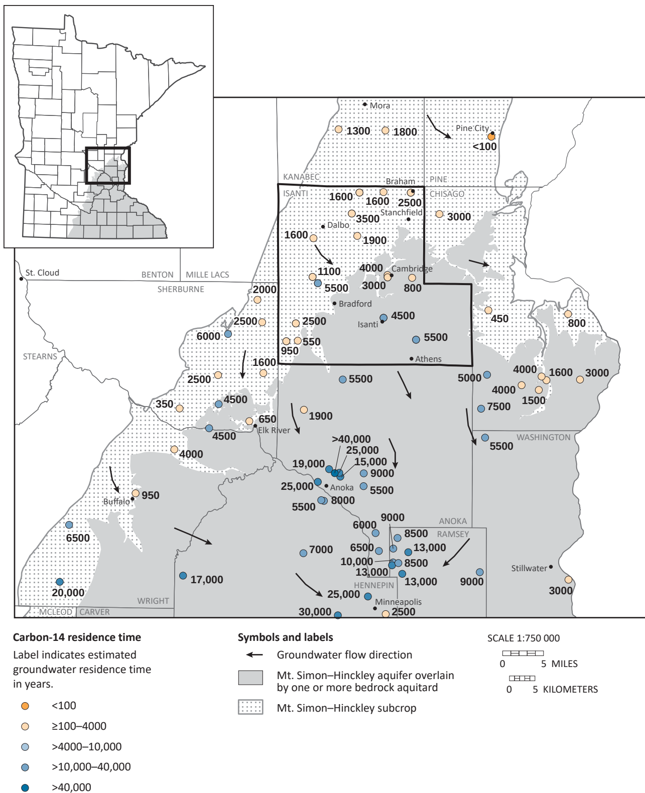
Figure 30. Carbon-14 residence time and groundwater flow of the Mt. Simon–Hinckley subcrop
