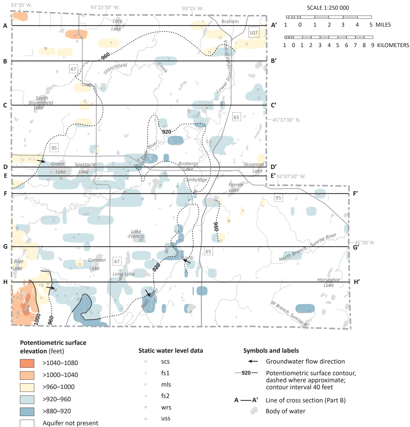
Figure 8. Potentiometric surface of the lower Quaternary buried sand aquifers
