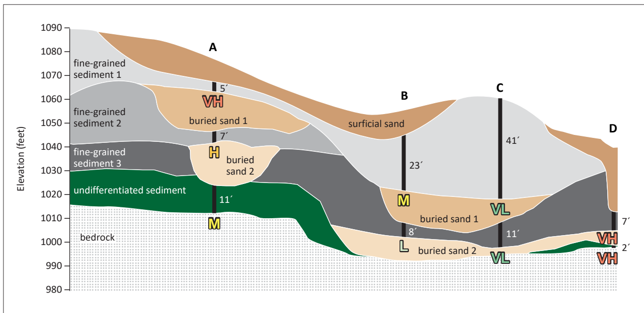
Figure 19. Cross section illustration of the pollution sensitivity model
