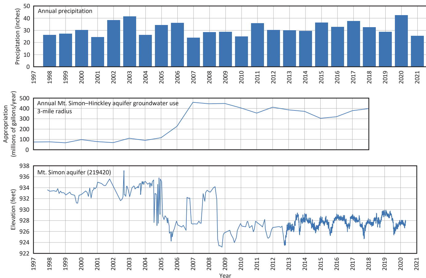
Figure 34. Hydrograph of precipitation, groundwater use, and groundwater elevation of a well at location 3 near Cambridge
