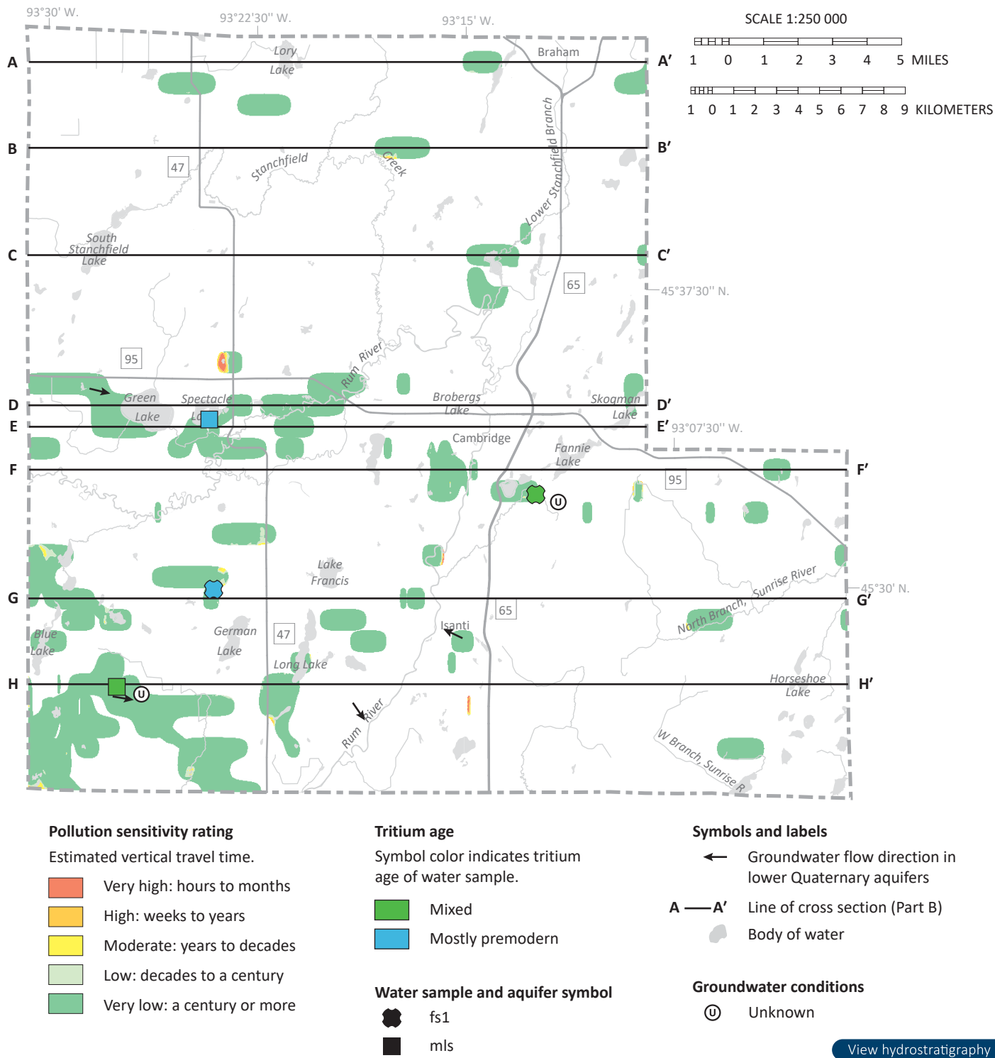
Figure 26. Pollution sensitivity of the lower Quaternary aquifers
