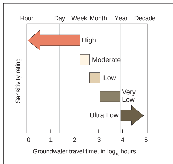
Figure 16. Pollution sensitivity of near-surface materials: travel time and ratings
