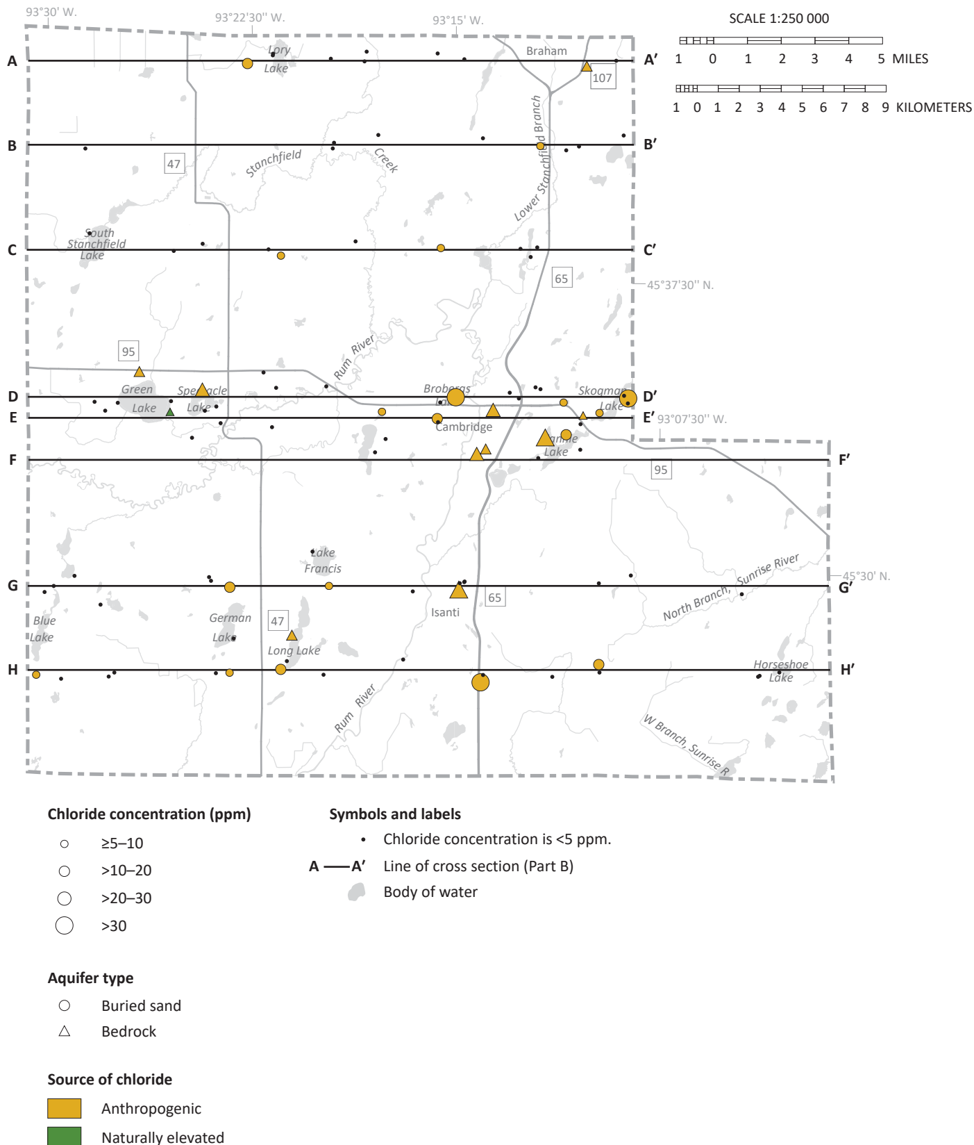
Figure 13. Chloride concentrations from groundwater samples
