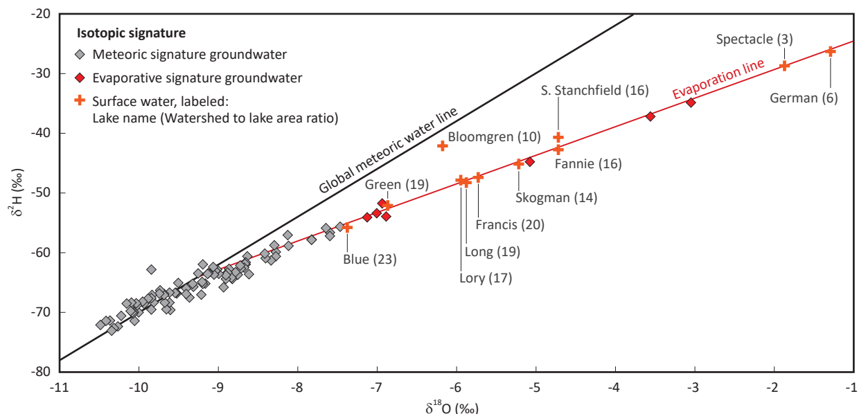
Figure 11. Stable isotope values from water samples
