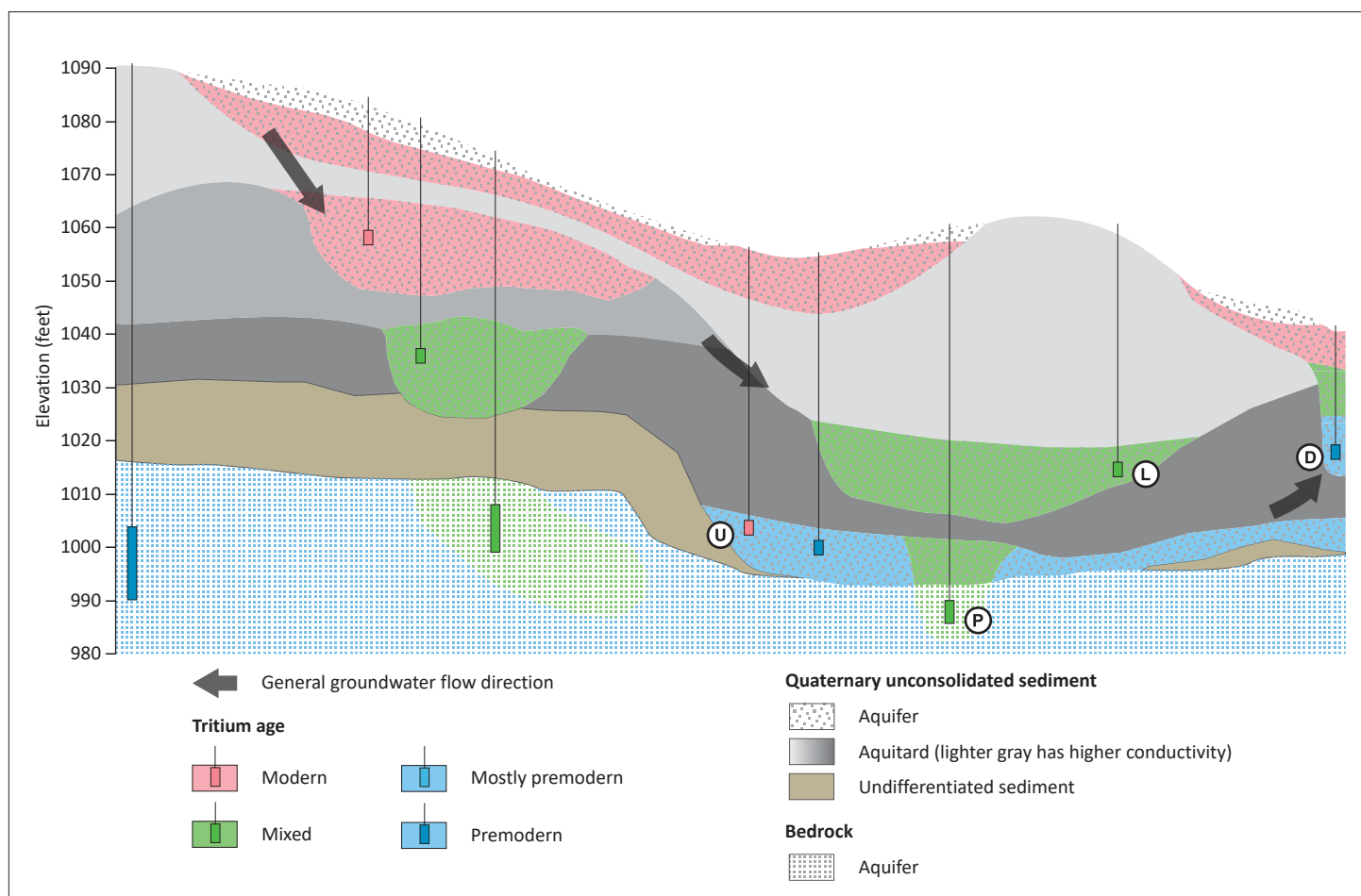
Figure 20. Cross section illustration of groundwater conditions
