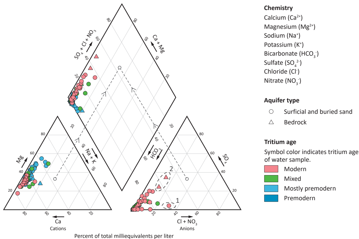
Figure 15. Piper diagram of groundwater sampled by DNR staff
