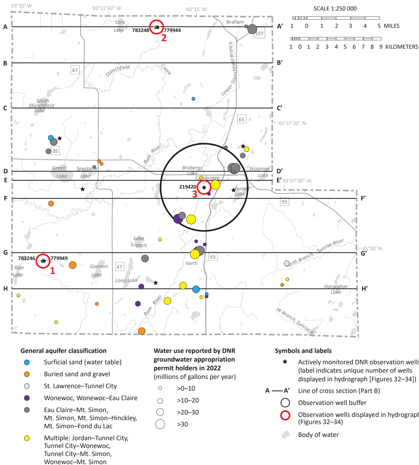
Figure 31. Groundwater appropriation permits shown by aquifer group and observation well locations
