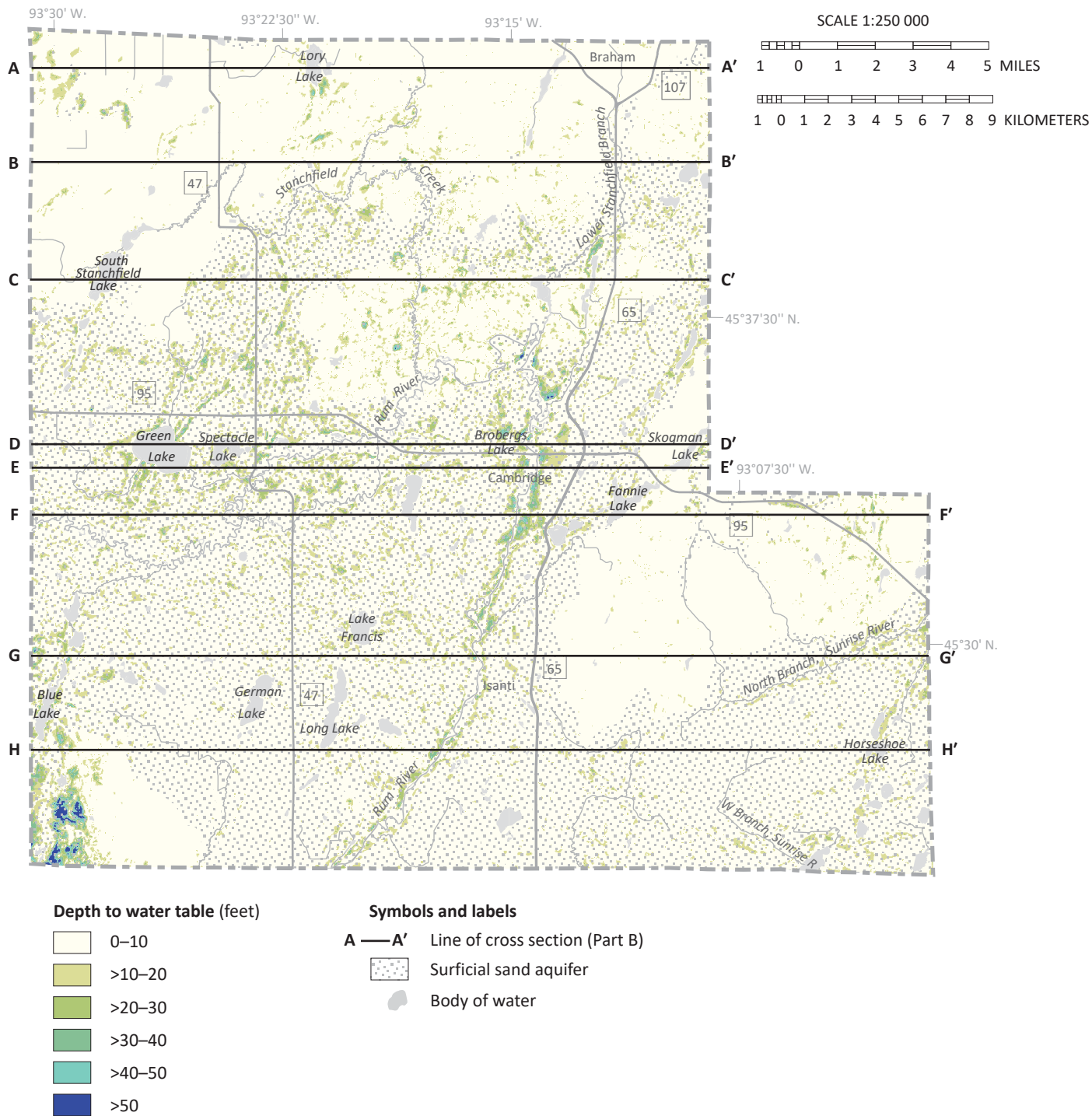
Figure 6. Depth to water table
