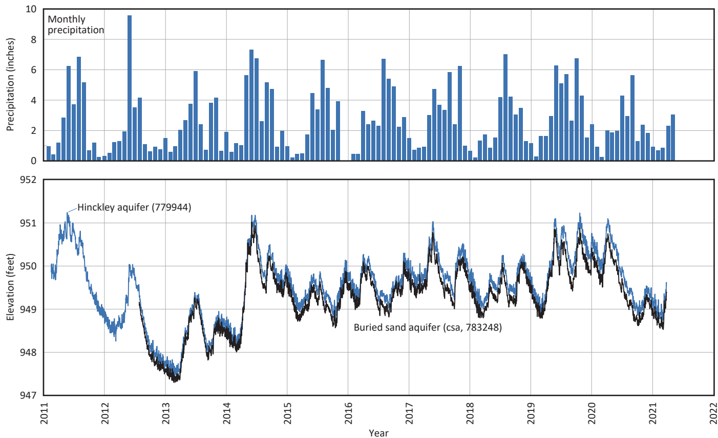
Figure 33. Hydrograph of precipitation and groundwater elevation of a well nest at location 2 in northern Isanti County
