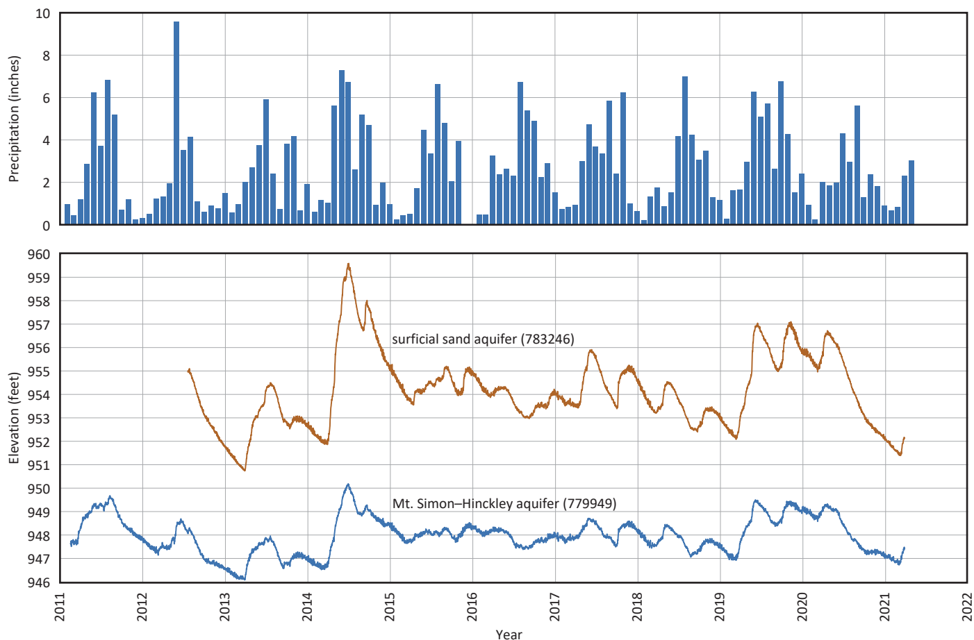
Figure 32. Hydrograph of precipitation and groundwater elevation of a well nest at location 1 in southwest Isanti County
