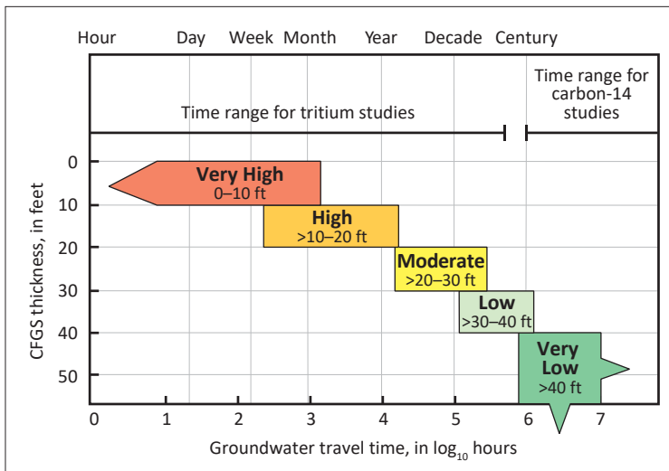
Figure 18. Pollution sensitivity rating for the buried sand aquifers and the bedrock surface
