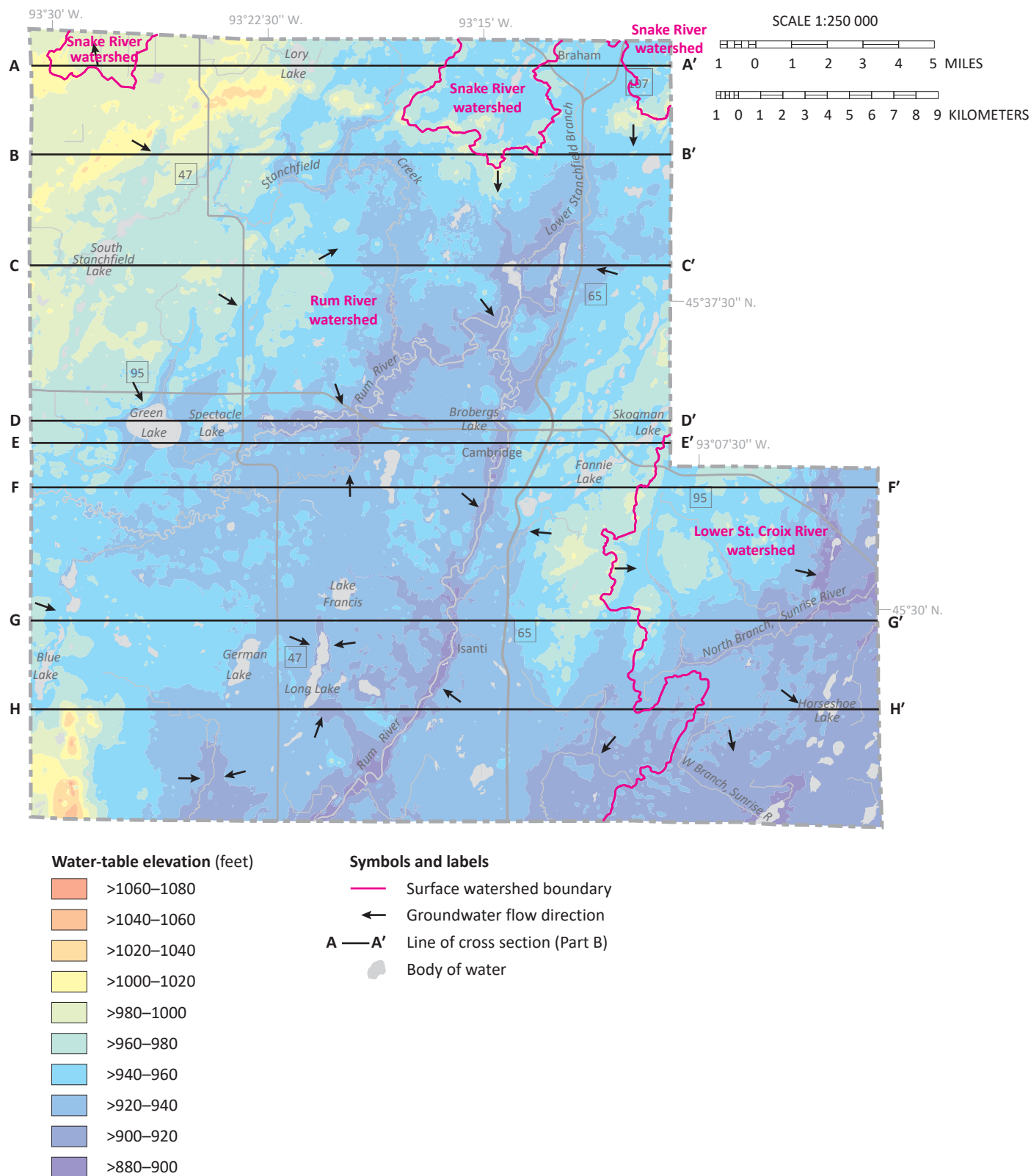
Figure 5. Water-table elevation and groundwater flow directions
