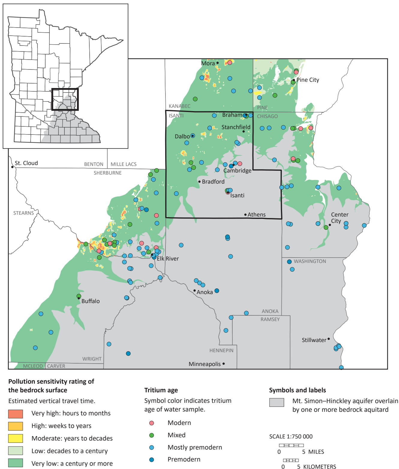
Figure 29. Pollution sensitivity and recharge of the Mt. Simon-Hinckley subcrop
