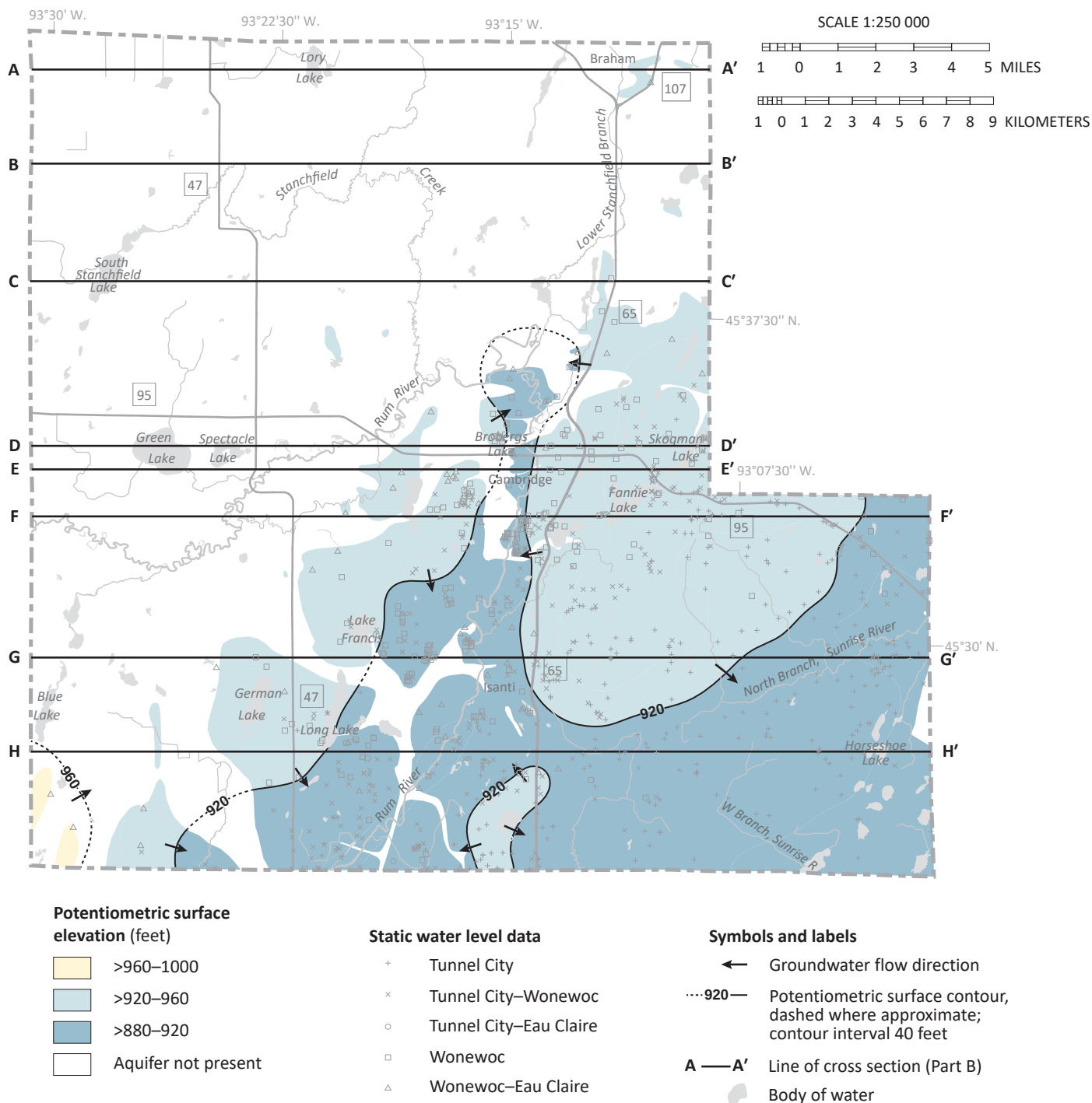
Figure 9. Potentiometric surface of the Upper Tunnel City and Wonewoc aquifers
