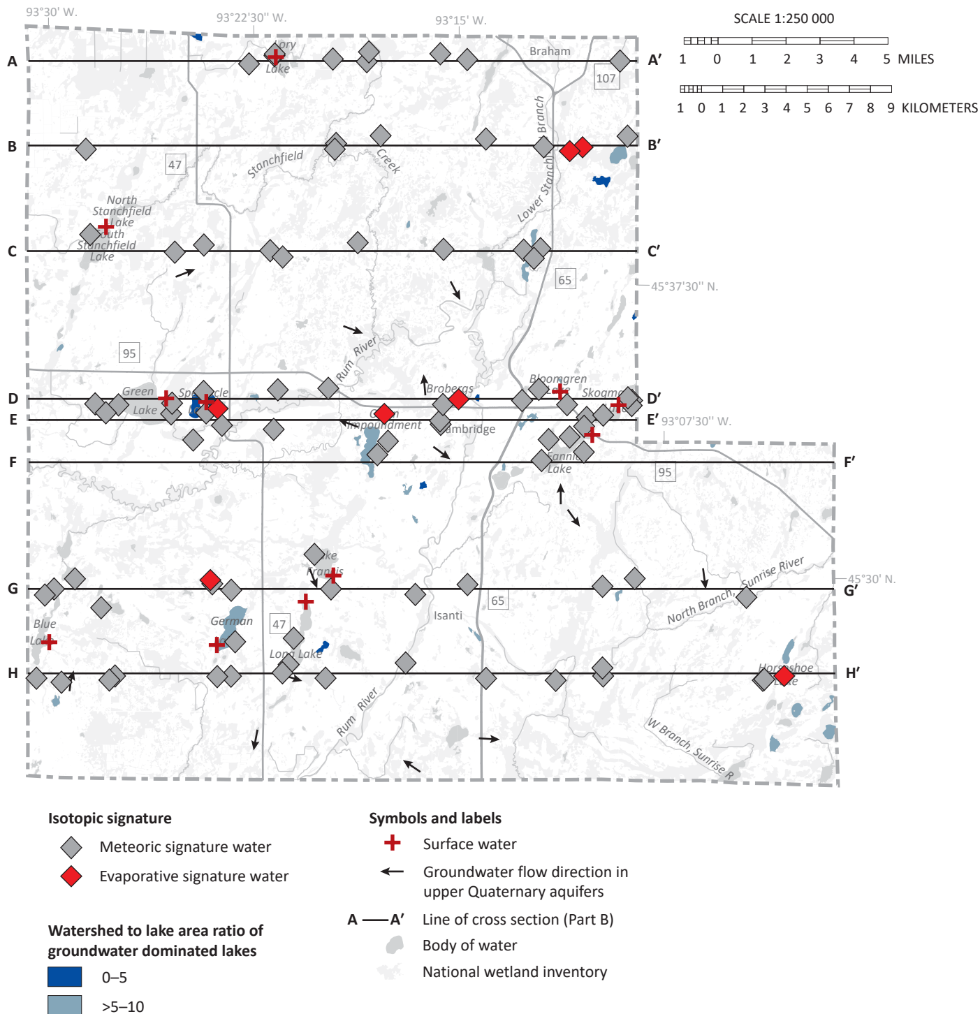
Figure 12. Stable isotope characteristics of groundwater samples
