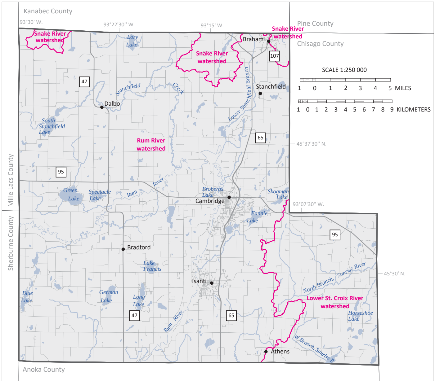
Figure 1. Isanti County, Minnesota
