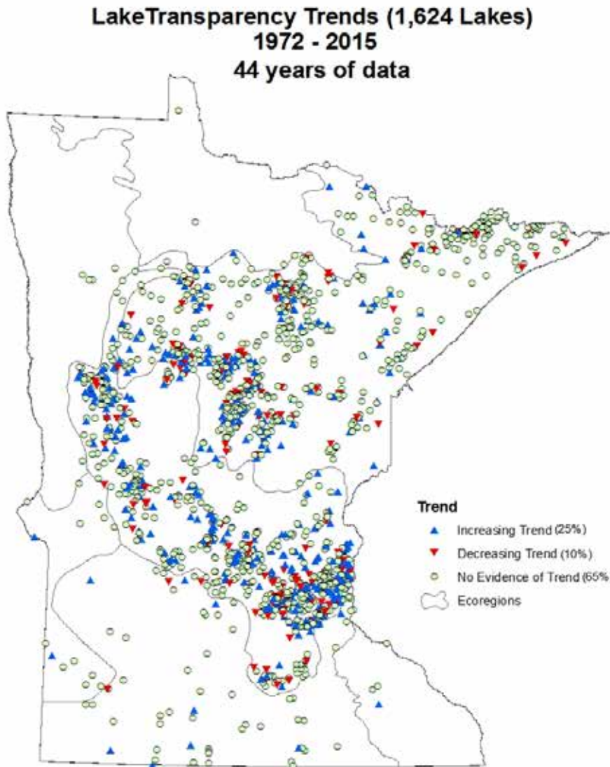
Figure 11. Lake Transparency Trends for 1972-2015
