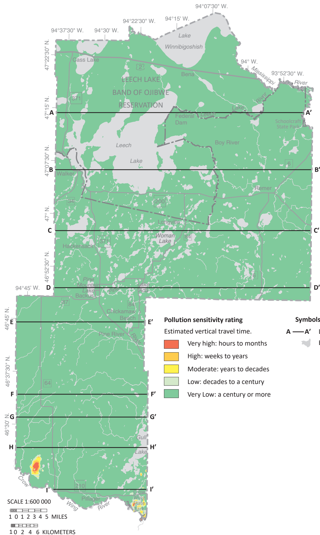
Figure 36. Pollution sensitivity of the bedrock surface. Very low sensitivity is the most common value. Some areas of higher sensitivity are mapped in the south. Less than 1 percent of county wells with known construction information are completed in these aquifers.
