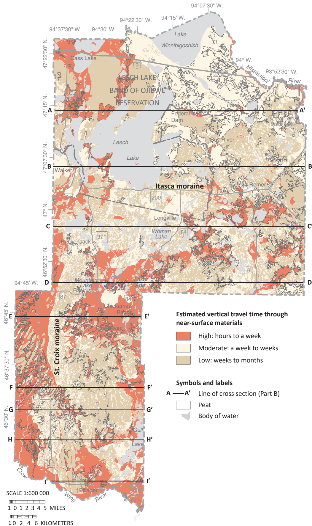
Figure 20. Pollution sensitivity of near-surface materials
