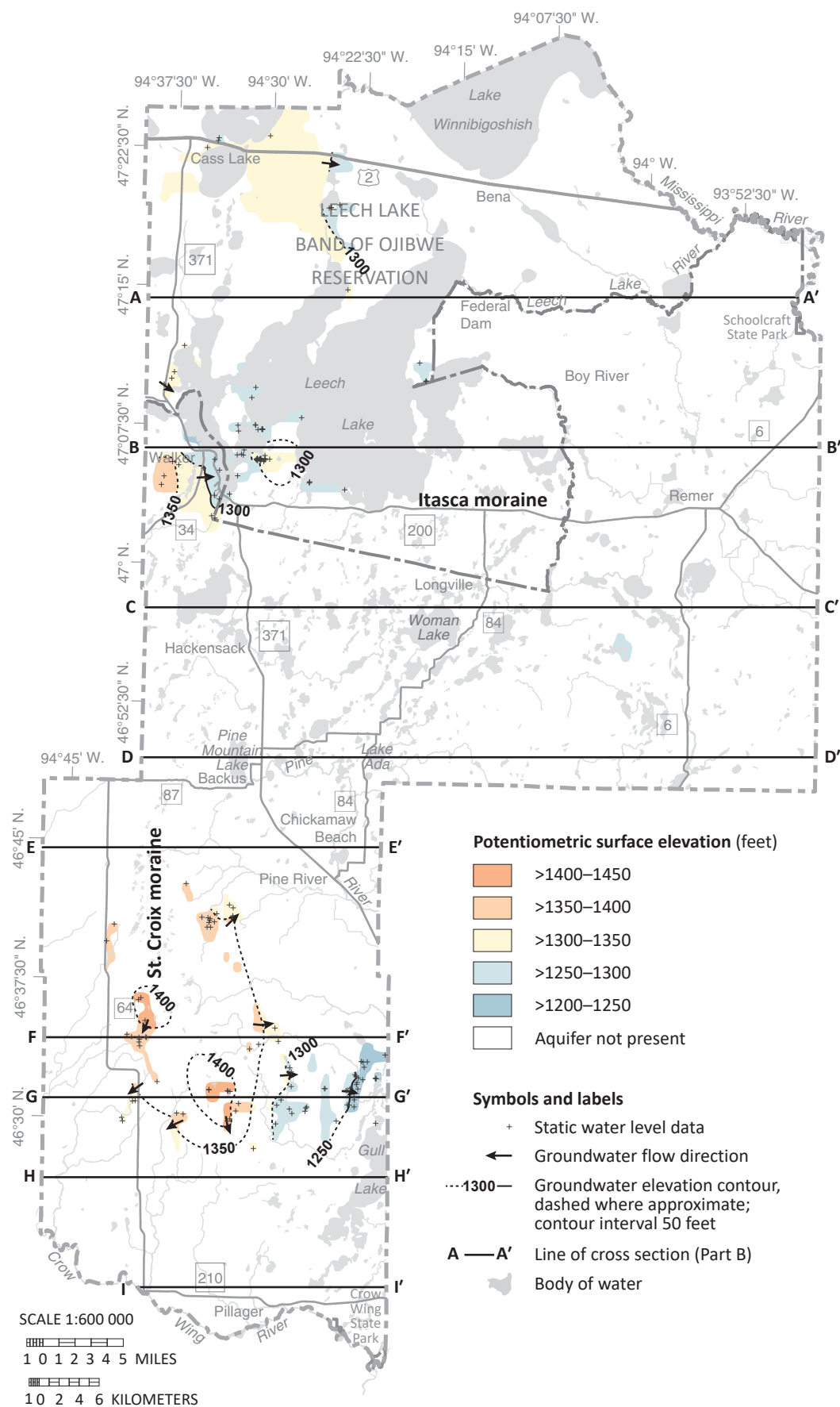
Figure 10. Potentiometric surface of the hsa4 and iss6 aquifers
