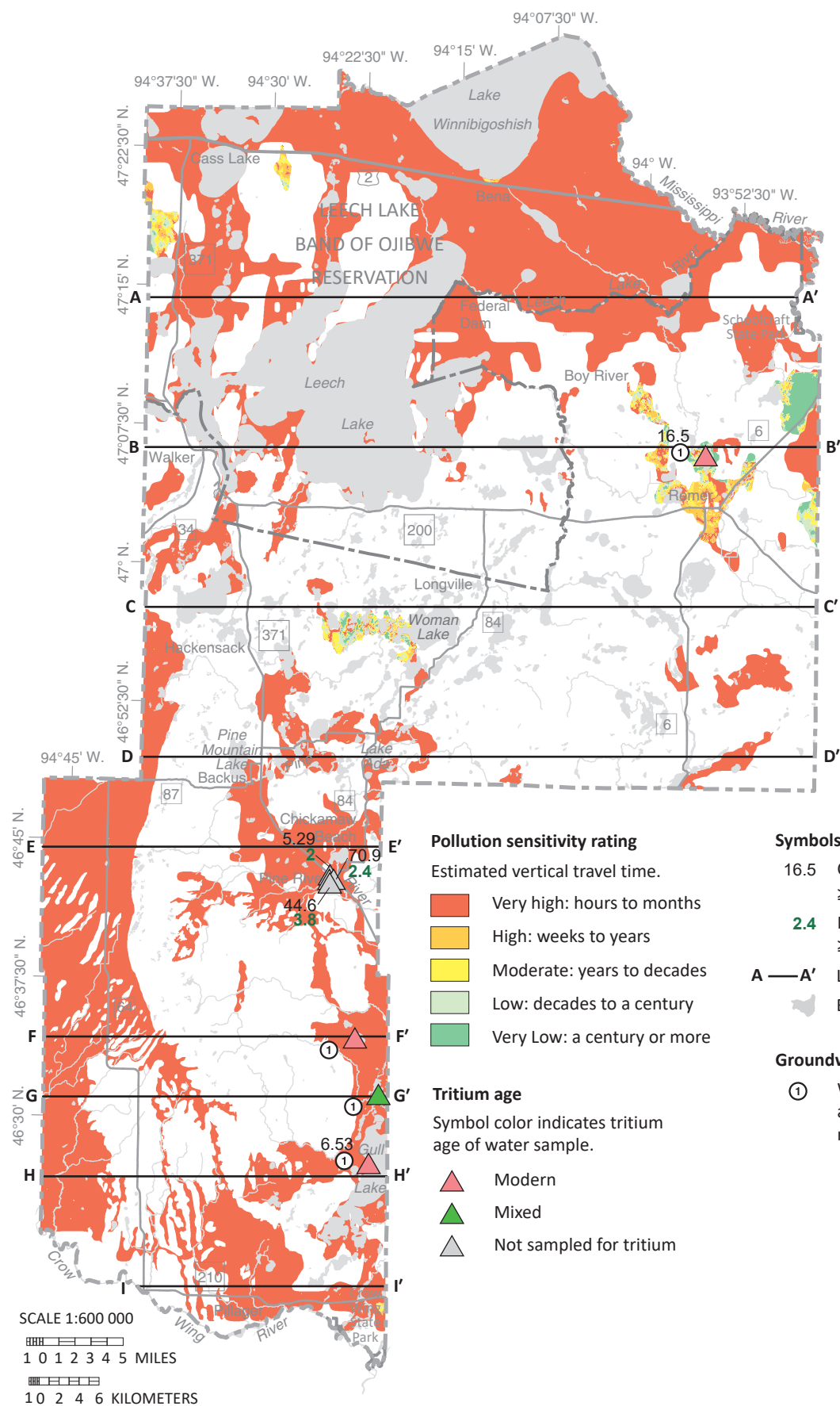
Figure 24. Pollution sensitivity of the bds, hsi1, and iss1 aquifers and groundwater flow directions Sensitivity is mostly very high, because of surface exposures over most of the county. Approximately 5 percent of county wells with known construction information are completed in the hsi1 and iss1 aquifers.
