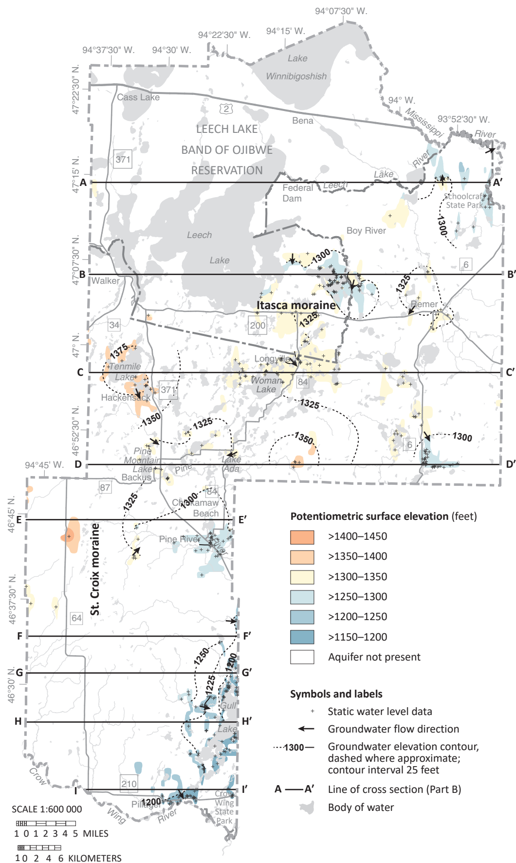
Figure 14. Potentiometric surface of the mls3 and sfs3 aquifers Much of the mapped portions of these aquifers is in the central portion of the county where groundwater flow directions tend to be complex. Tenmile Lake in the west near Hackensack appears to be near the apex of flow which radiates easterly and south toward the Pine River.
