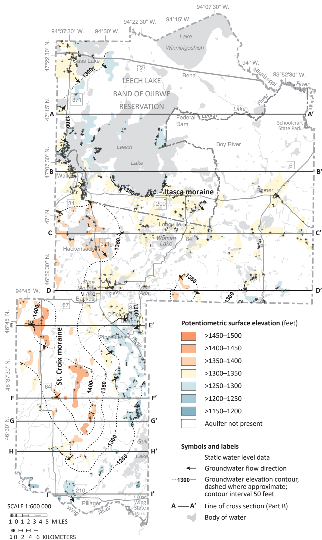
Figure 8. Potentiometric surface of the hsa2 and iss4 aquifers The dominant flow directions are from the topographic highs of the two moraines radially toward major surface-water features. In the north flow is from the western portion of the Itasca moraine (Hackensack area) radially toward Leech and Woman lakes. In the south flow is from the crest of the St. Croix moraine radially toward Pine River, Crow Wing River, and Gull Lake.
