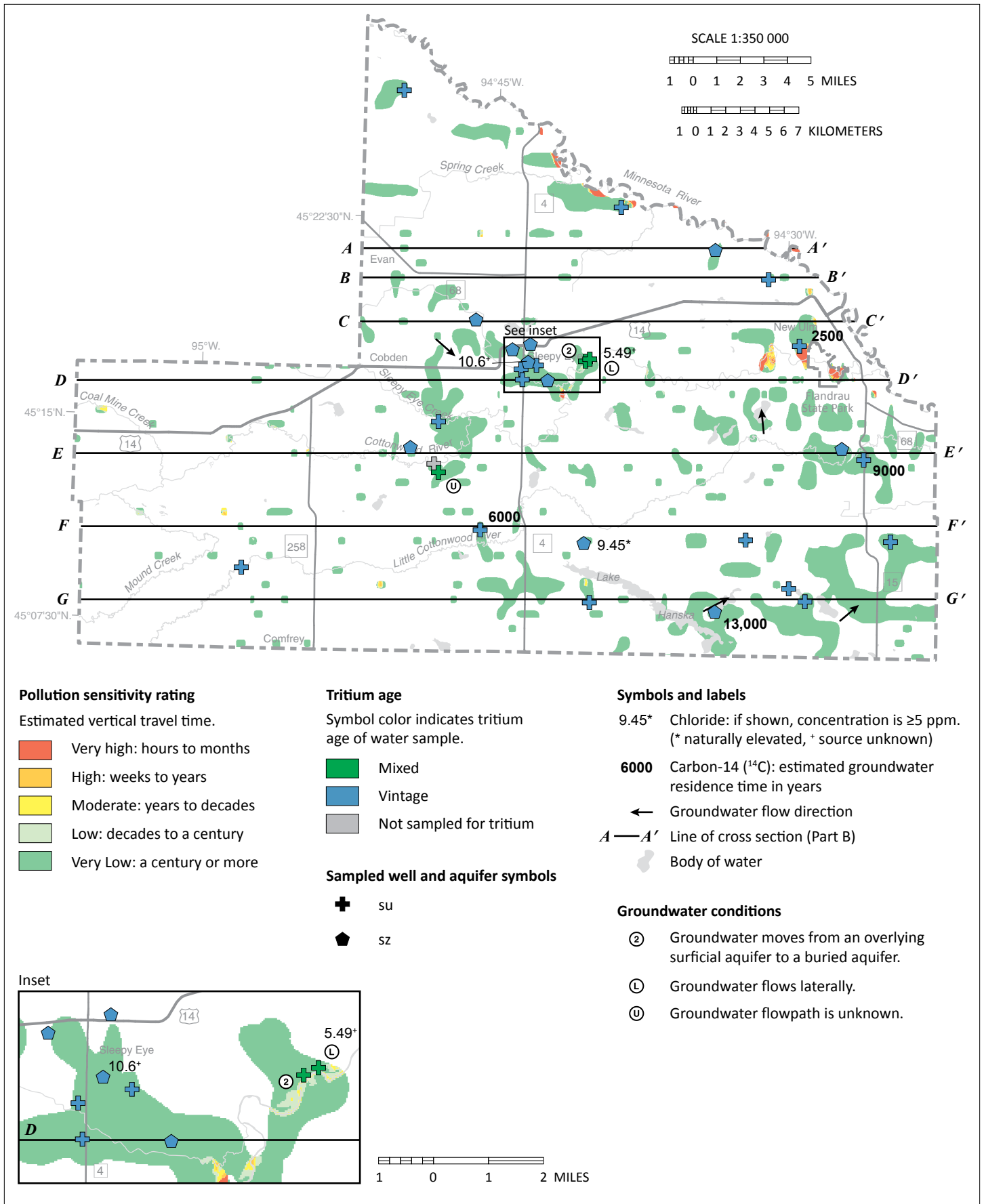
Figure 29. Pollution sensitivity of the su and sz (undifferentiated buried sand) aquifers and groundwater flow directions These undifferentiated aquifers were mapped as sand bodies of various sizes across the county. The pollution sensitivity is mostly very low with some higher sensitivity ratings in the Minnesota and Cottonwood river valleys where these aquifers are relatively shallow.
