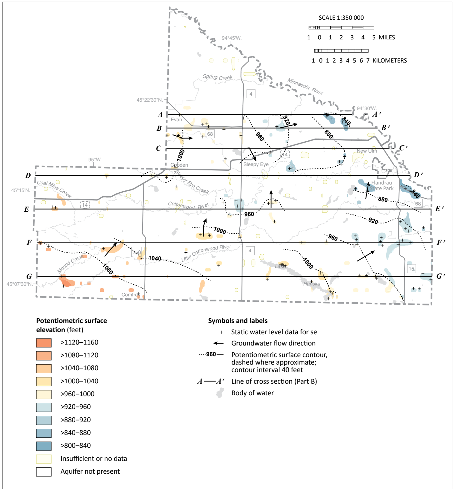
Figure 11. Potentiometric surface of the se aquifer The dominant groundwater flow directions are toward the Minnesota and Cottonwood rivers.
