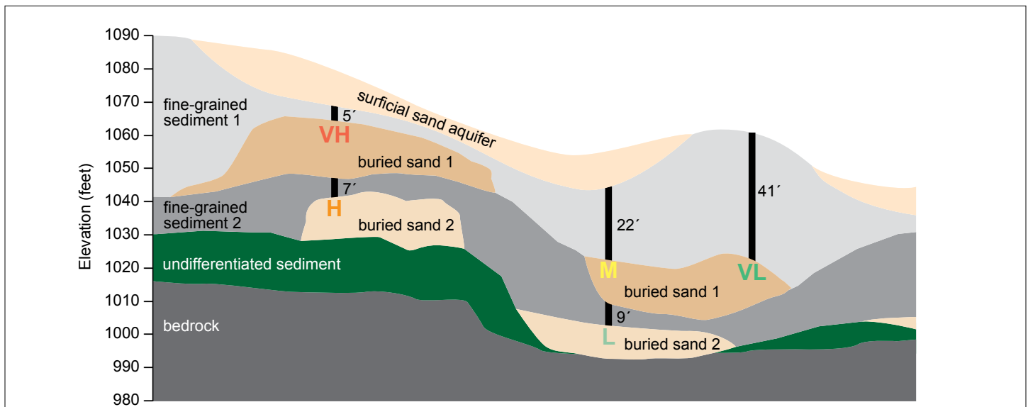
Figure 22. Cross section showing examples of pollution sensitivity ratings
