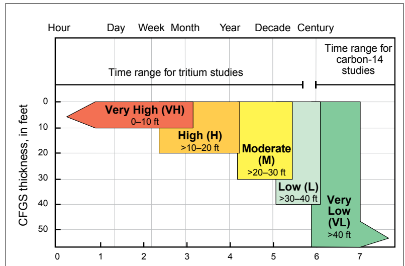
Figure 21. Geologic sensitivity rating for the buried sand aquifers and the bedrock surface
