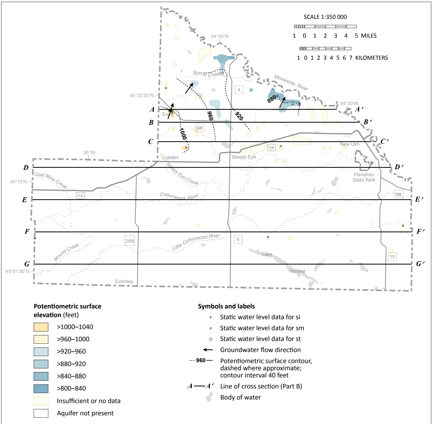
Figure 8. Potentiometric surface of the si, sm, and st aquifers Limited data indicate groundwater flow directions toward the Minnesota River.
