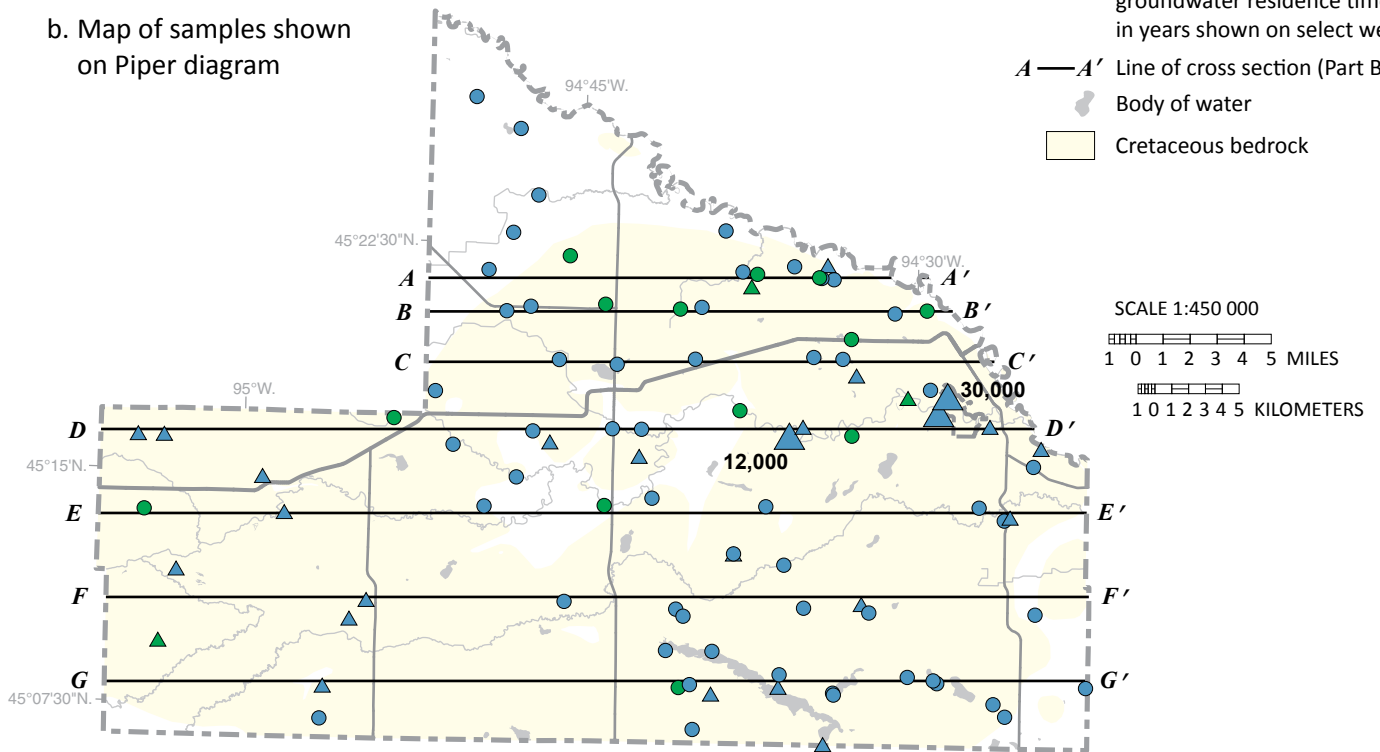
Figure 18. Piper diagram of groundwater samples and tritium age
