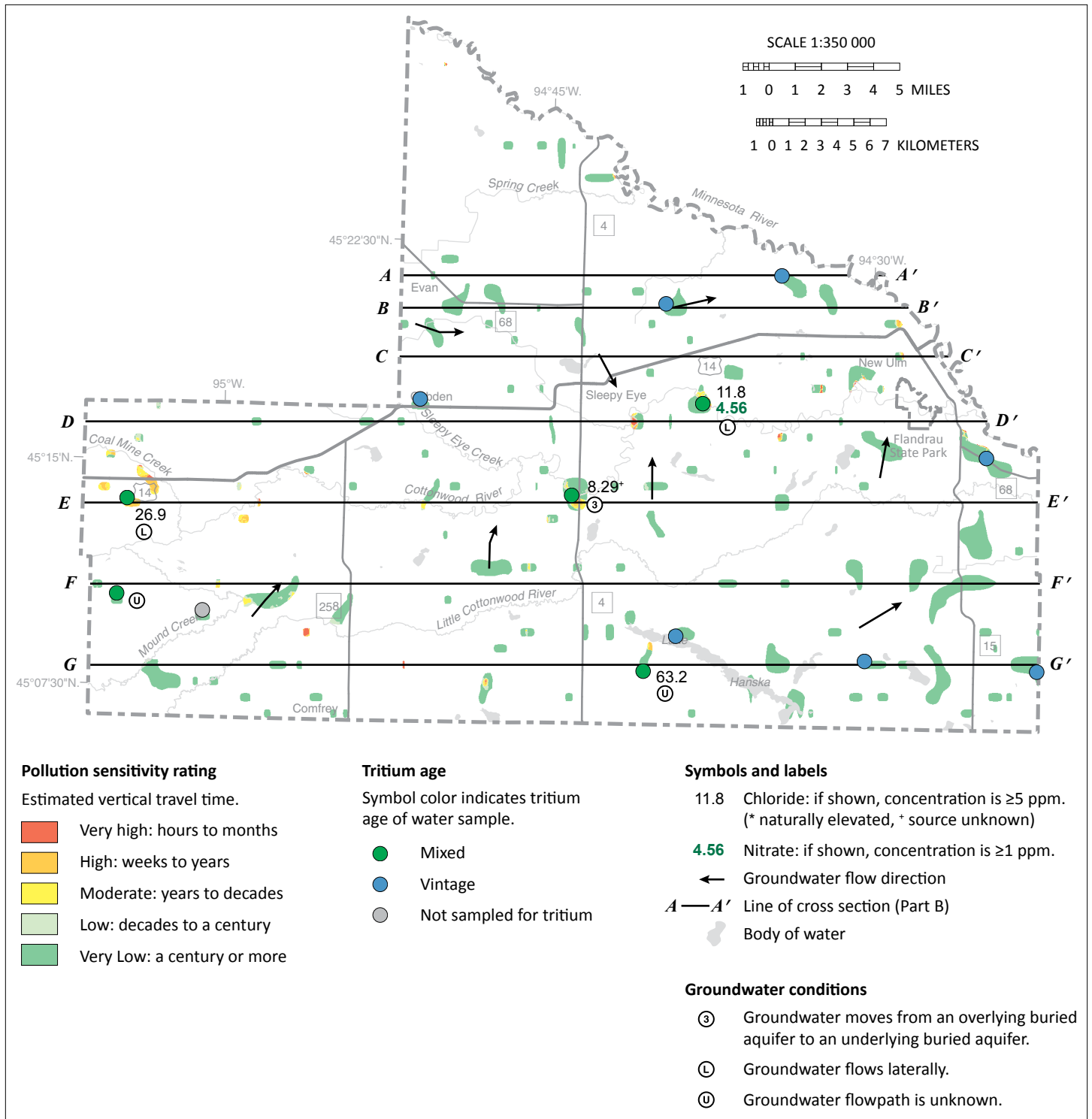
Figure 28. Pollution sensitivity of the se aquifer and groundwater flow directions
