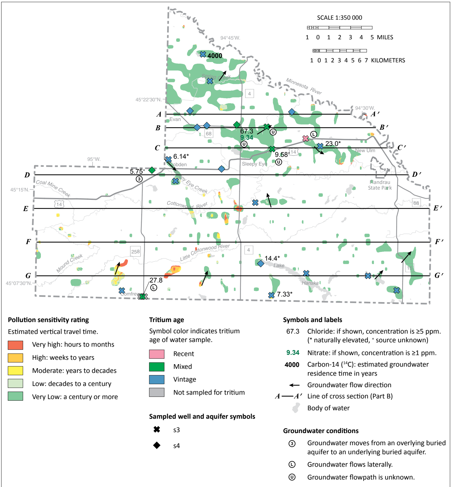
Figure 27. Pollution sensitivity of the s3 and s4 aquifers and groundwater flow directions
