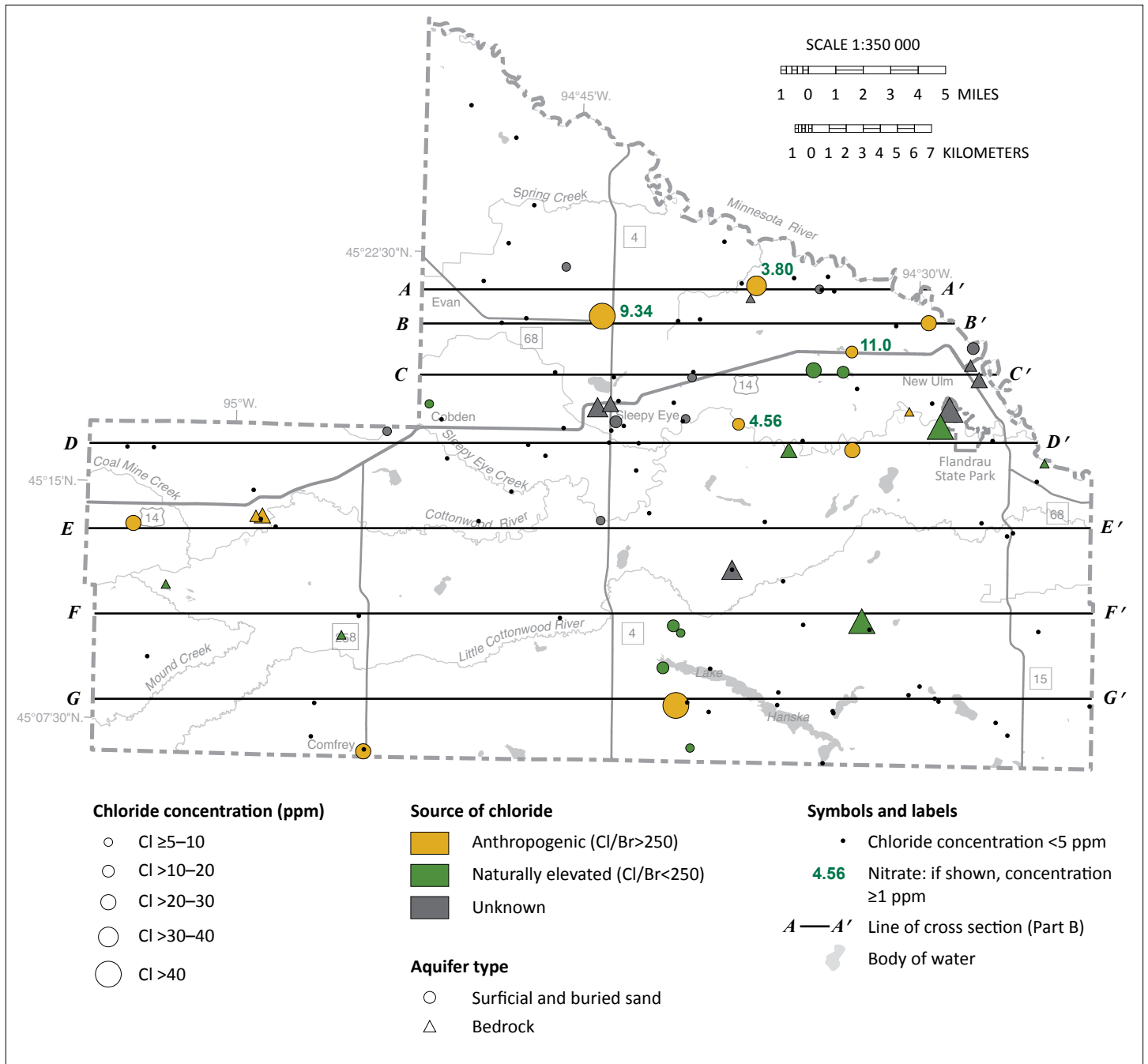
Figure 16. Chloride and elevated nitrate concentrations from groundwater samples
