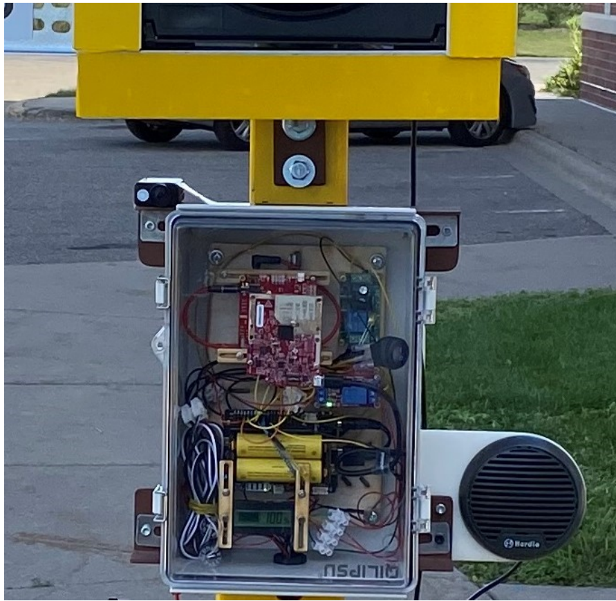
Figure 2.5 Photograph of electronics box and speaker on the smart work zone traffic signal.
