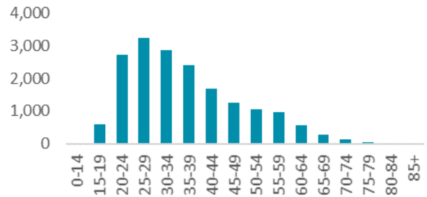
Figure 2.03: Impaired Driving Incidents (“DWIs”) by Age Group
