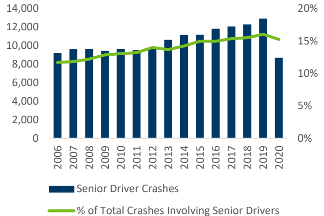
Figure 11.01: Senior Driver Crash Trends
