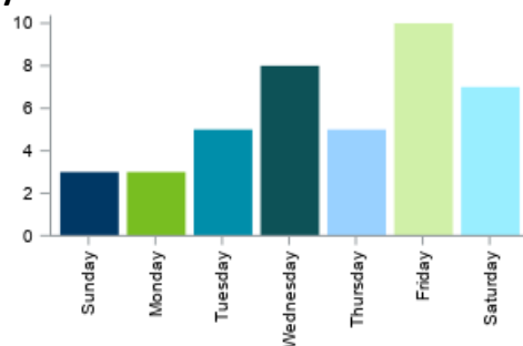
Figure 9.03: Motor Vehicle/Train Crashes by Day of Week
