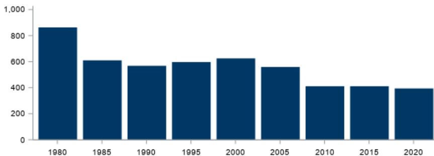
Figure 2: Minnesota Traffic Fatalities
