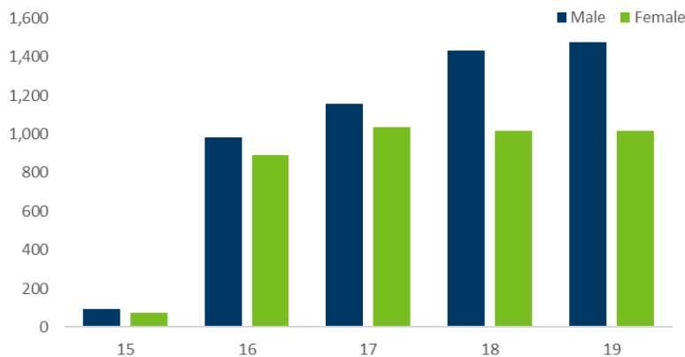
Figure 10.03: Teen Driver Crashes by Age and Gender
