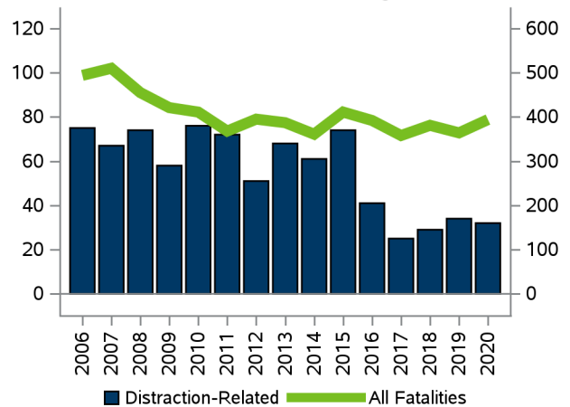
Distraction-Related Fatality Trends
