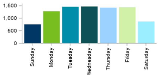
Figure 11.02: Senior Driver Crashes by Day of Week
