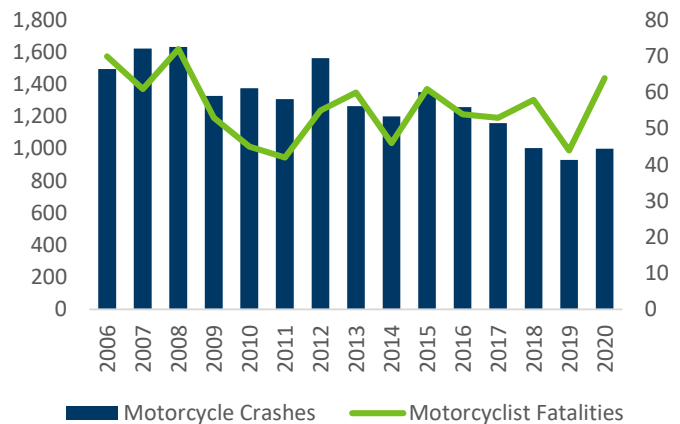
Figure 4.01: Motorcycle Crash Trends
