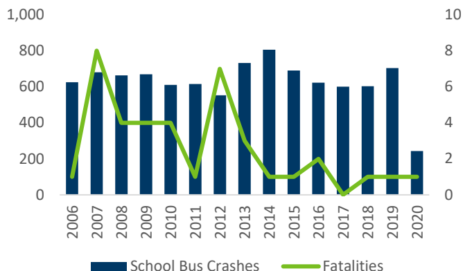
Figure 8.01: School Bus Crash Trends
