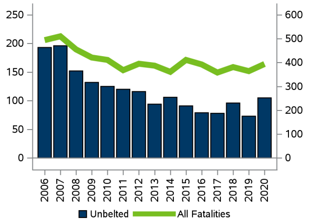
Unbelted Fatality Trends
