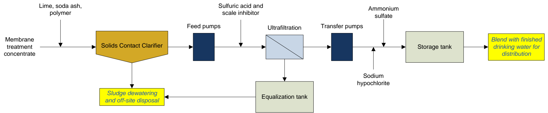
Figure 4-2 Zero liquid discharge concentrate management, City of Palm Coast Water Treatment Plant #2
