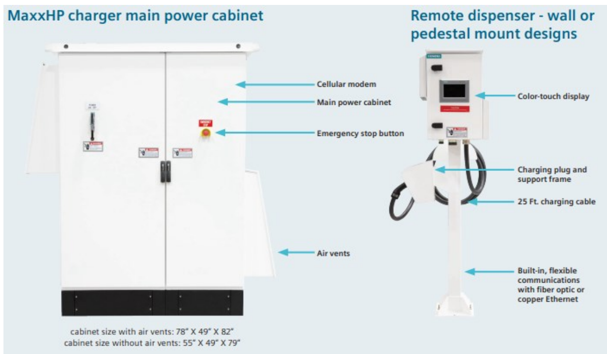
Figure 34: Siemens MaxxHP charger dimensions 89
