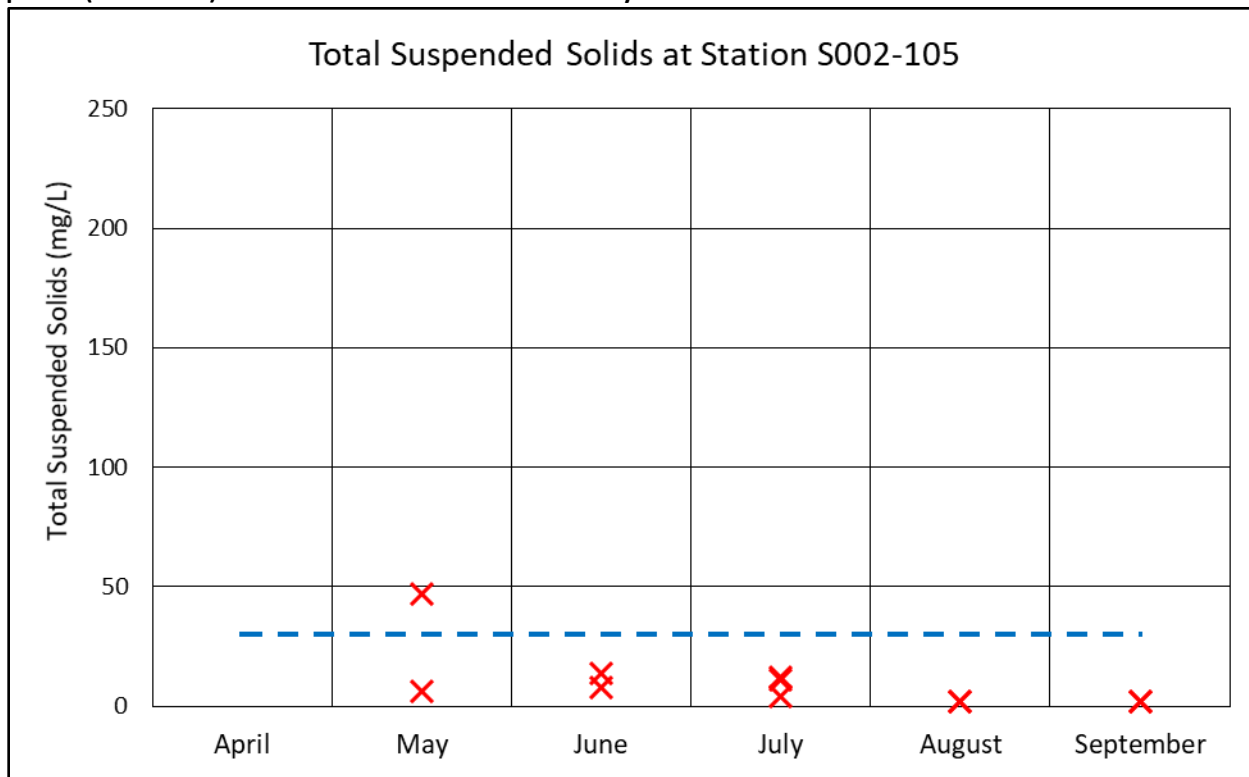
Figure B-1: TSS sampling aggregated by month on Hay Creek at the monitoring station S002-105. The dashed line denotes the stream water quality standard (30 mg/L). Data originates from intensive watershed monitoring period (2015-2016). Data not included in the TMDL analysis.
