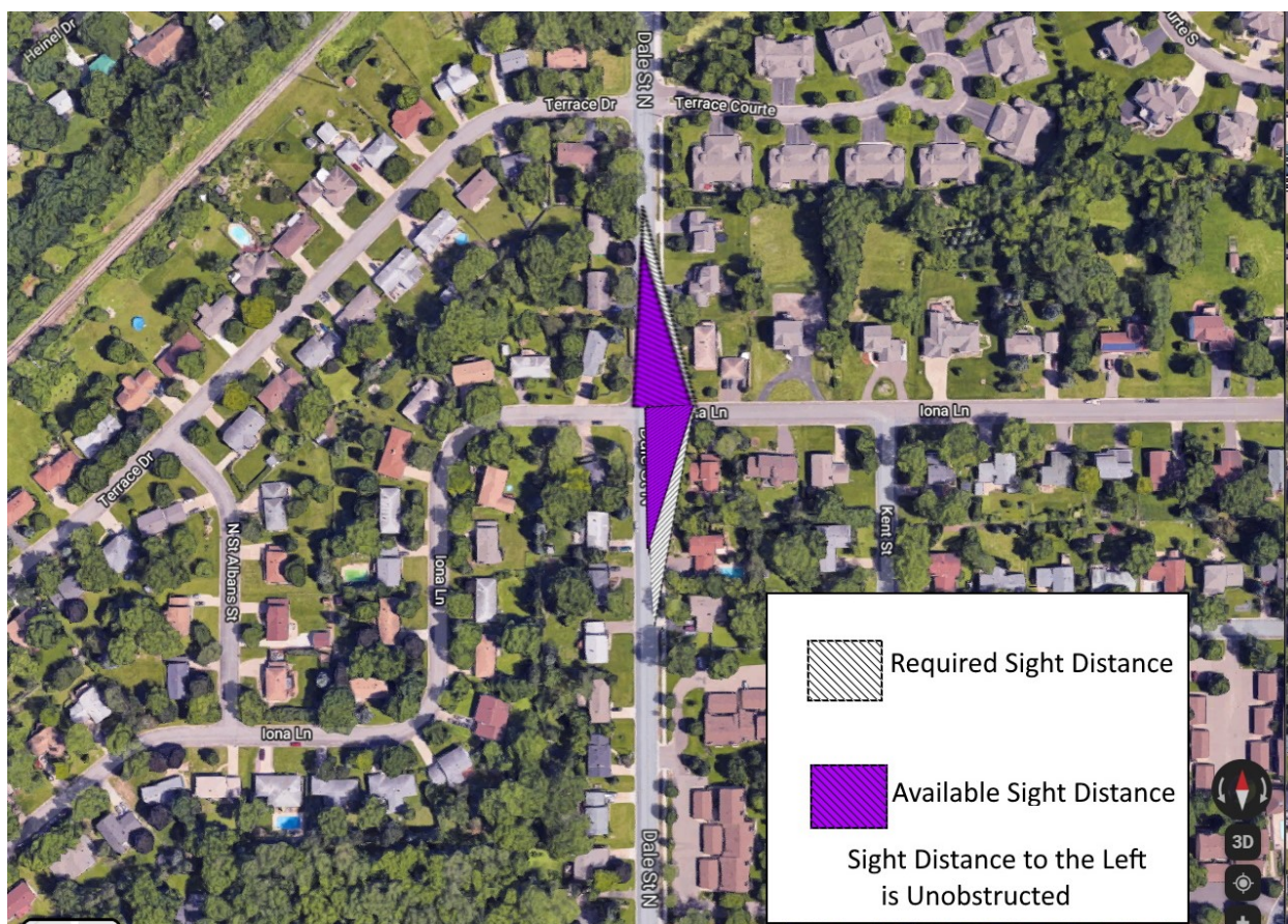
Figure 3.40 Available sight distance and required sight distance at Dale St N and Iona Ln
