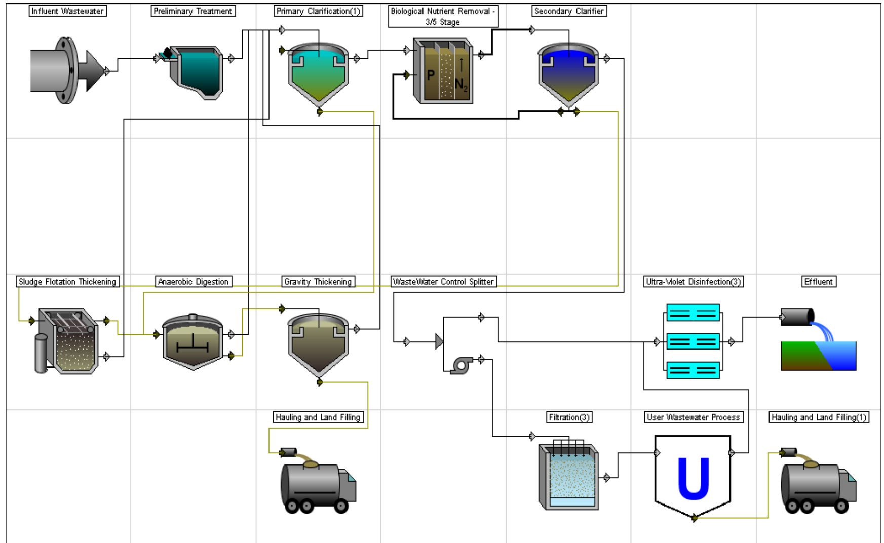
Figure D-4 Process flow diagram of potential WWTF upgrades to meet future WQBELs for Albert Lea
