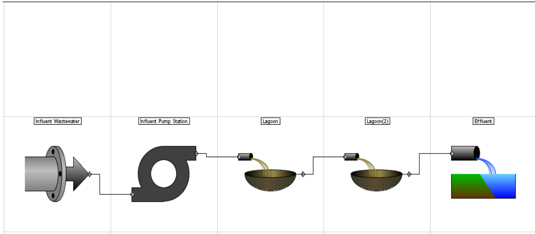
Figure D-4 Process flow diagram of existing Cook WWTF
