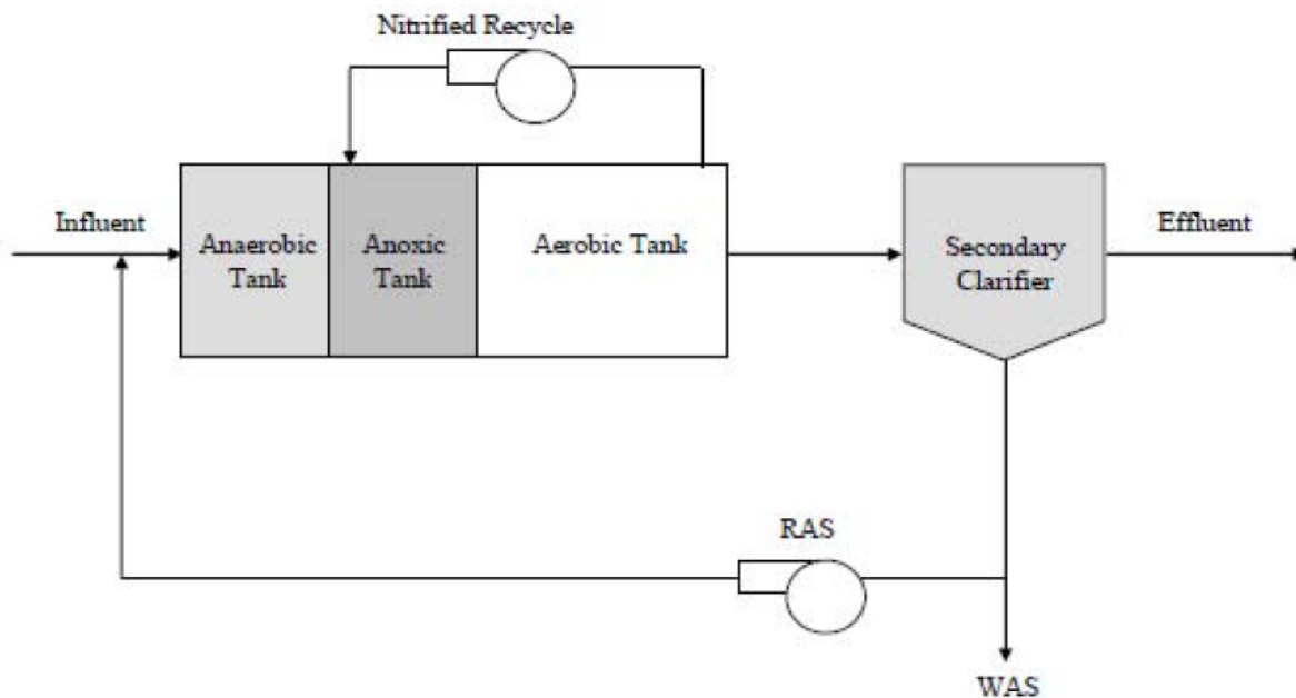
Figure 5-7 3-Stage Pho-Redox (A 2 /O) process flow
