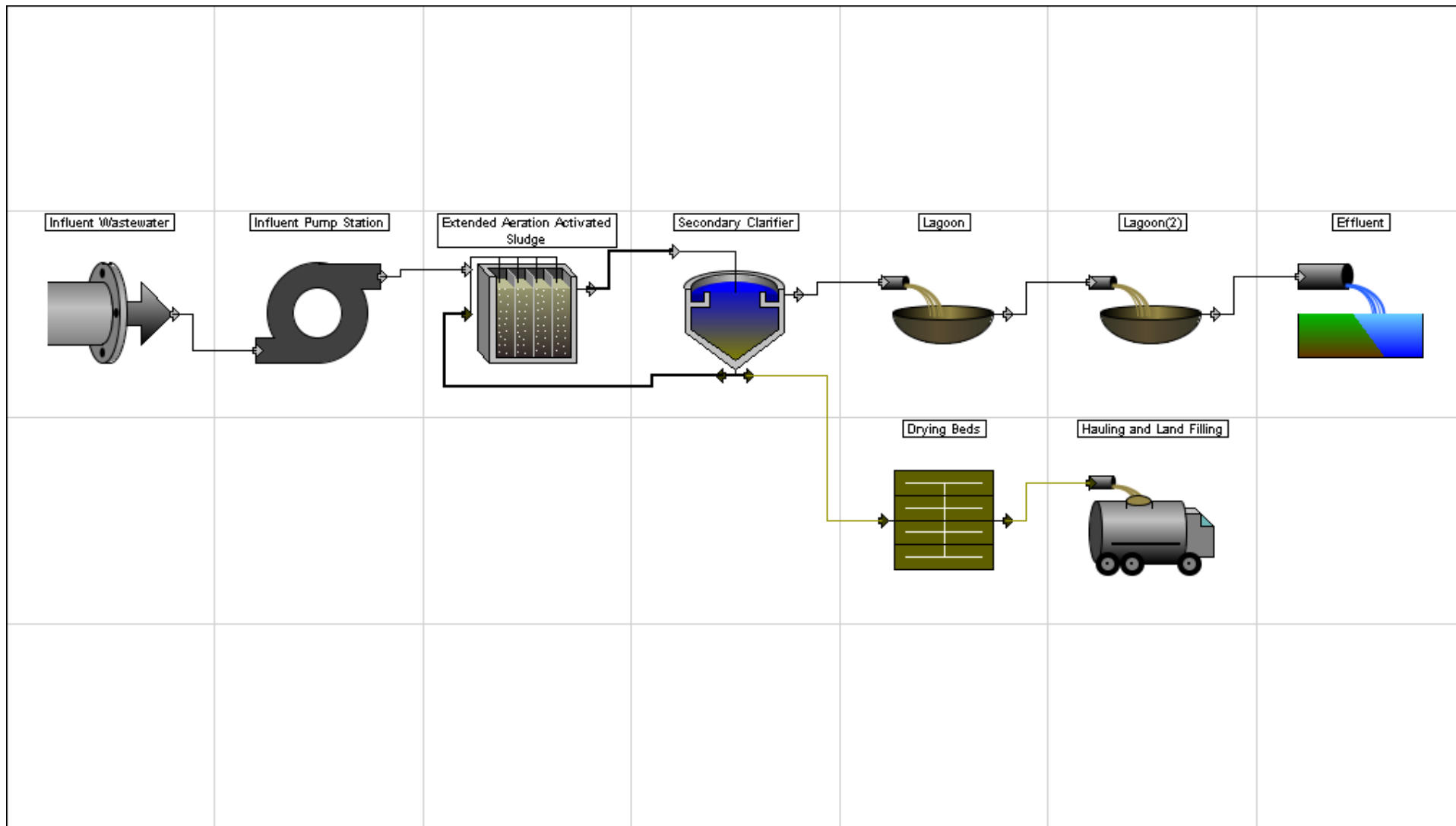
Figure D-2 Process flow diagram of potential WWTF upgrades to meet current WQBELs for Ada
