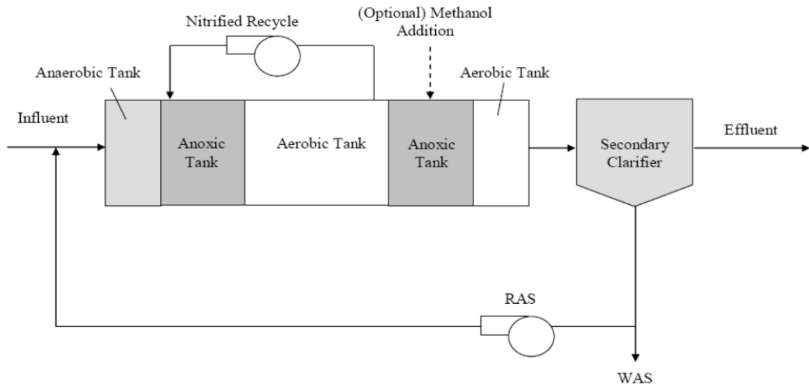
Figure 5-8 5-Stage Bardenpho process flow
