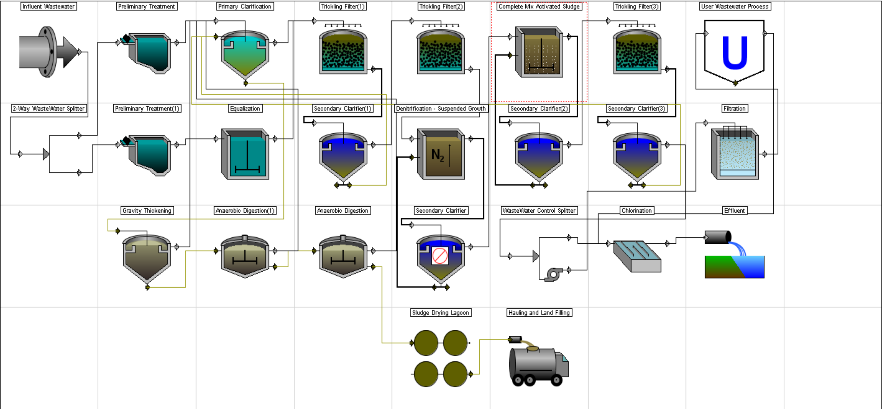
Figure D-3 Process flow diagram of potential WWTF upgrades to meet future WQBELs for Hibbing
