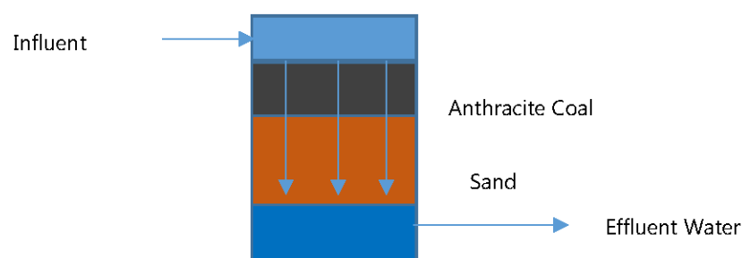
Figure 5-1 Tertiary media depth filtration process flow
