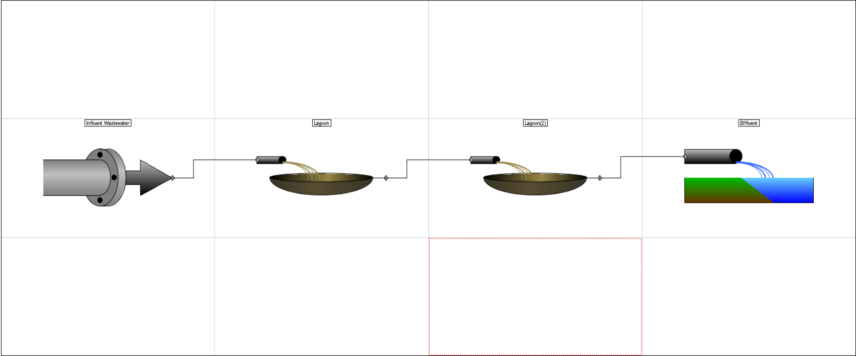
Figure D-1 Process flow diagram of existing Hanska WWTF
