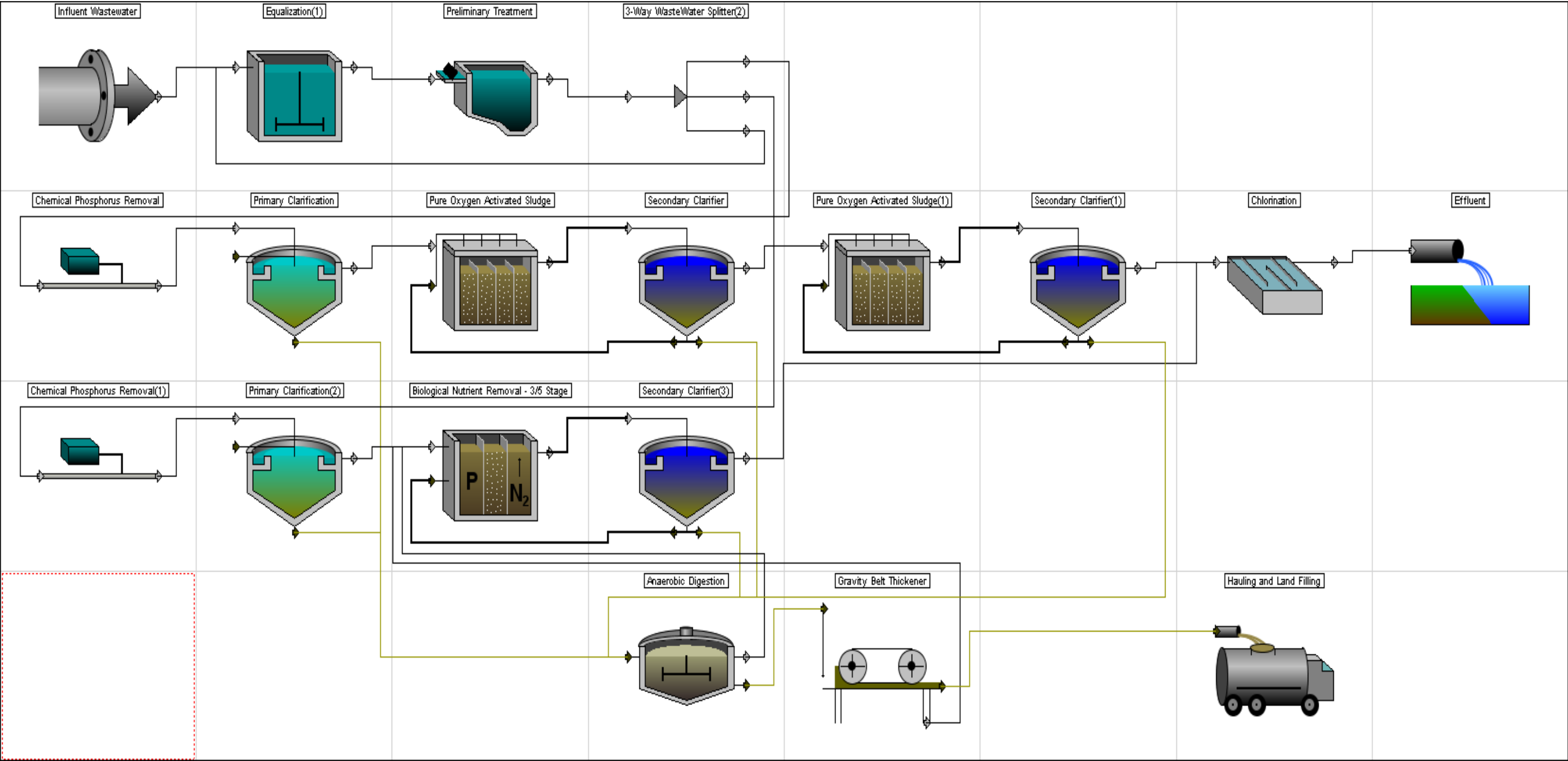
Figure D-1 Process flow diagram of existing Rochester WRP
