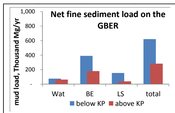
Figure 10: A chart illustrating the relative net sediment contribution from each major watershed, broken down into sediment derived from different geomorphic regimes (above vs. below knickpoint). Data shown are from Scenario 4.
