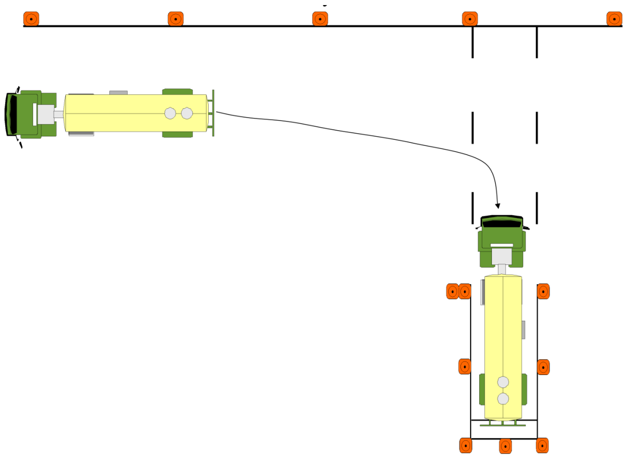
Figure 11.4: Alley Dock
