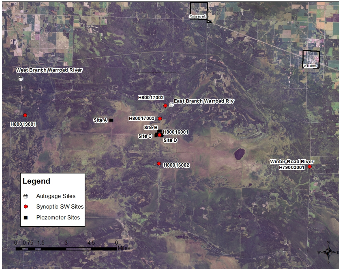
Figure 10: Synoptic Surface Water Measurement Locations with Autogage and Piezometer Locations
