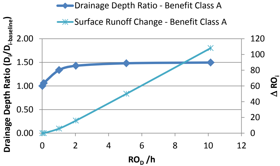
Figure 33. Effect of contributing area on surface runoff under conventional drainage for various drainage depth ratios.
