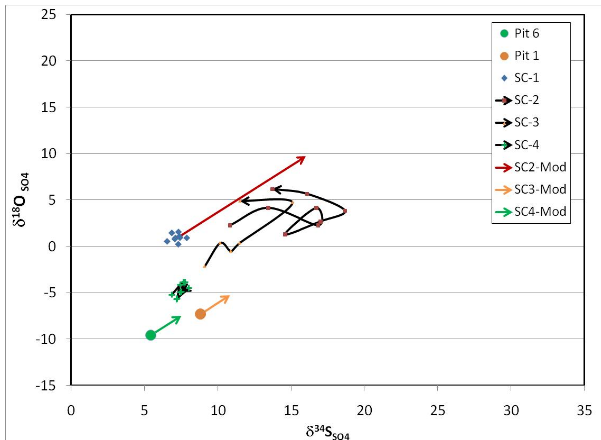
Fig. 13. \delta^{34}\text{S} and \delta^{18}\text{O} values for the dissolved \text{SO}_4^{2-} at SC-1, SC-2, SC-3, SC-4, and for the \text{SO}_4^{2-} in Pits 1 and 6. The arrows connecting the individual data points for each site show the temporal progression of the samples during the season. SC2-Mod, SC3-Mod, and SC4-Mod are the modeled isotopic pathways for reduction of waters from the LTV tailings basin, Pit-1, and Pit-6, respectively. See text for explanation.
