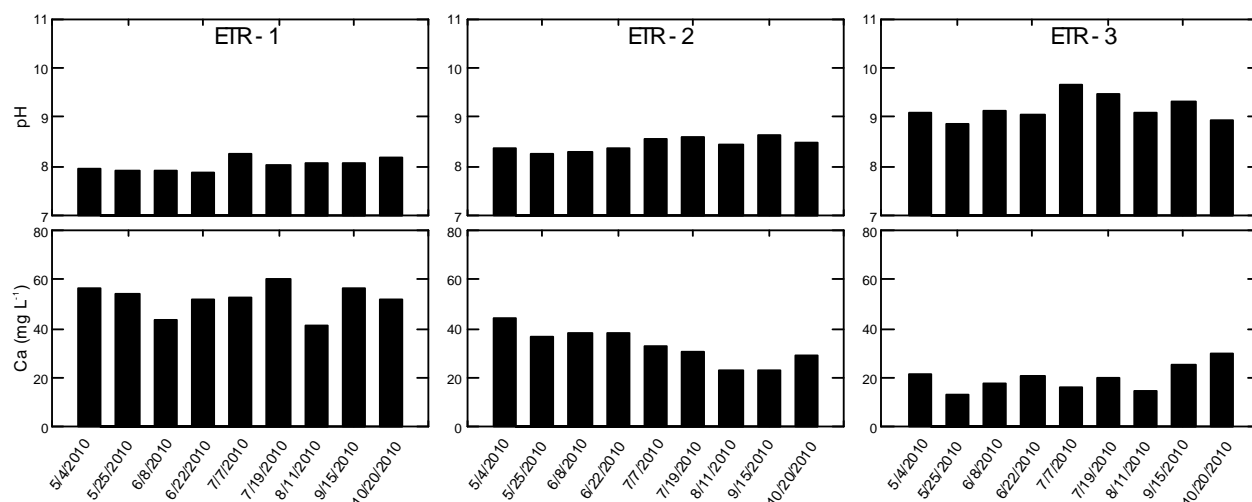
Fig. 18. pH values and Ca concentrations at sampling locations ETR-1 , ETR-2 , and ETR-3 . The large increase in pH and decrease in Ca that occurs in the lake between inlet (ETR-1, and ETR-2) and outlet (ETR-3) sites is indicative of high productivity in the lake, with correspondingly high deposition rates for calcite and organic carbon into the bottom sediments. It is proposed that this high productivity drives \text{SO}_4^{2-} reduction and production of \text{HS}^- and \text{H}_2\text{S} in the bottom sediments, especially during the summer months (when pH is highest in the surface waters – indicative of greater productivity in surface waters). The generation of \text{HS}^- and \text{H}_2\text{S} in bottom sediments is believed, in turn, to generate highly mobile \text{MeHgHS}^0 .
