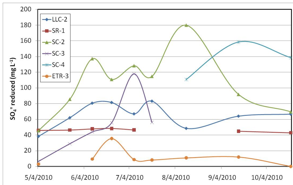
Fig. 19. Sulfur isotope-based estimates of the mass of \text{SO}_4^{=} reduced per liter of water in wetlands and lakes investigated in this study. The plotted values apply to the wetland (LLC-2, SC-3, SC-4), tailings basin (SR-1, SC-2), or lake located immediately upstream from the listed sampling site. The method used to calculate \text{SO}_4^{=} lost relies on the measured changes in \delta^{34}\text{S}_{\text{SO}_4} . Estimates for SR-1 were not available in mid-summer because \text{SO}_4^{=} concentrations were below the levels needed to conduct \delta^{34}\text{S}_{\text{SO}_4} analysis. SC-3 estimates are only available before August because flow at the site subsided after July 1 when pumping from Pit 1 was stopped. SC-4 estimates were only available approximately a month after Pit 1 pumping was stopped because the relative inputs from SC-3 and Pit 6 sites to SC-4 were difficult to unravel before the pumping stopped.
