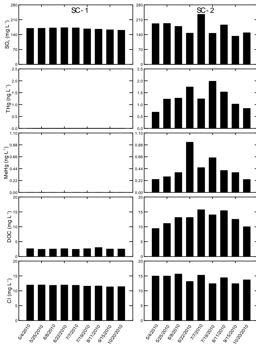
Fig. 12. A comparison of \text{SO}_4^{2-} , THg, MeHg, DOC, and \text{Cl}^- levels in samples collected from sites SC-1 and SC-2. Site SC-1 is at the toe of the former LTV mining company's tailings basin. Site SC-2 is located downstream from this and beyond a wetland complex. The higher \text{SO}_4^{2-} and \text{Cl}^- levels indicate that other waters from the tailings basin containing elevated \text{SO}_4^{2-} and \text{Cl}^- are day-lighting in the wetland.
