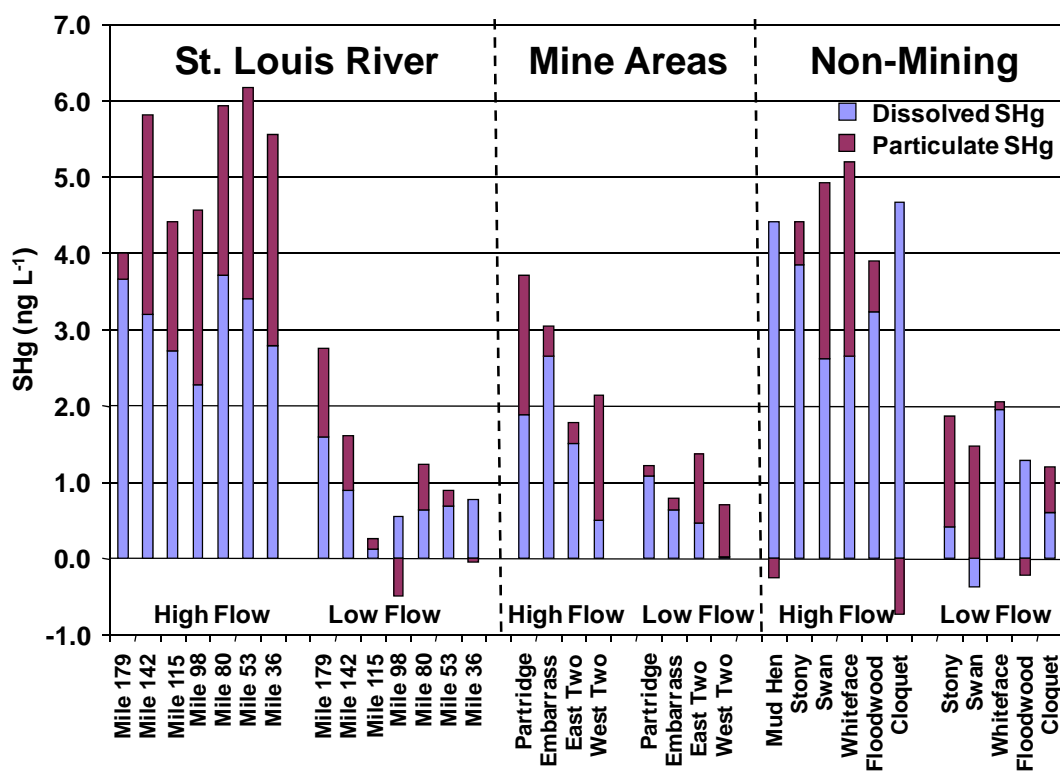
Fig. 10. Dissolved and particulate SHg concentrations calculated for samples collected from the St. Louis River and its tributaries during May and September/October 2008. Slightly negative values represent cases where the filtered samples have slightly higher SHg concentrations than the unfiltered samples.
