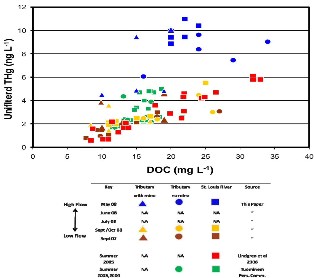
Figure 20. THg and DOC concentrations for unfiltered samples collected from the St. Louis River and its tributaries. This figure also includes THg and DOC data reported by Lindgren et al. (2006) for St. Louis River samples collected in the summer of 2005 (red, moderate to low flow conditions) and unpublished THg and DOC data collected from the summer of 2003 and 2004 for the Western Lake Superior Sanitary District (Tim Tuominen, personal communication). The latter data set are represented by green squares for the St. Louis River samples and green circles for tributaries.
