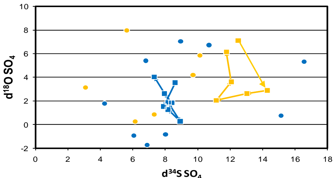
Figure 14. Sulfate isotope values for water in the St. Louis River and its tributaries. The yellow symbols reflect St. Louis River (connected squares) and tributary (circles) samples collected under dry conditions in September 2007. The blue symbols represent St. Louis River (connected squares) and an extended set of tributary samples (circles) collected under wet conditions in June 2008. The very high \delta^{34}\text{S}_{\text{SO}_4} values (15 and greater) were found for Elbow and Long Lake Creeks, which were not sampled during the September sampling trip. The shift to lower \delta^{34}\text{S}_{\text{SO}_4} and \delta^{18}\text{O}_{\text{SO}_4} values for \text{SO}_4 in the St. Louis River under wet conditions (compared to dry conditions) indicates a major change occurred in the relative loading from individual \text{SO}_4 sources. It is suspected that the high \delta^{34}\text{S}_{\text{SO}_4} source represented by the Elbow Creek samples was a very significant contributor of sulfate to the St. Louis River during the dry period. However this component was dominated by the other lower \delta^{34}\text{S}_{\text{SO}_4} sources under wet conditions in June.
