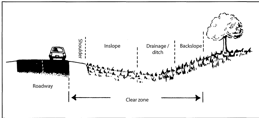
Figure 25. A roadway clear zone in a wooded area specifies standards for conserving trees and providing safe road.
