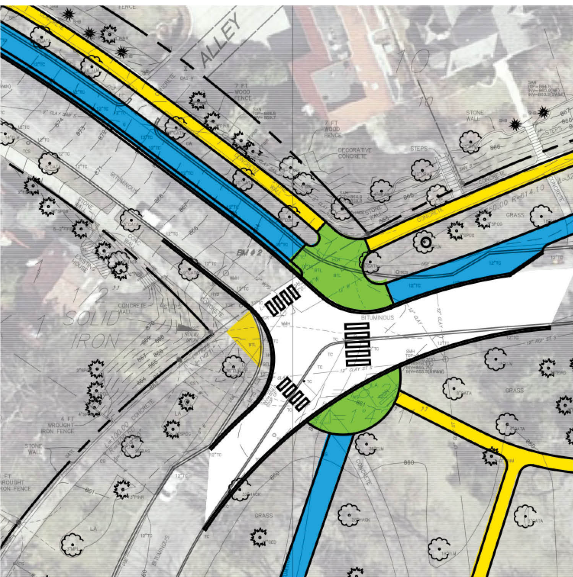
DEAN PARKWAY & WEST CEDAR LAKE INTERSECTION
