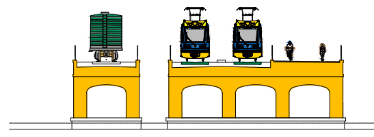
TYPICAL SECTION AT BRIDGE
