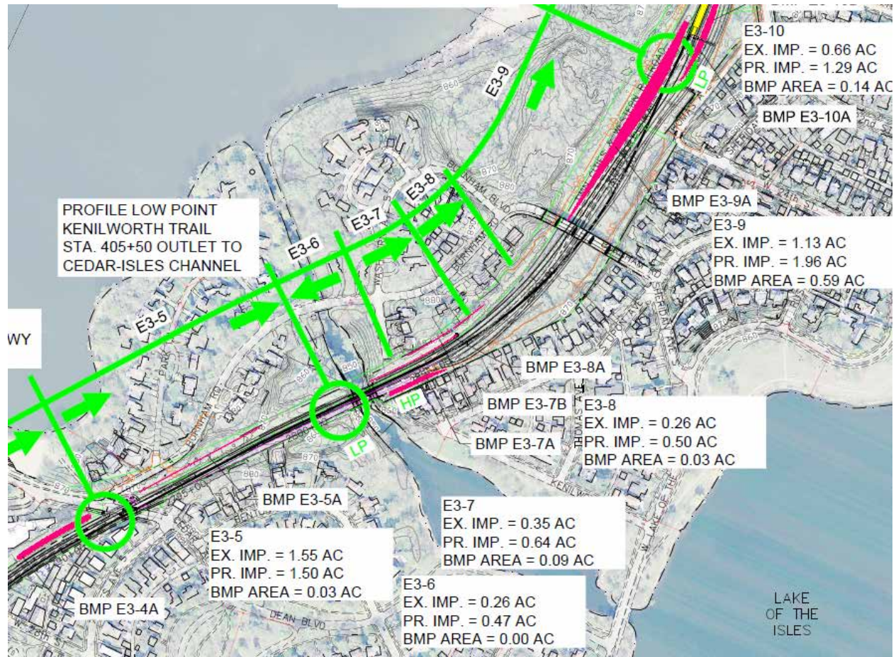
Figure 1 SPO Bridge Option Water Resources Proposed Conditions Map (Segment E3), SPO, September 2014
