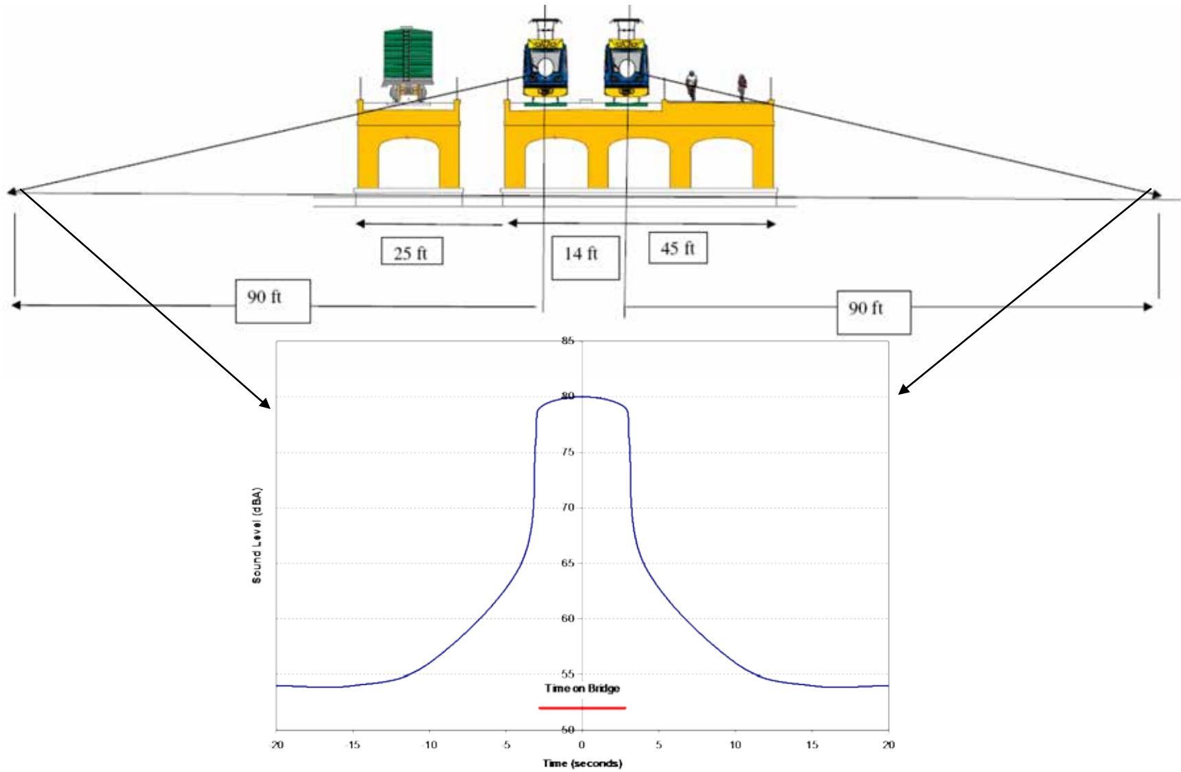
EXHIBIT 9 BRIDGE CROSS SECTION AND ESTIMATE PASS-BY TIME HISTORY ON WATER
