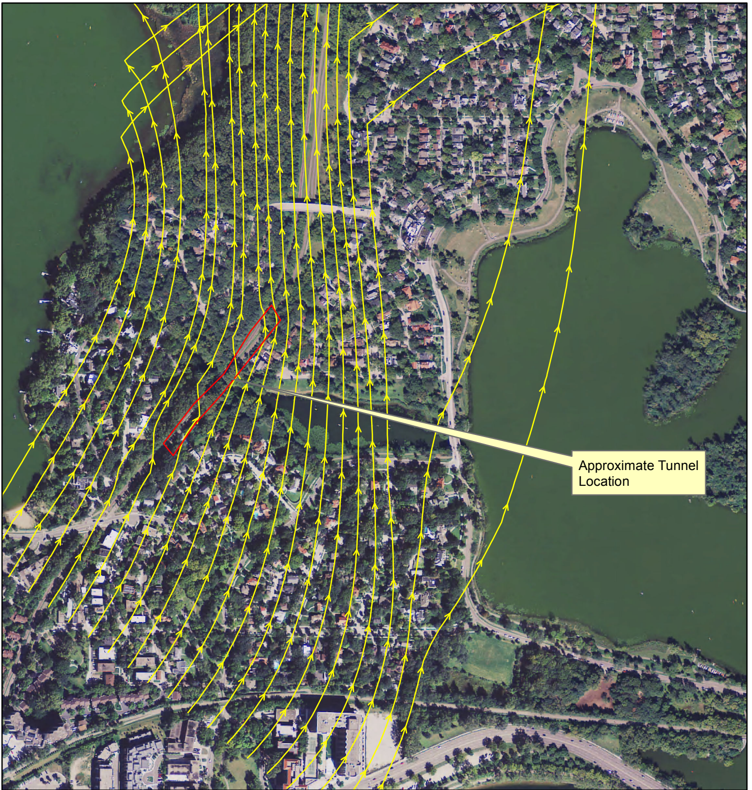
Shallow groundwater flow paths for depths to 60 feet below ground surface
