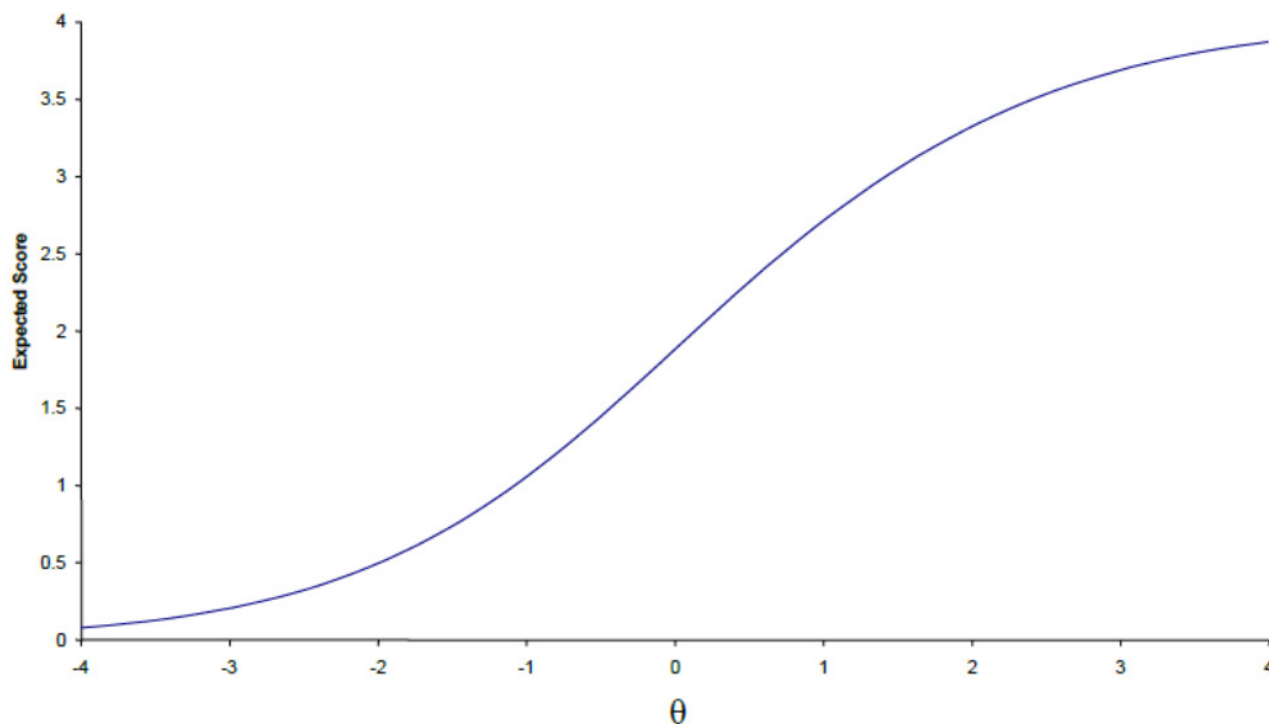
Figure 6.3. Rasch Partial Credit Model Item Expected Score Function for an Example 4-Point Item
