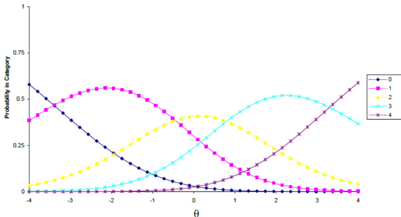
Figure 6.5. Generalized Partial Credit Model Category Response Functions for Sample Polytomous Item with a = 0.4 , b = 0.3 , d_1 = 0 , d_2 = 3.7 , d_3 = 0.75 , d_4 = -0.5 , and d_5 = -3
