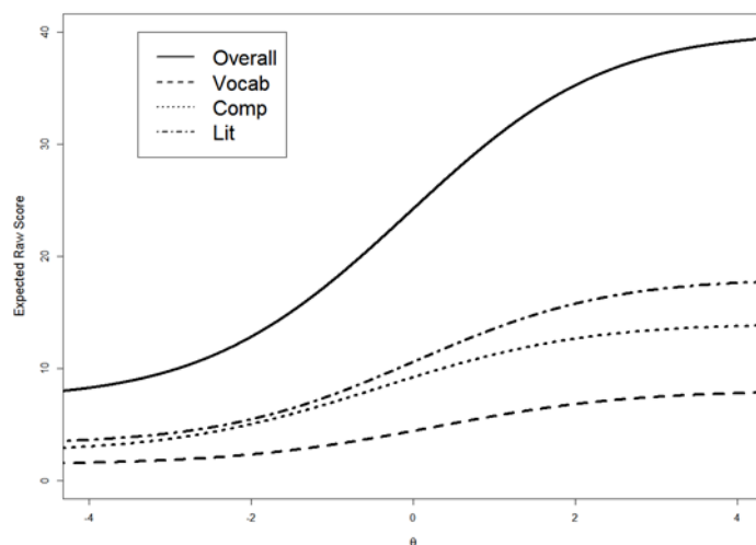
Figure 6.6. Sample Test Response Function for Reading MCA-II
