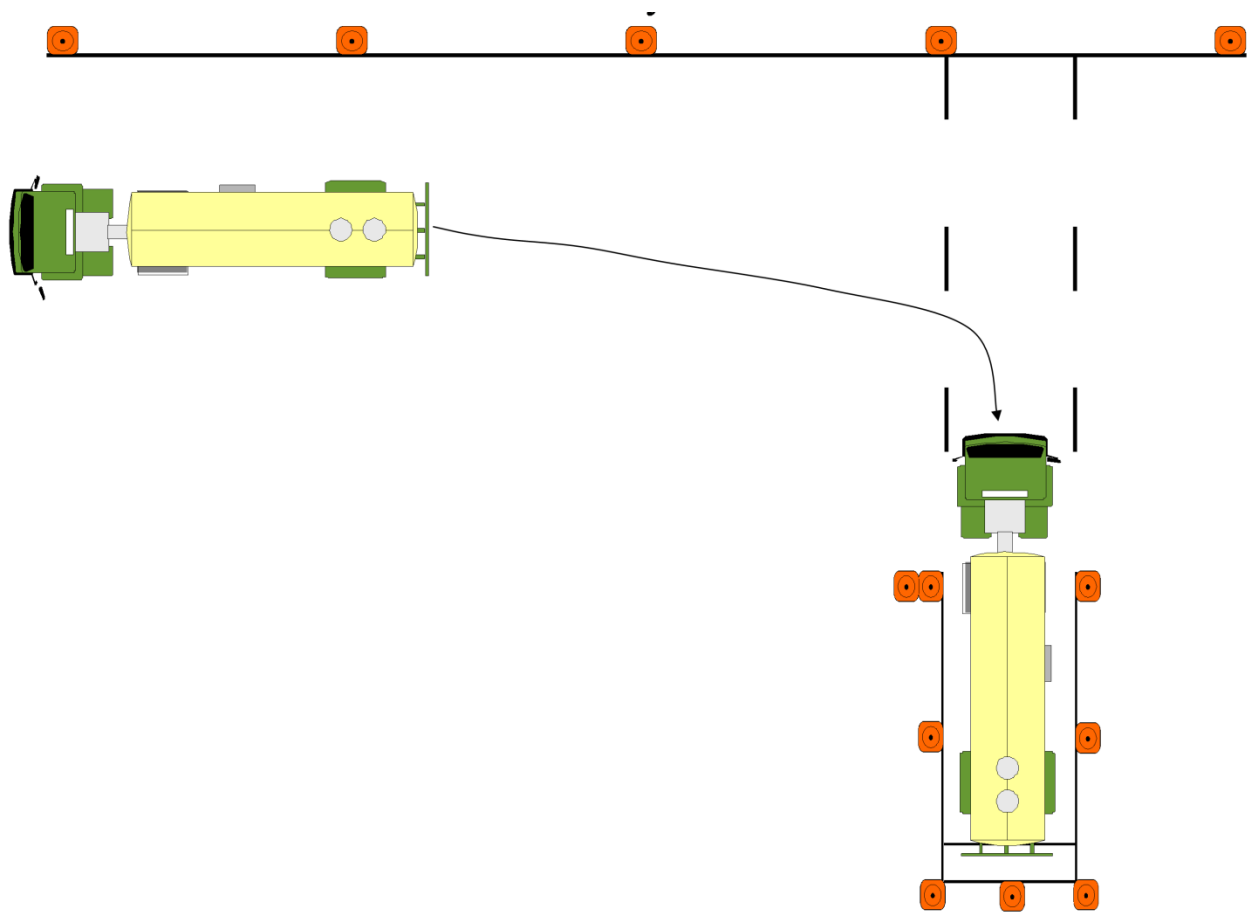
Figure 11.4: Alley Dock
