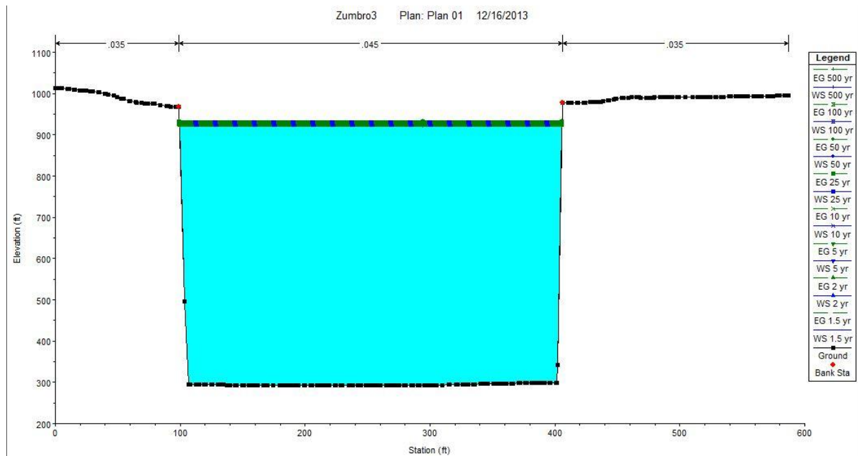
Figure 9. Zumbro River HEC-RAS cross section north of Rochester.
