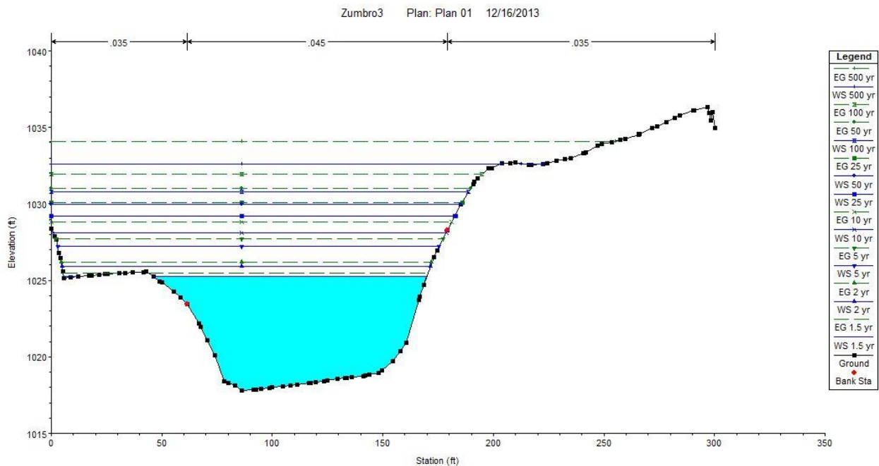
Figure 12. Zumbro River HEC-RAS cross section at Oxbow Park near Byron.
