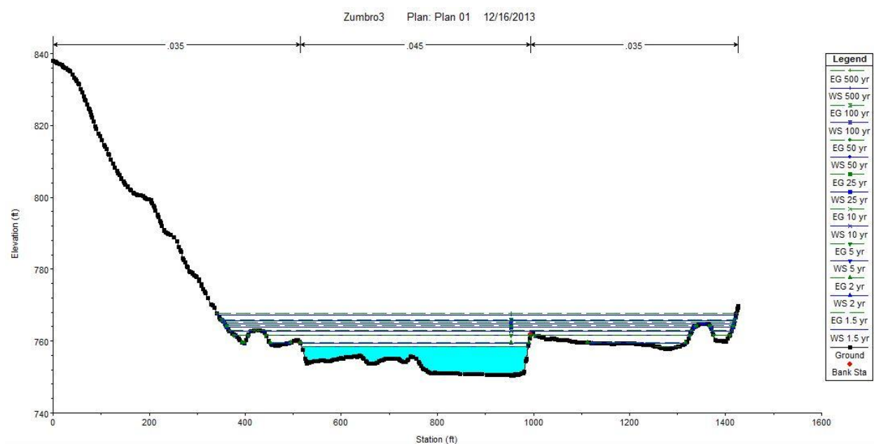
Figure 23. Zumbro River HEC-RAS cross section at Milleville.
