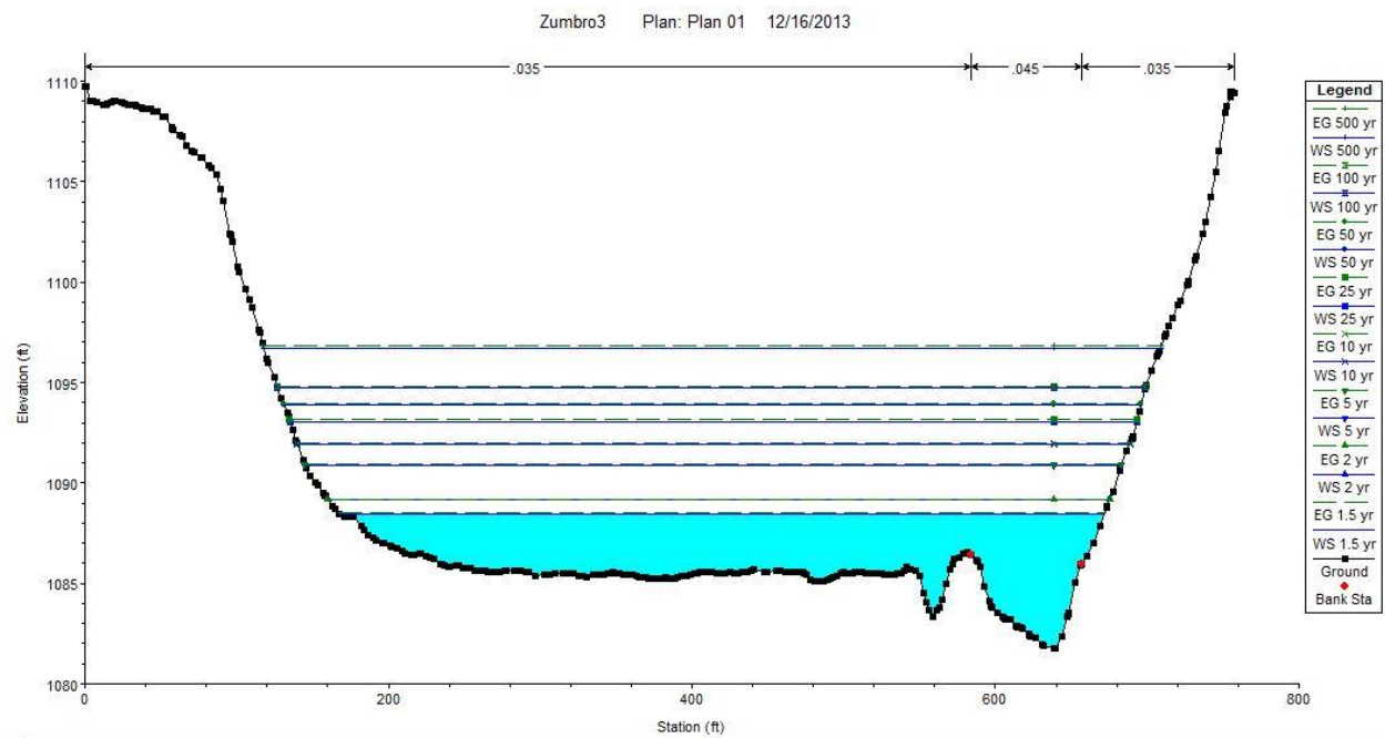
Figure 17. Zumbro River HEC-RAS cross section at Kenyon.
