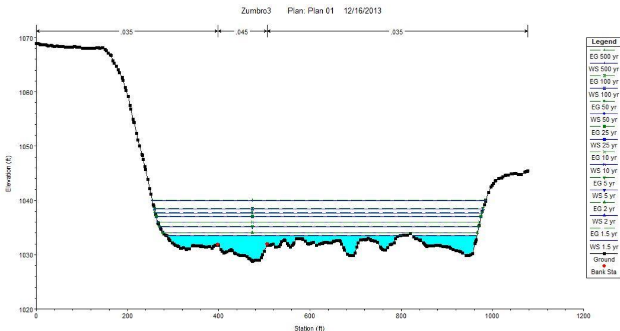
Figure 8. Zumbro River HEC-RAS cross section downstream of Salem Creek.
