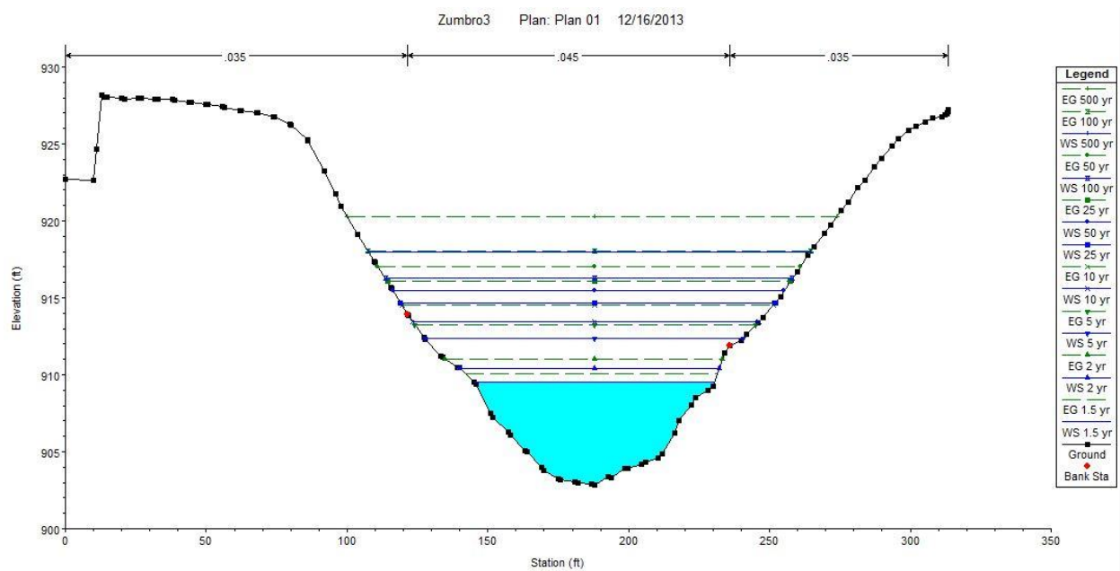
Figure 20. Zumbro River HEC-RAS cross section at Mazeppa.
