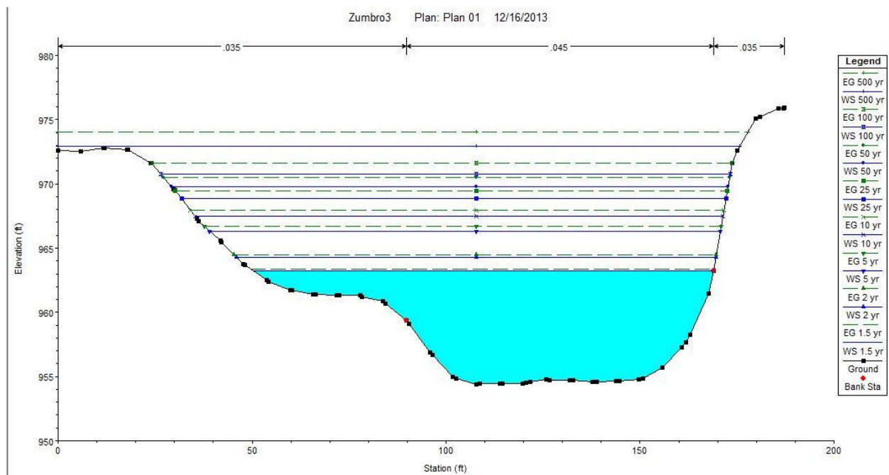
Figure 19. Zumbro River HEC-RAS cross section at Zumbrota.
