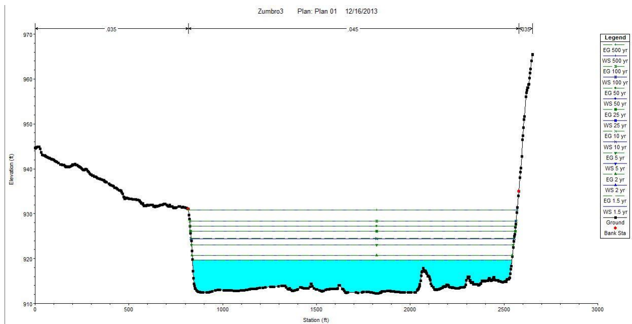
Figure 10. Zumbro River HEC-RAS cross section at Zumbro Lake.
