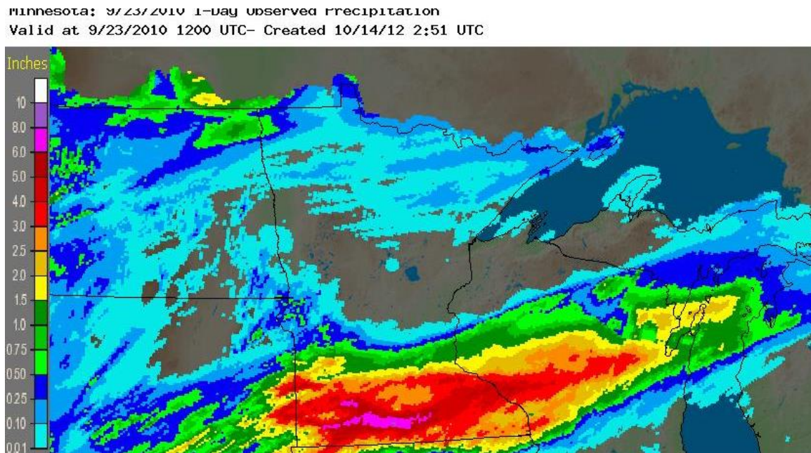
Figure 2. NOAA Doppler radar rainfall record.
