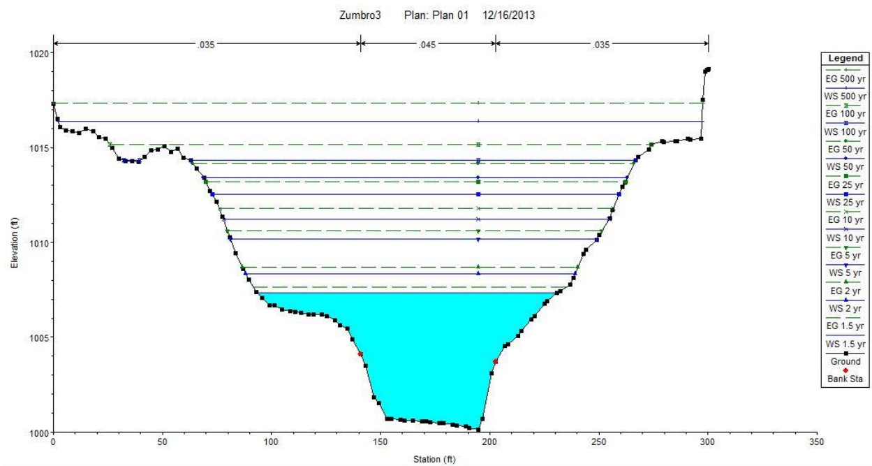
Figure 18. Zumbro River HEC-RAS cross section at Wanamingo.
