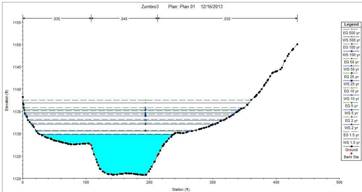
Figure 11. Zumbro River HEC-RAS cross section at Mantorville.
