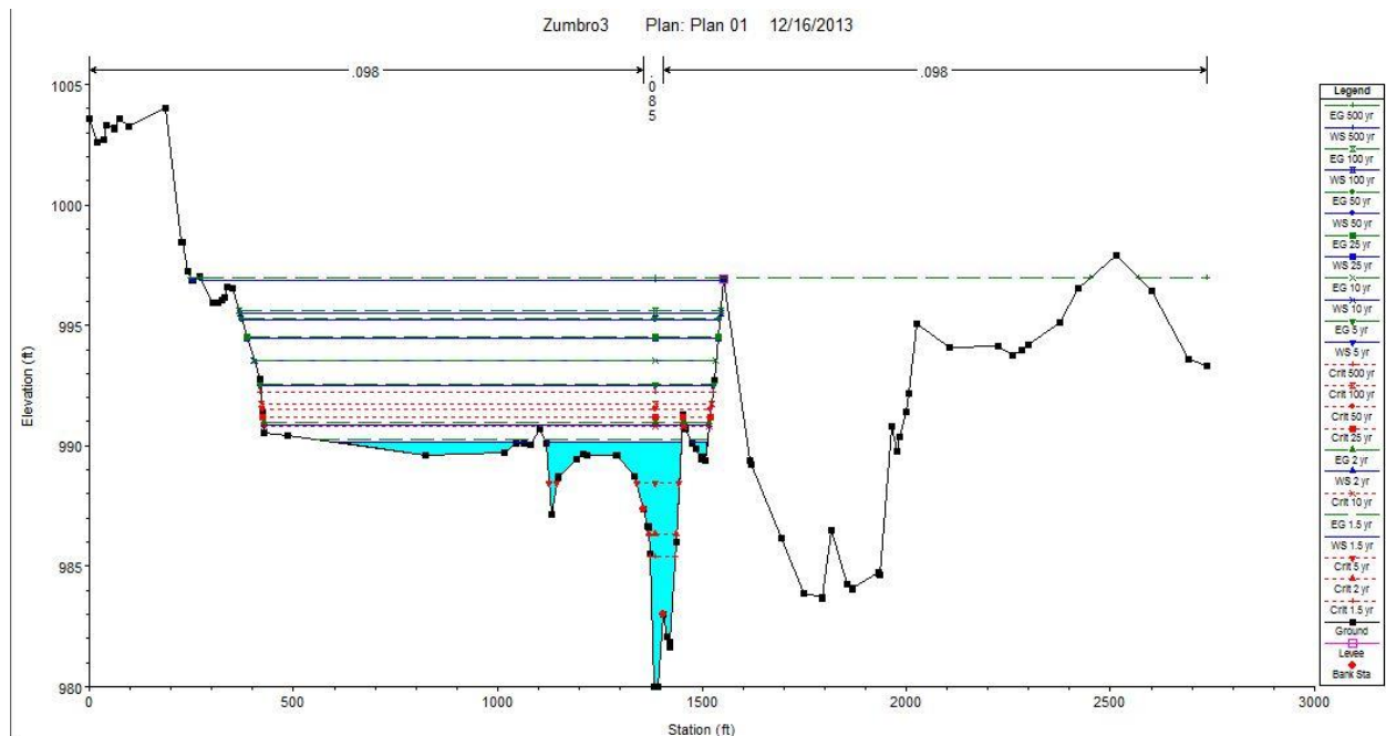
Figure 14. Zumbro River HEC-RAS cross section just upstream (southwest) of Pine Island.
