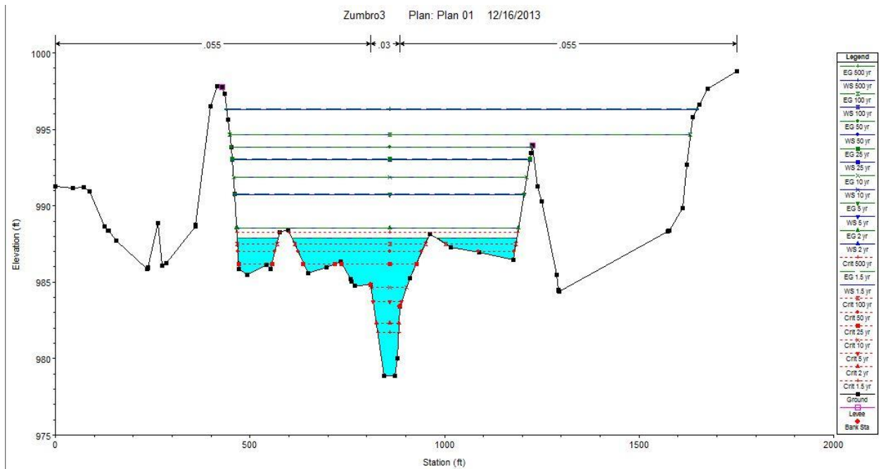
Figure 15. Zumbro River HEC-RAS cross section just upstream (northwest) of Pine Island.
