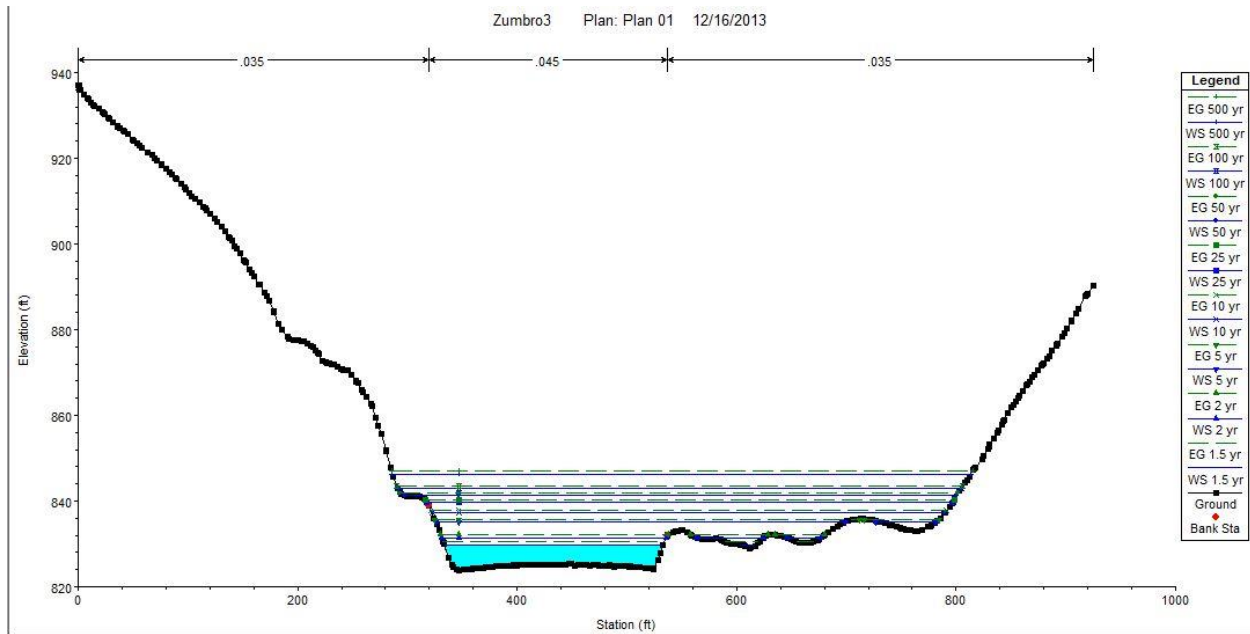
Figure 21. Zumbro River HEC-RAS cross section at Zumbro Falls.
