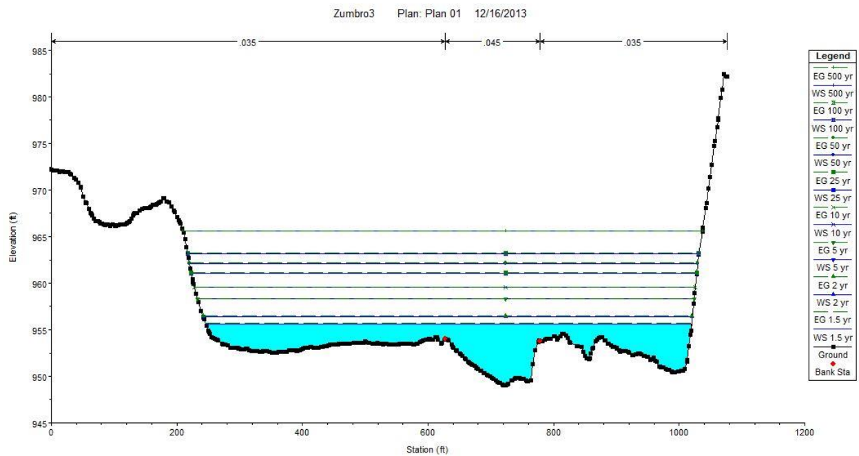
Figure 13. Zumbro River HEC-RAS cross section upstream (southwest) of Oronoco.
