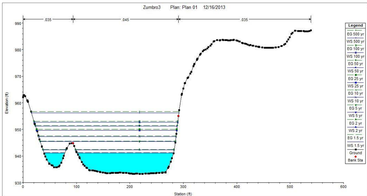
Figure 16. Zumbro River HEC-RAS cross section just below Oronoco.
