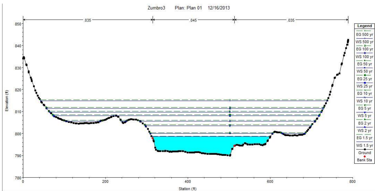
Figure 22. Zumbro River HEC-RAS cross section at Hammond.
