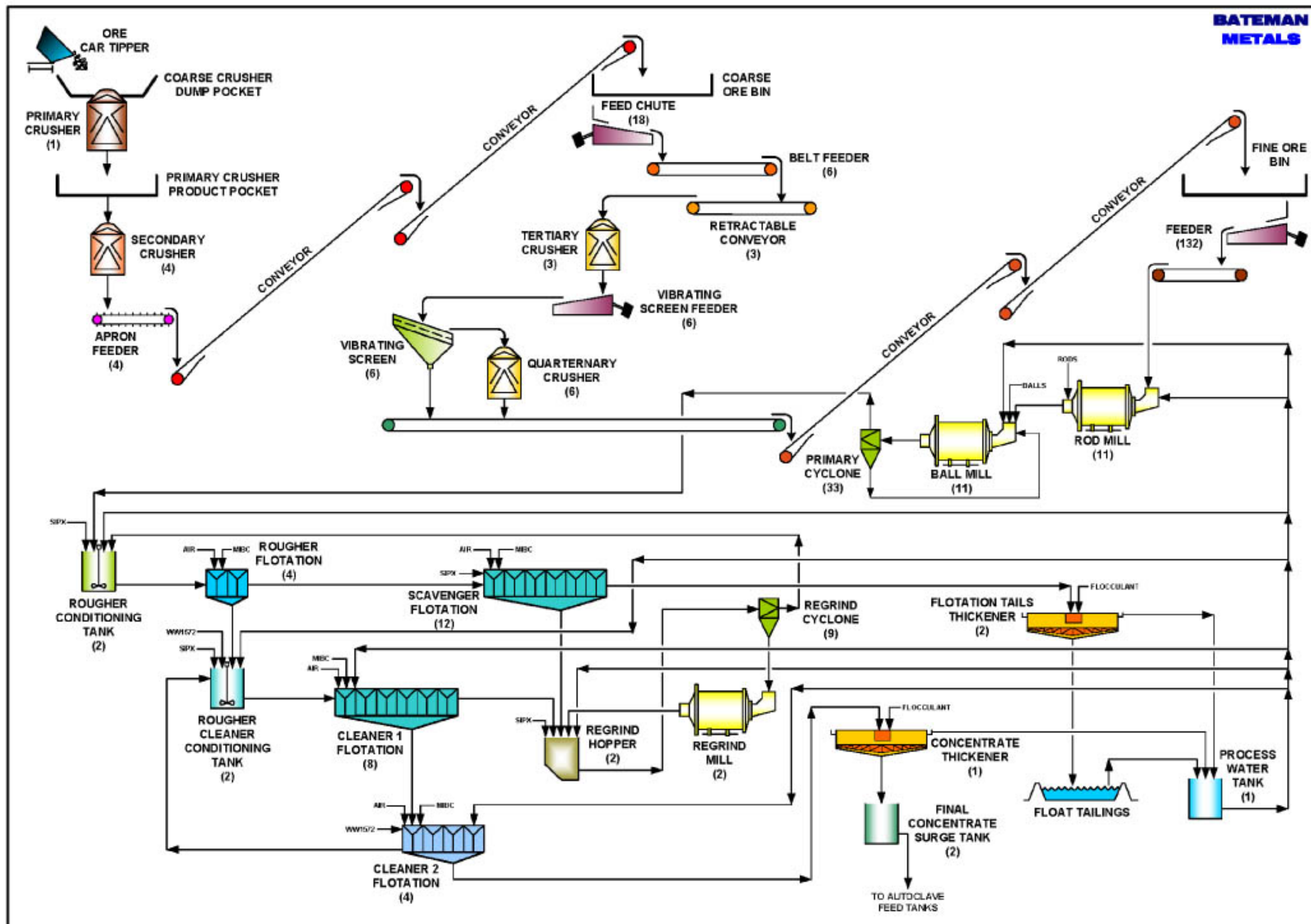
Figure 6-2 COMMUNITION AND FLOTATION SCHEMATIC DIAGRAM
