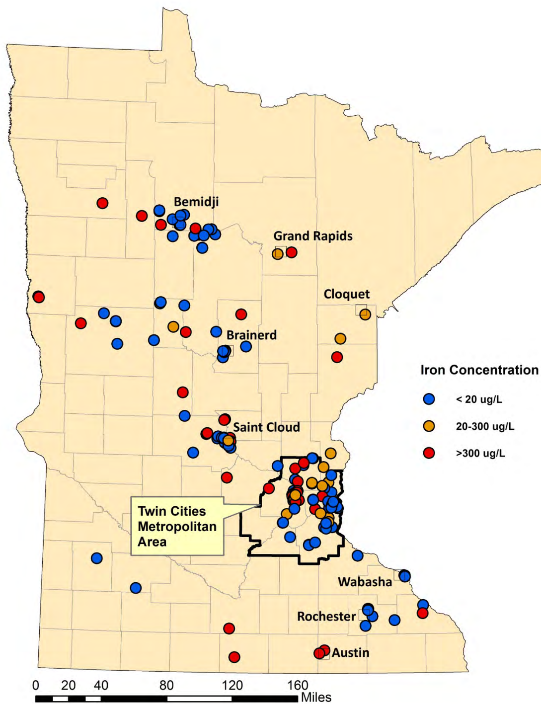
Figure 16. Iron concentrations in Minnesota's ambient groundwater, 2007-2011 [Data from the Minnesota Pollution Control Agency's Ambient Groundwater Monitoring Network].
