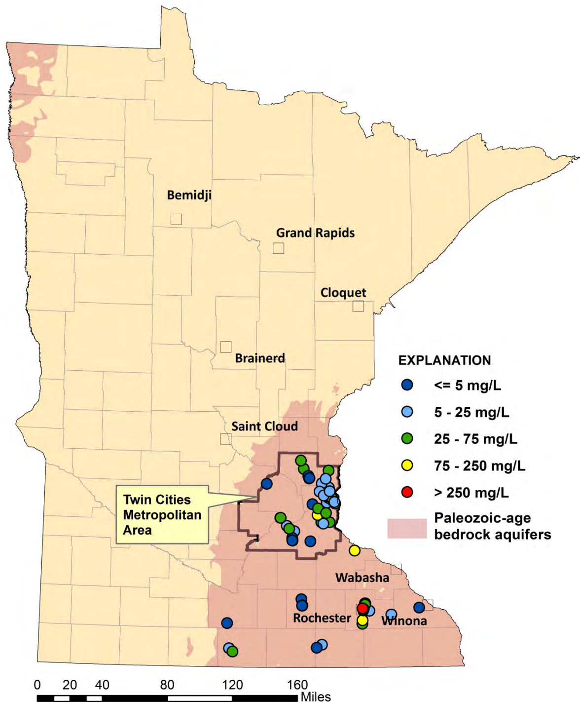
Figure 8. Chloride concentrations in the ambient groundwater from selected Paleozoic-age bedrock aquifers in Minnesota, 2007-2011
