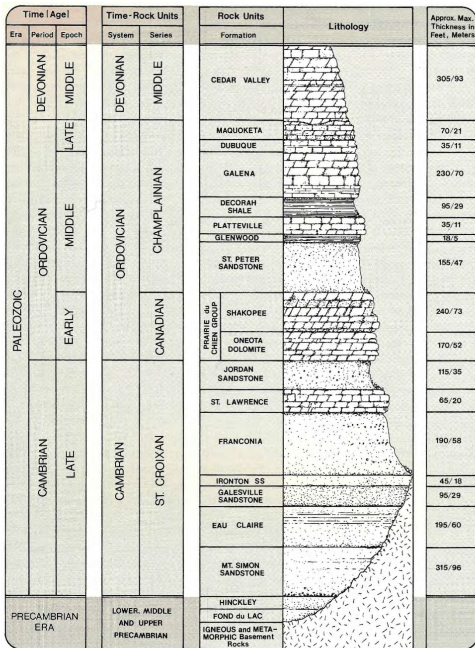
Figure 1. Stratigraphic column of the bedrock aquifers in Southeastern Minnesota [Ojakangas et al., 1982]
