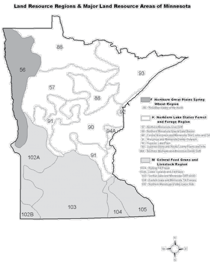
Figure 8.1b Land Resource Regions and Major Land Resource Areas of Minnesota
