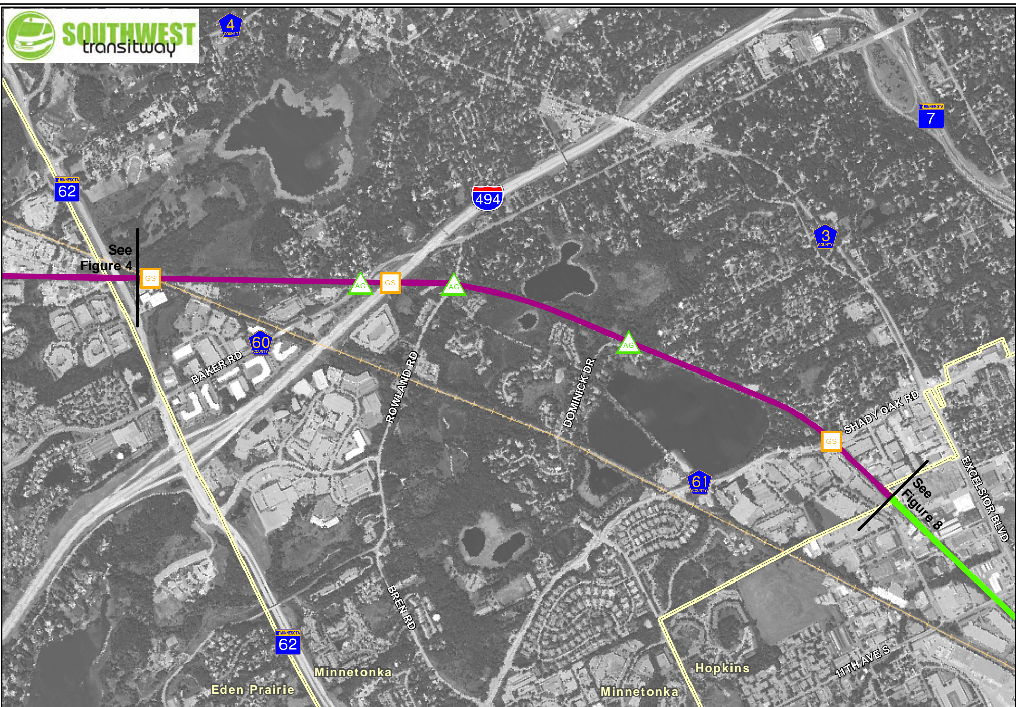
Figure 5 Major Segment 1 Alignments and Intersection Location Codes
