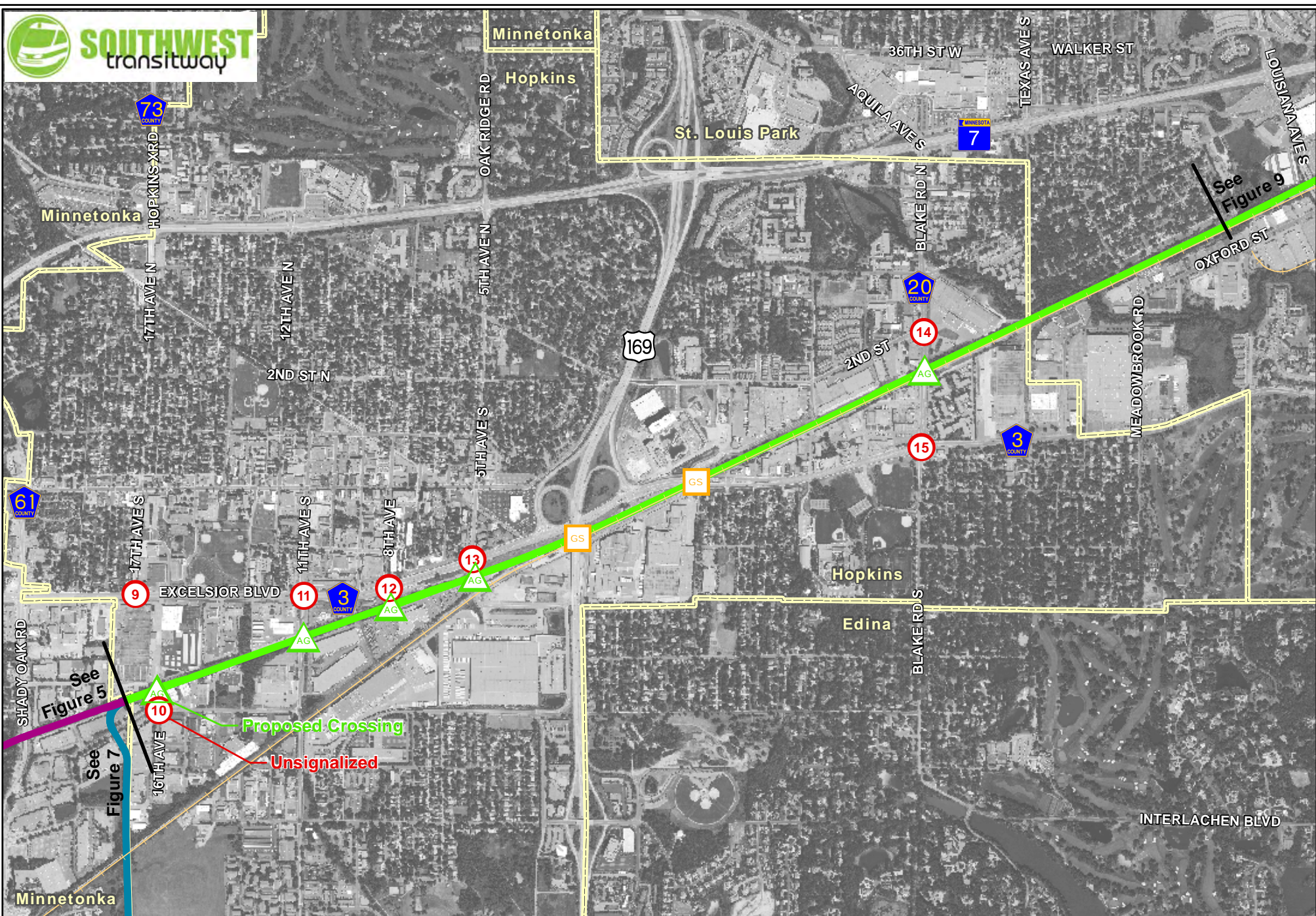
Figure 8 Major Segment 4 Alignments and Intersection Location Codes
