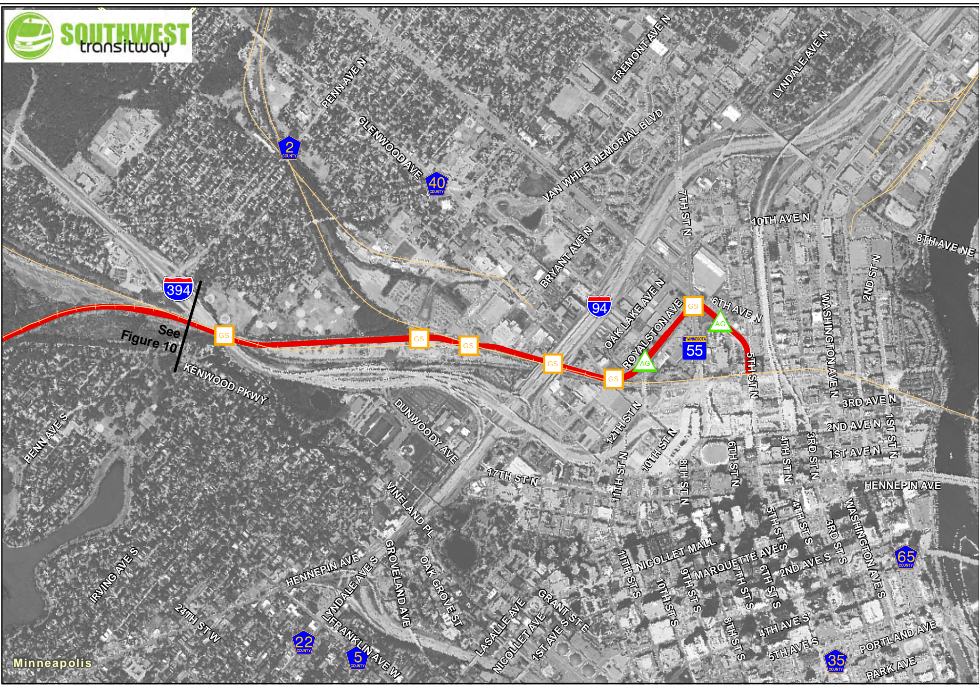
Figure 11 Major Segment A Alignments and Intersection Location Codes
