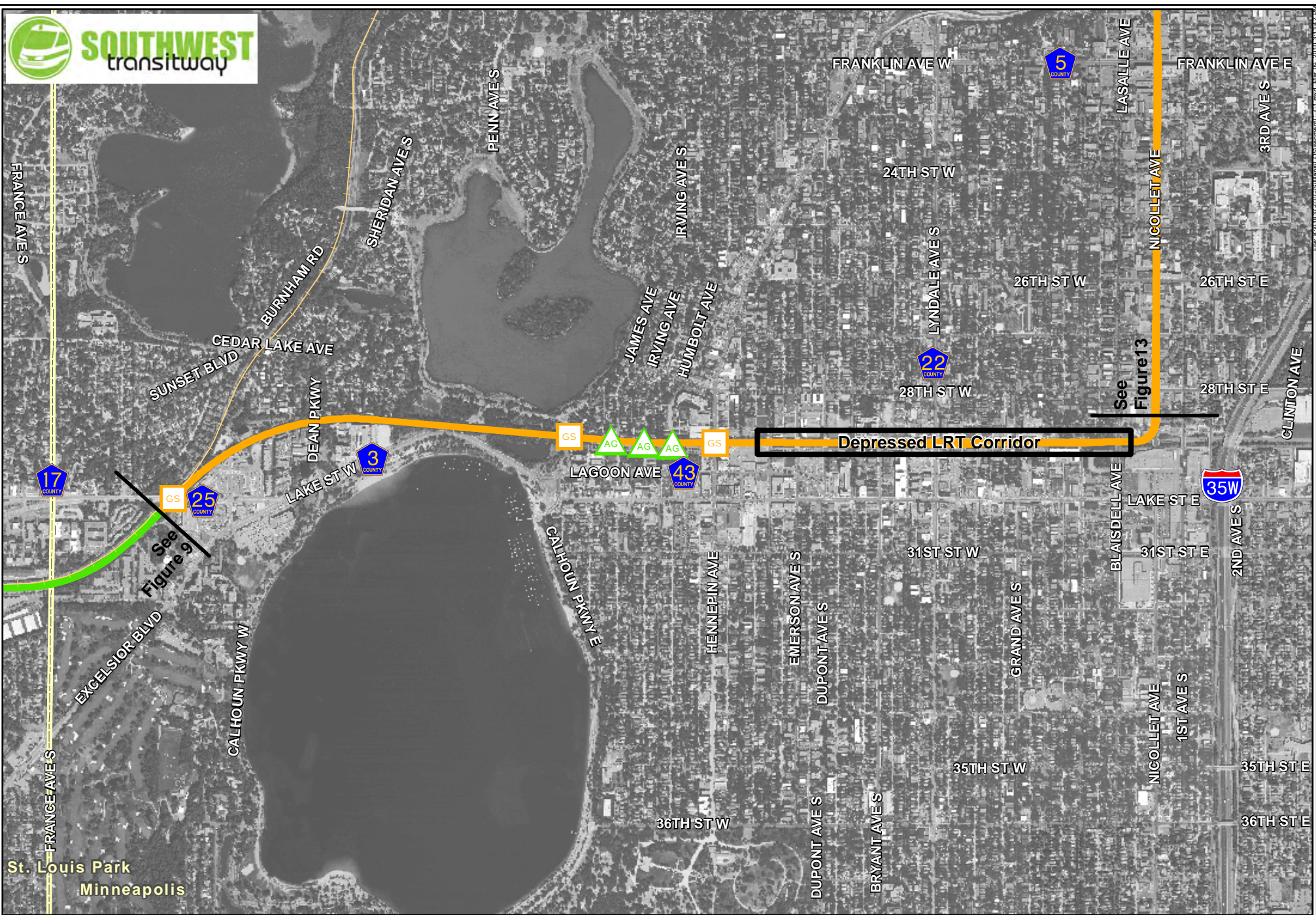
Figure 12 Major Segment C Alignments and Intersection Location Codes
