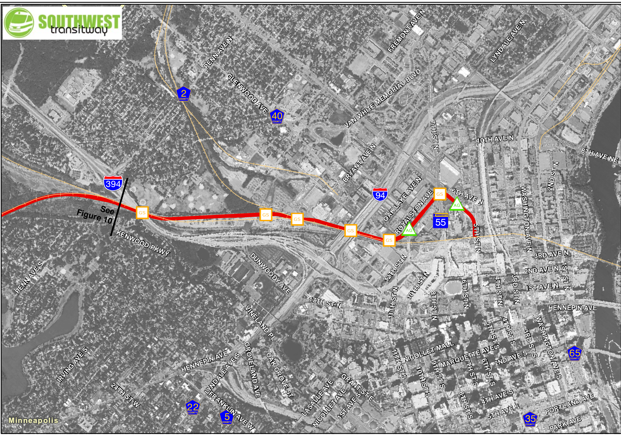
Figure 12 Major Segment A Alignments and Intersection Location Codes
