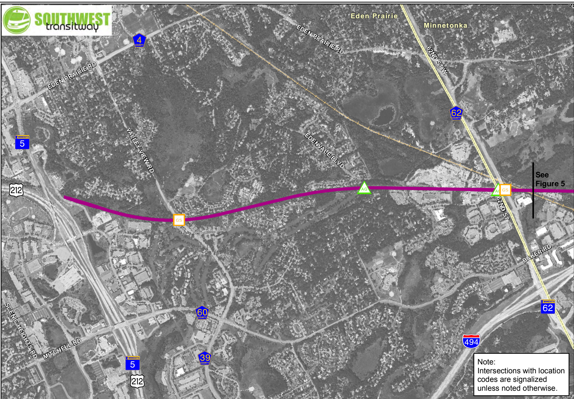
Figure 4 Major Segment 1 Alignments and Intersection Location Codes
