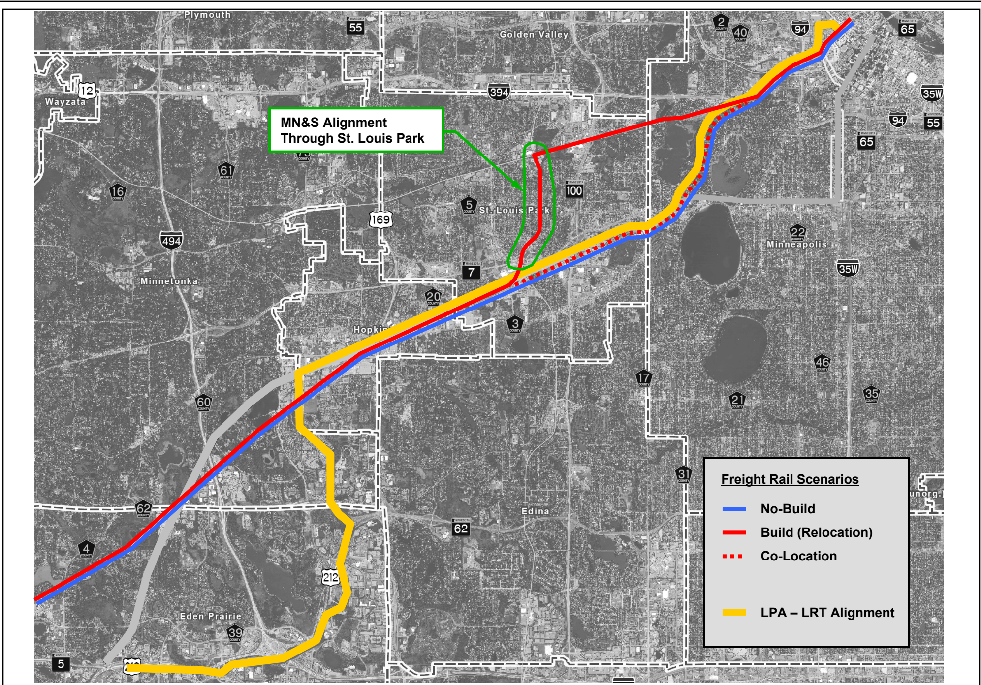
Figure 3 Freight Rail Scenarios
