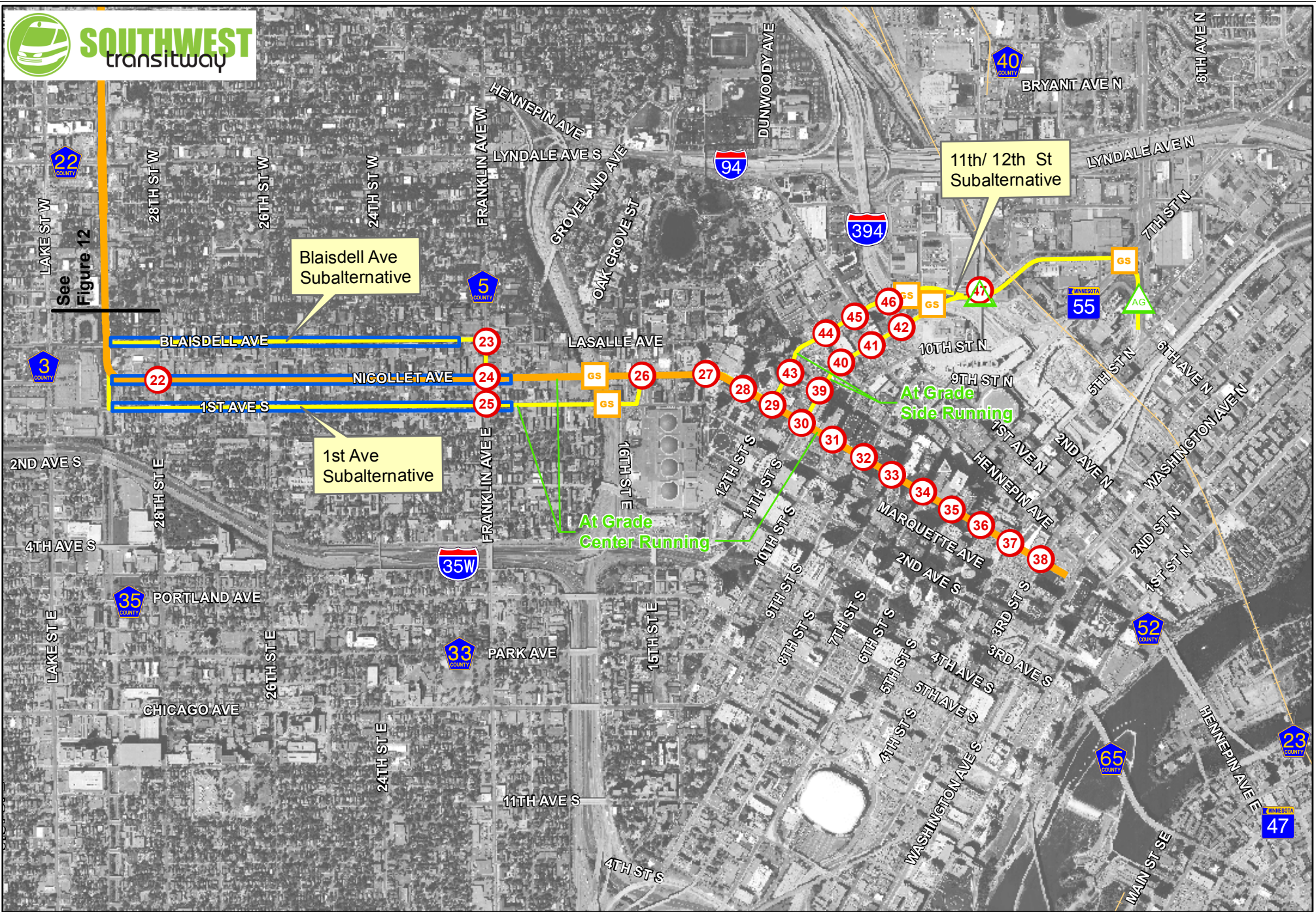
Figure 14 Major Segment C Alignments and Intersection Location Codes
