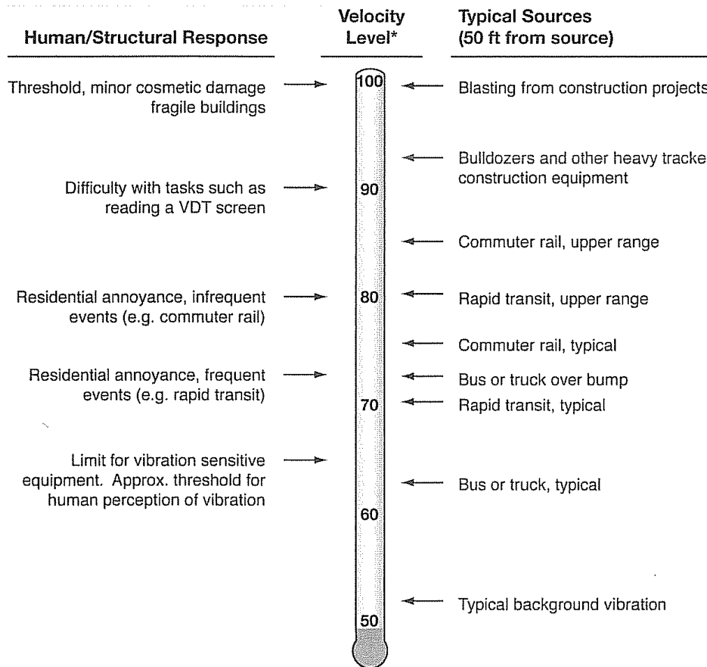
Figure 1. Common Vibration Sources
