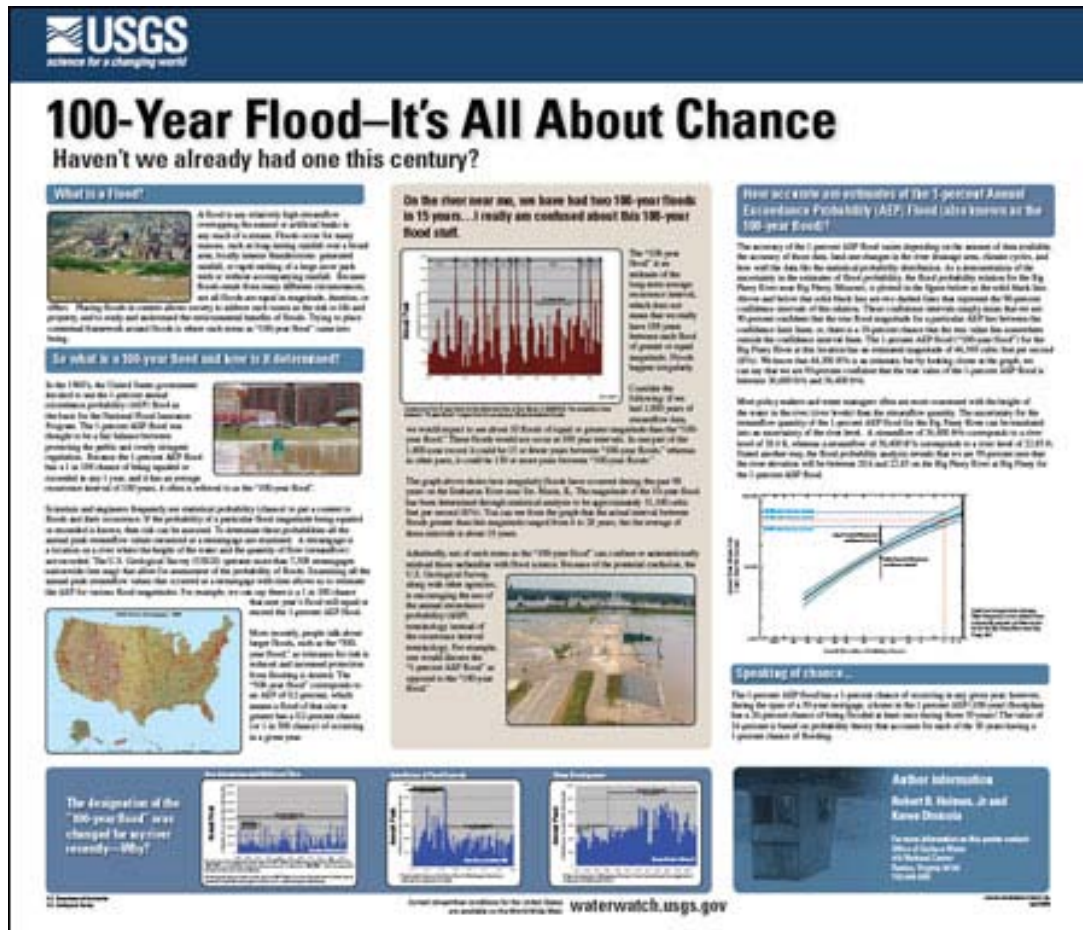
Figure 11 100-Year Flood
