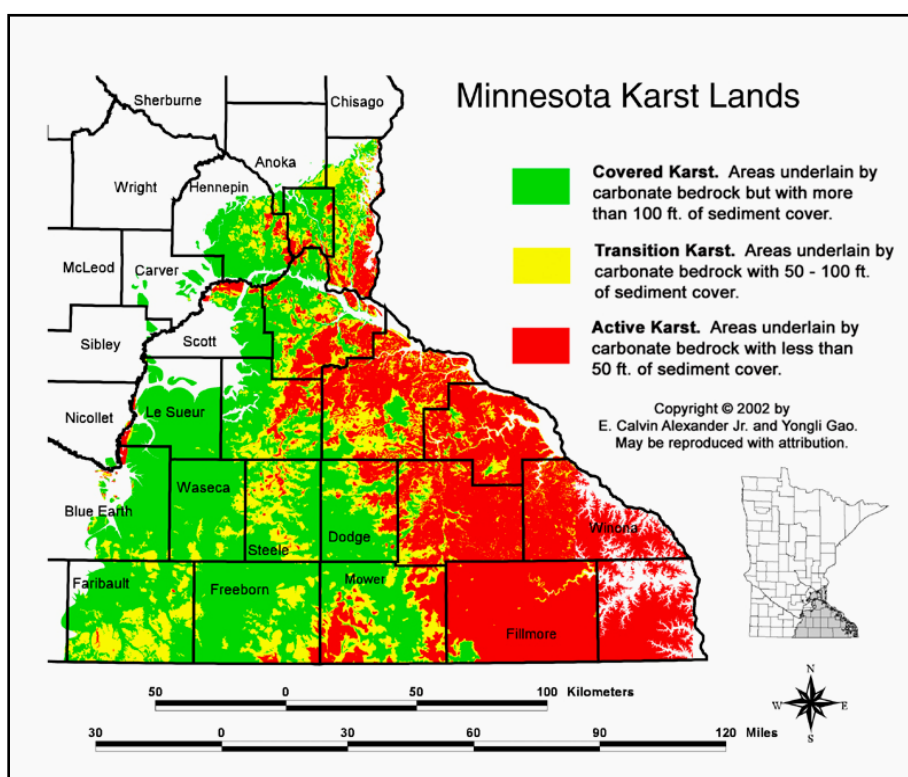
Figure 36 Minnesota Karst
