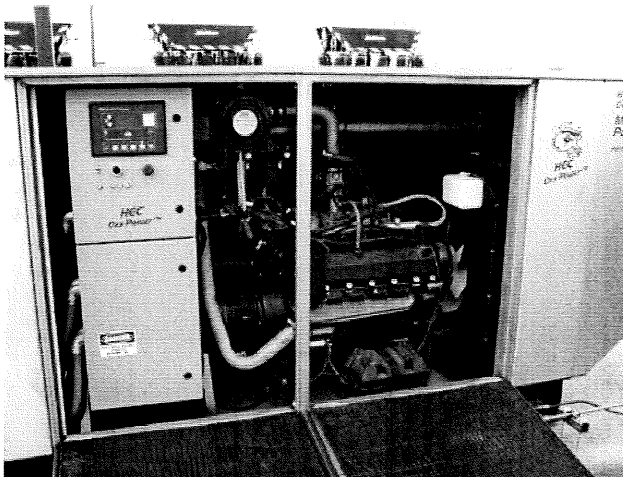
Picture 3. 60 kW hydrogen engine generator set
