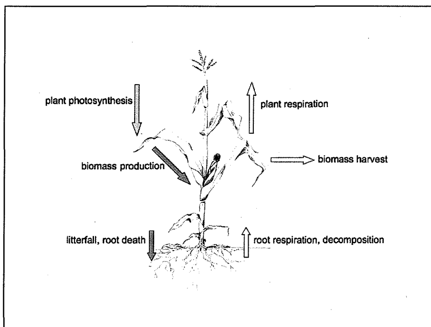
Fig. 1. A simplified diagram of C cycling in a terrestrial plant-soil system. Green arrows indicate CO 2 uptake by plants through photosynthesis. Orange arrows indicate incorporation of C into biomass and C inputs to soil from the death of plant parts (litterfall and root death). Yellow arrows indicate C return to the atmosphere through plant respiration or through the decomposition of litter and soil C by soil organisms. Carbon in harvested tissues also eventually returns to the atmosphere during digestion (by humans and animals), combustion, or eventual decomposition.
