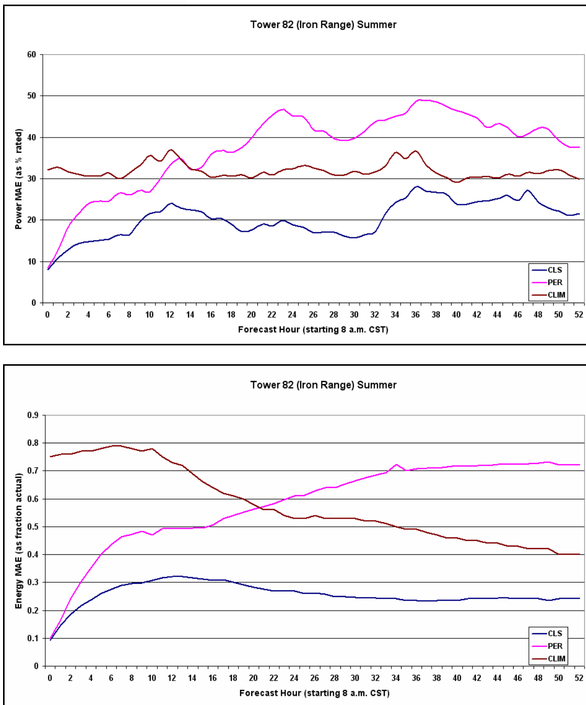
Figure 95: Power mean absolute error (top) and energy mean absolute error as a fraction of actual production (bottom) as a function of forecast hour for the summer months (June, July, Aug.) for the CLS, climatology (CLIM), and persistence (PER) forecasts for Tower 82 (Iron Range).
