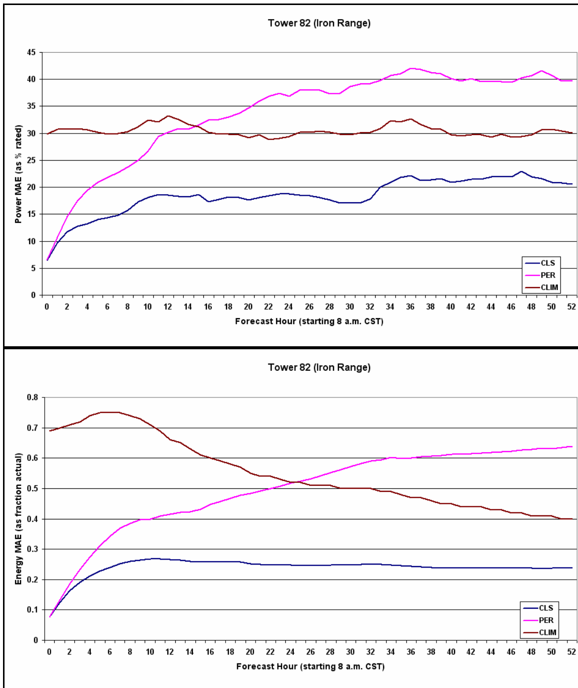
Figure 91: Power mean absolute error (top) and energy mean absolute error (bottom) as a function of forecast hour for all months for the CLS, climatology (CLIM), and persistence (PER) forecasts for Tower 82 (Iron Range).
