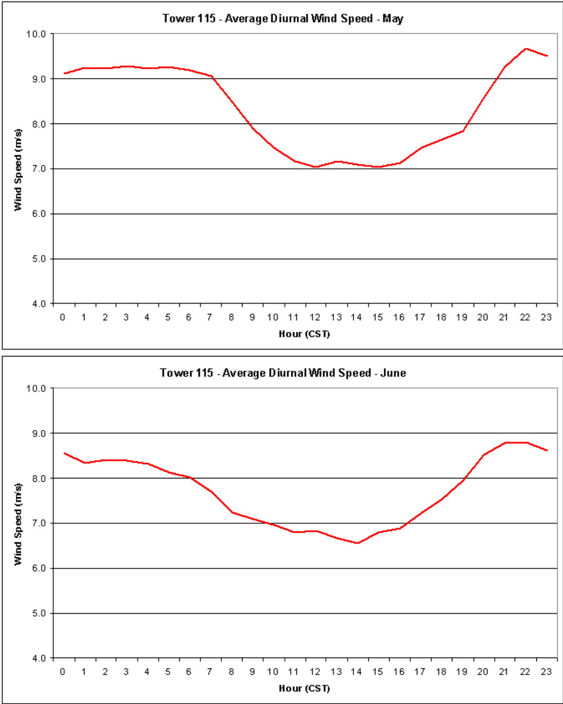
Figure 85: Average May and June 80 m diurnal wind speed at Tower 115 in m/s.
