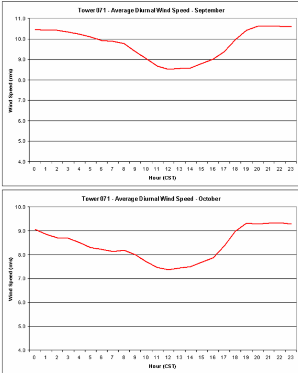
Figure 66: Average September and October 80 m diurnal wind speed at Tower 71 in m/s.
