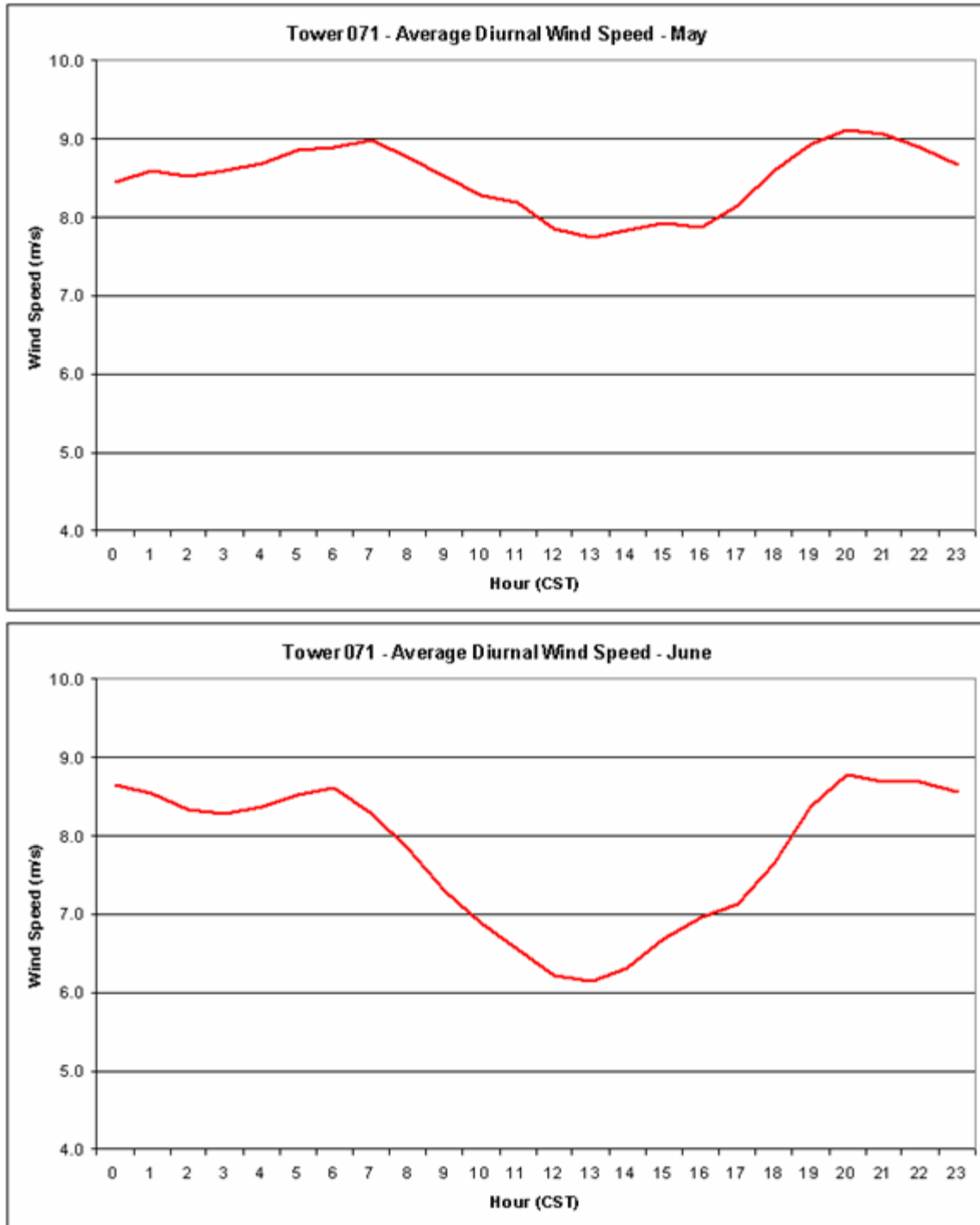
Figure 64: Average May and June 80 m diurnal wind speed at Tower 71 in m/s.
