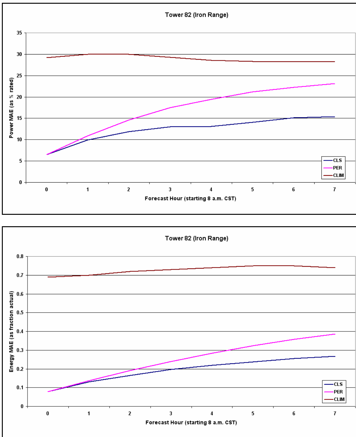
Figure 96: Power mean absolute error (top) and energy mean absolute error as a fraction of actual production (bottom) as a function of forecast hour for all months for the CLS, climatology (CLIM), and persistence (PER) forecasts for Tower 82 (Iron Range).
