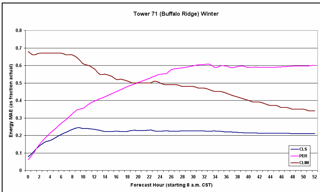
Figure 92: Power mean absolute error (top) and energy mean absolute error as a fraction of actual production (bottom) as a function of forecast hour for the winter months (Dec., Jan., Feb.) for the CLS, climatology (CLIM), and persistence (PER) forecasts for Tower 71 (Buffalo Ridge).
