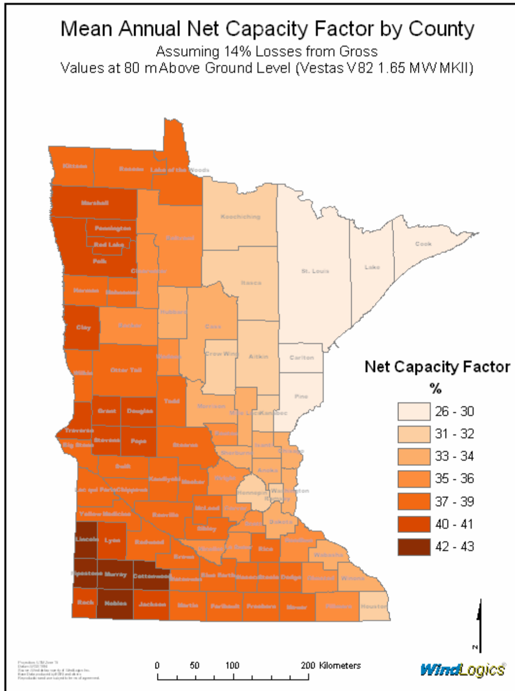
Figure 19: State mean annual net capacity factors by county.
