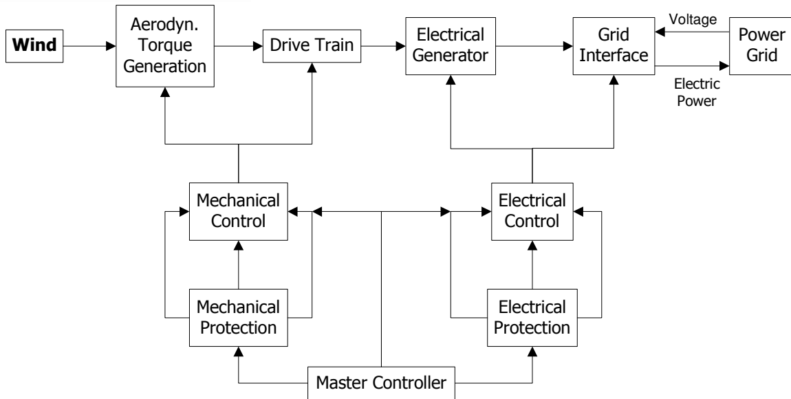
Figure 2: Generalized wind turbine model with control elements and hierarchy.
