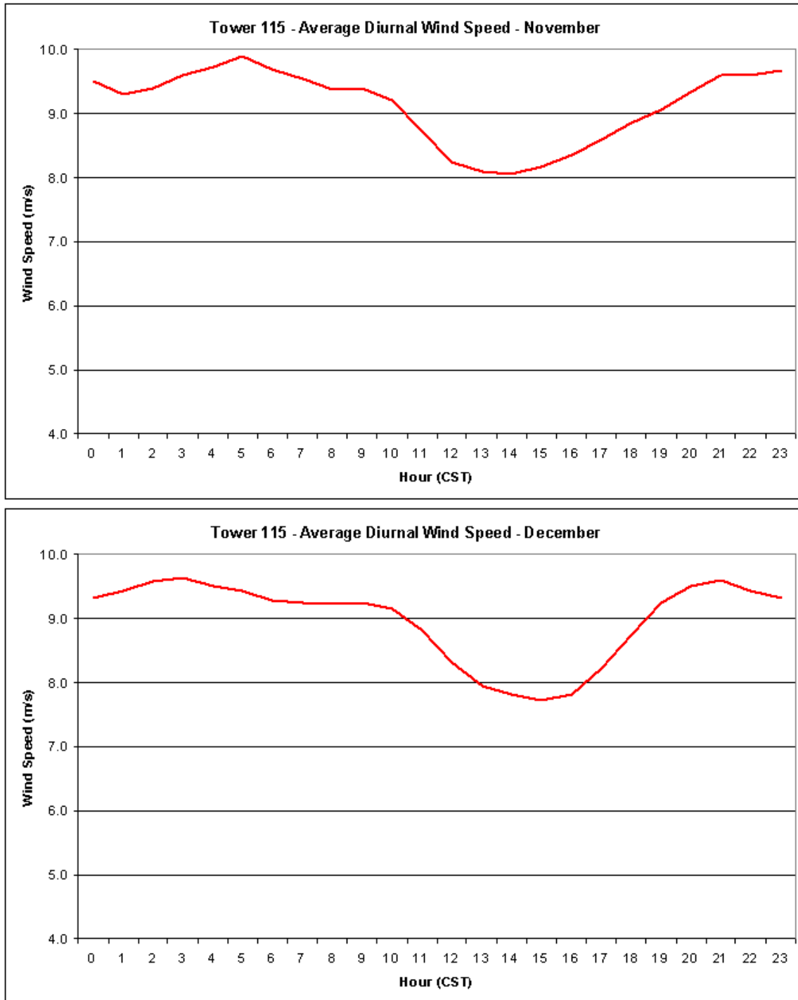
Figure 88: Average November and December 80 m diurnal wind speed at Tower 115 in m/s.
