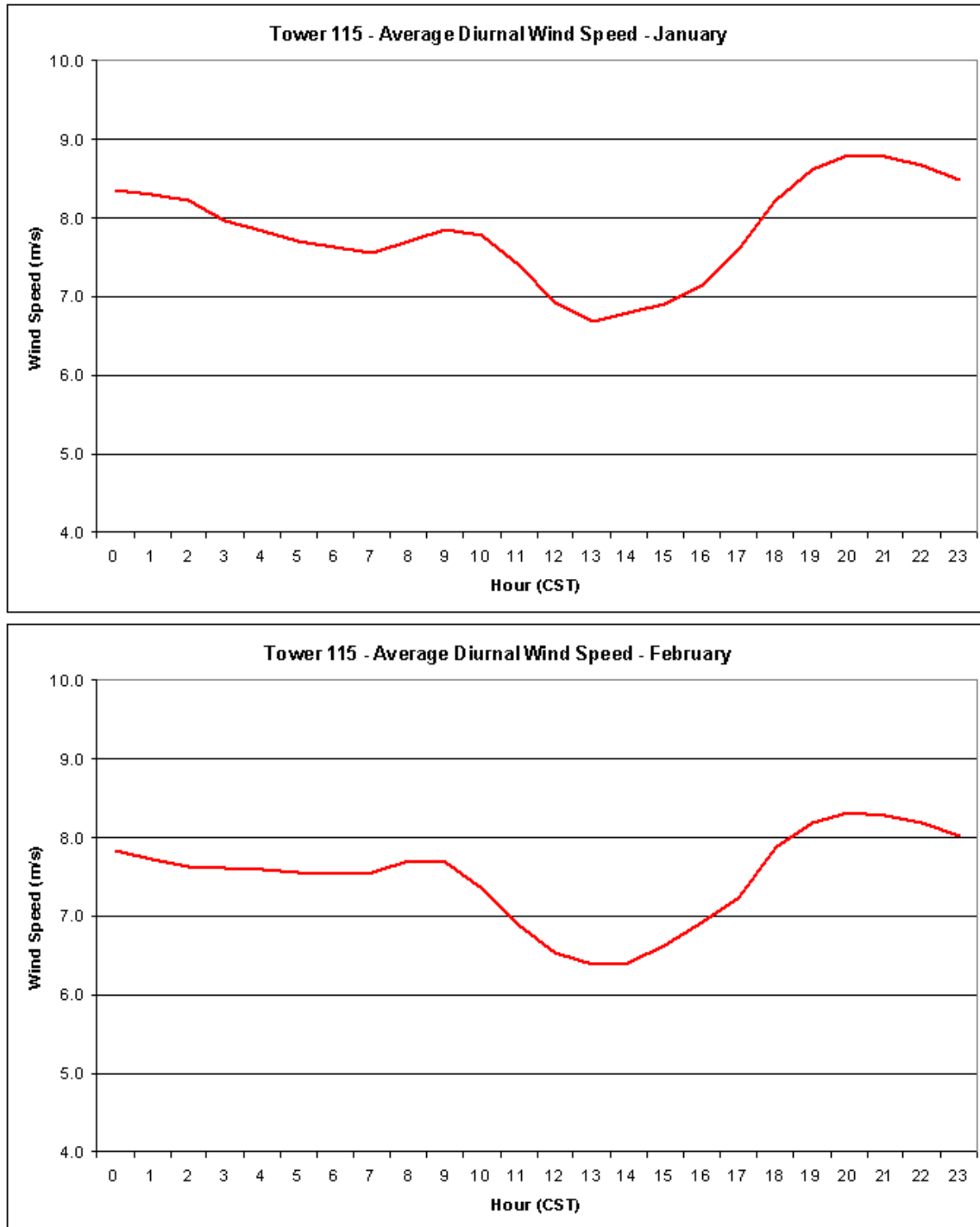
Figure 83: Average January and February 80 m diurnal wind speed at Tower 115 in m/s.
