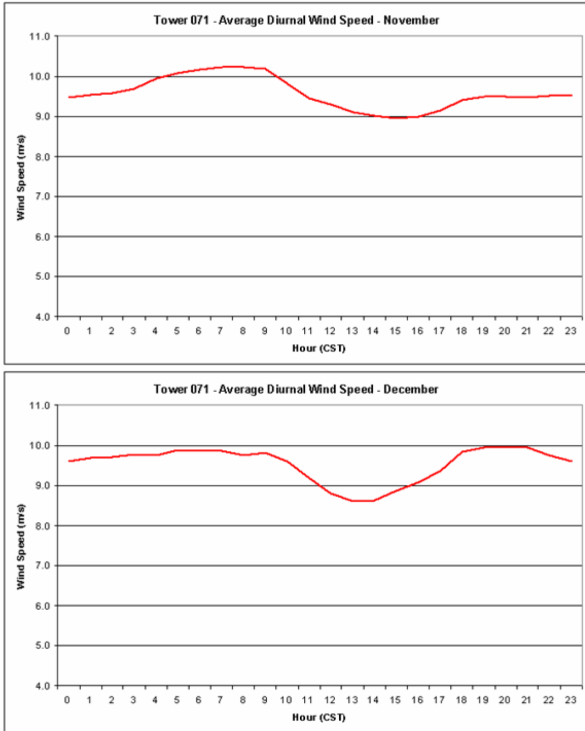
Figure 67: Average November and December 80 m diurnal wind speed at Tower 71 in m/s.
