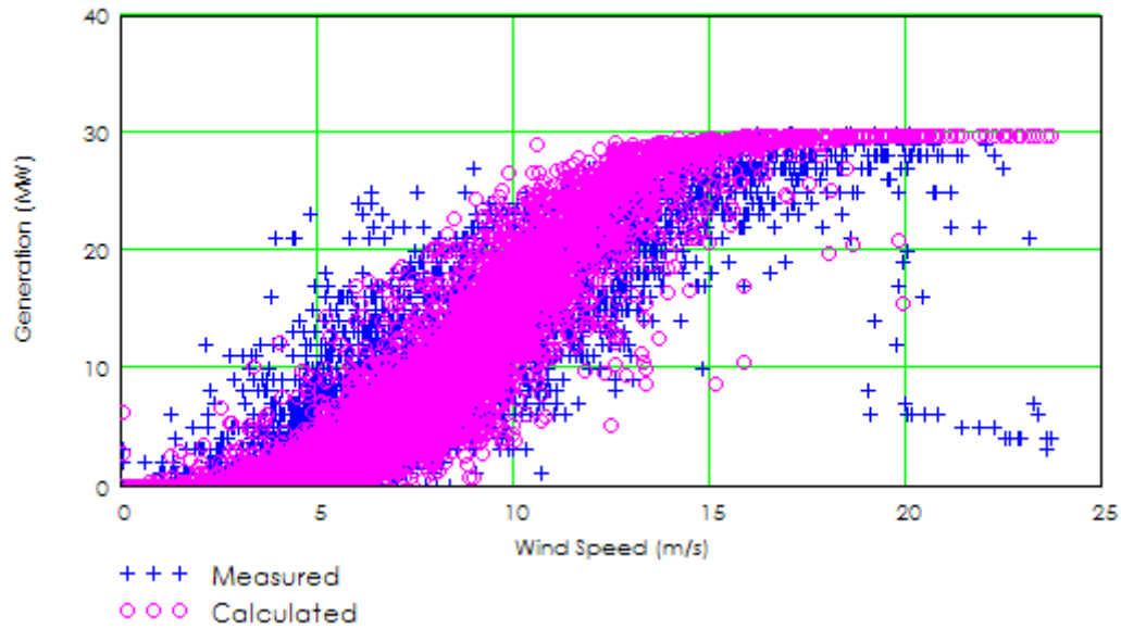
Figure 62: Measured and modified calculated plant power curves.
