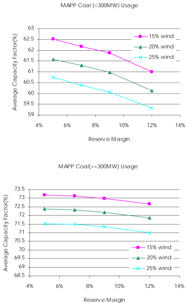
Figure 49: Coal unit capacity factor as functions of wind generation and operating reserve level
