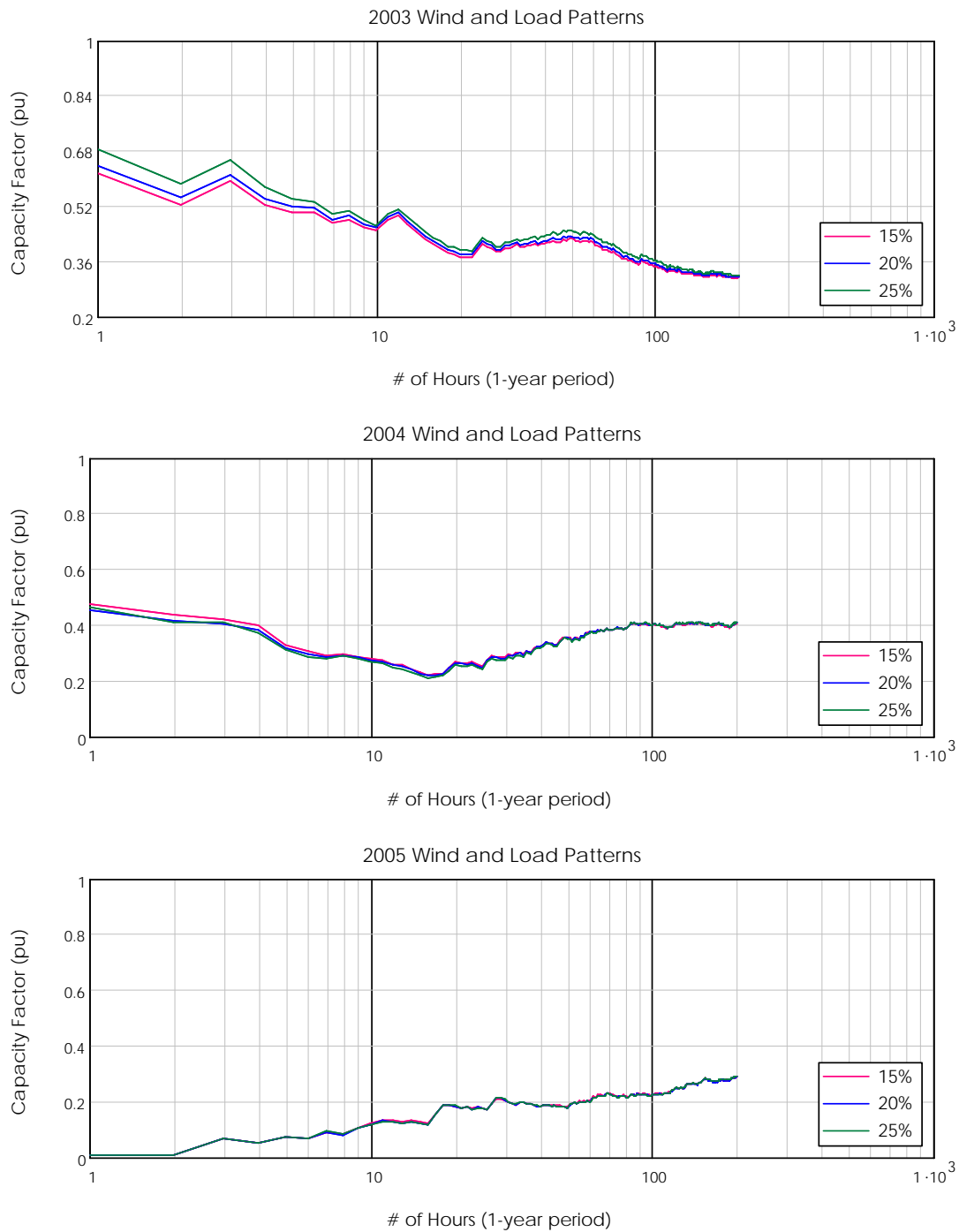
Figure 32: Wind generation capacity factor for varying number of highest load hours. (2003, 2004, and 2005 wind and load patterns)
