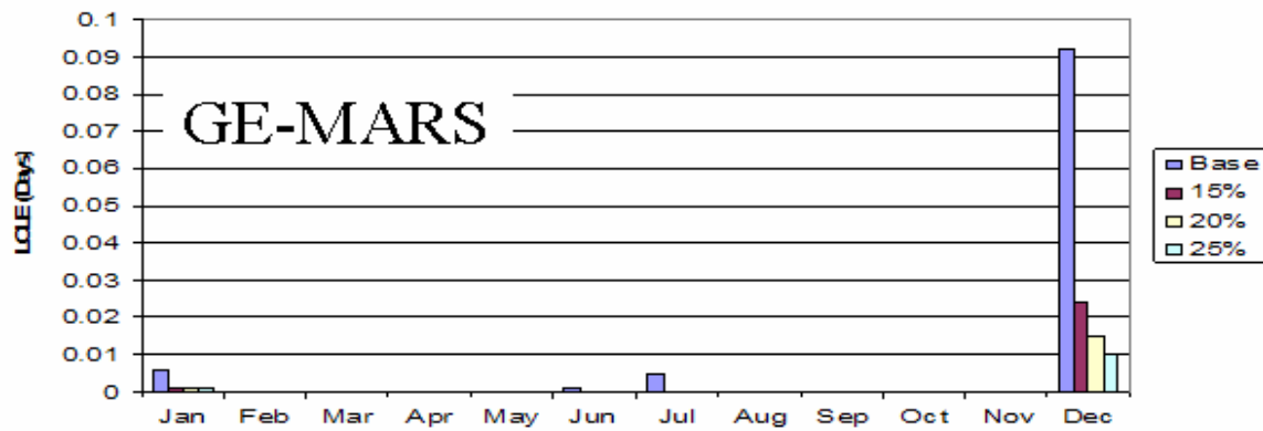
Figure 44: Weekly LOLP results for 2004 for GE-MARS and Marelli
