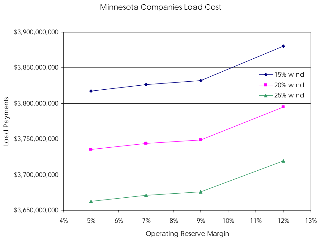
Figure 47: Load payments for Minnesota companies as a function of wind penetration and operating reserve level.
