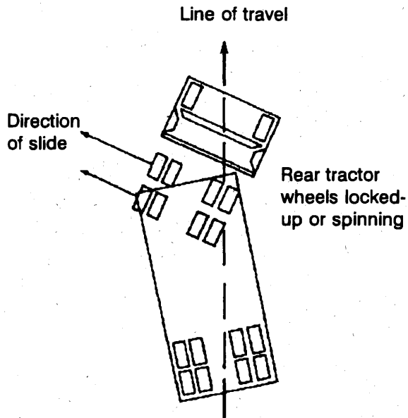
Figure 6-2 Tractor Jackknife
