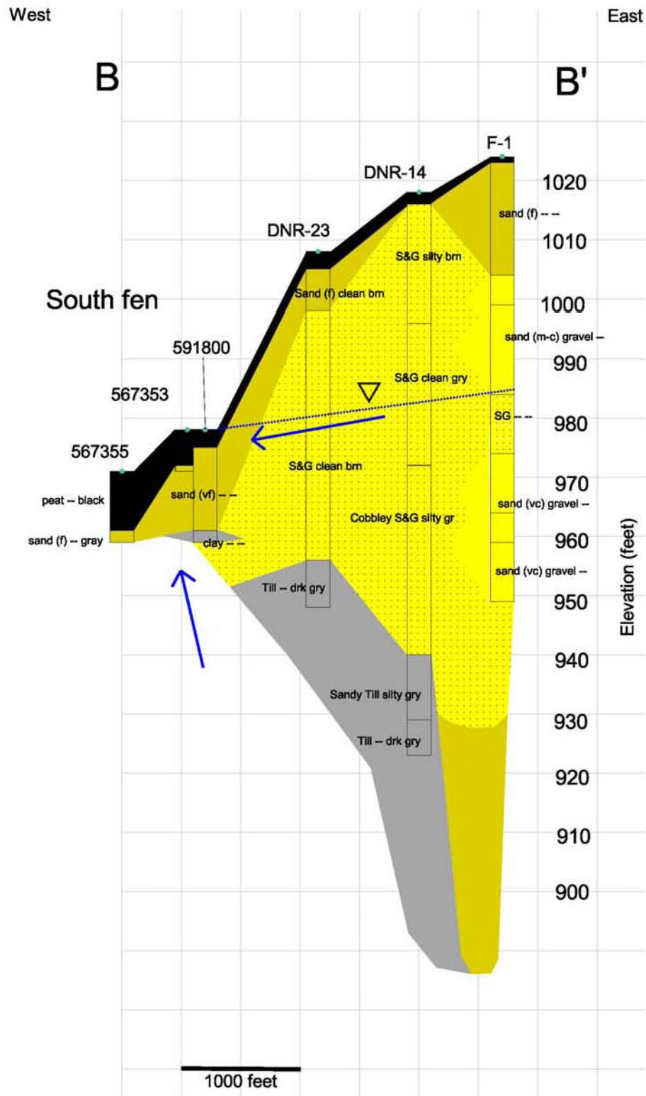
Figure 10.4. Geologic cross section along a trace from the South Fen to the height of the beach ridge south of the Trust Fund Pit.
