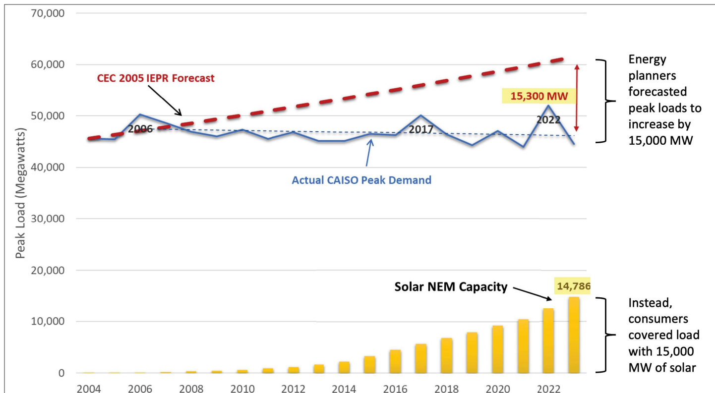
Figure 5. Customer Solar Compared to Load Deviation from Forecast
