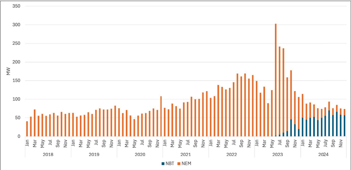
Figure 20. Residential Solar Installations by Installation Date
