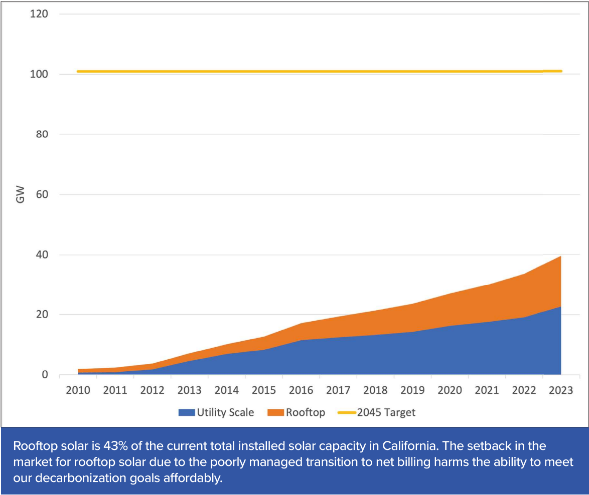
Figure 26. Solar Growth Needed to Decarbonize the Grid
