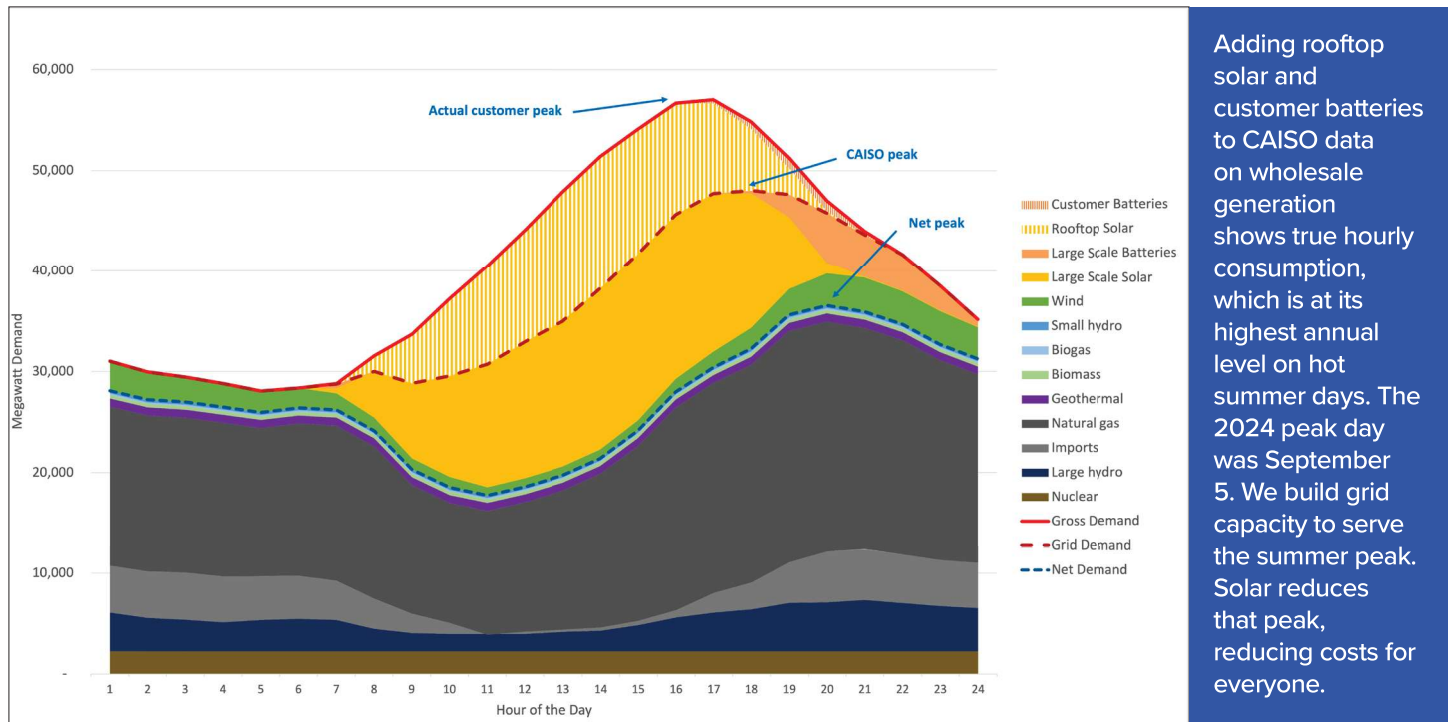
Figure 6. California Energy Sources Covering Actual Gross Peak Load
