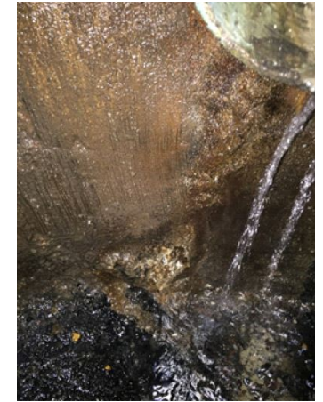
Infiltration at Manhole Structures
