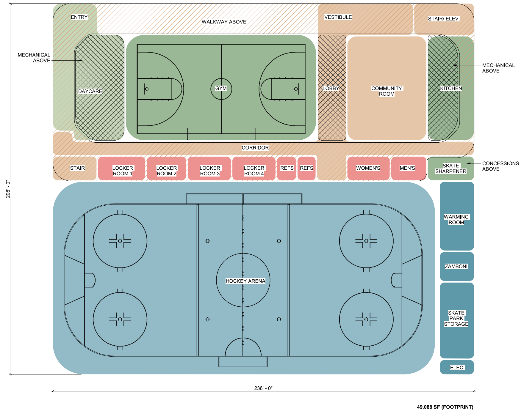
1 CONCEPT PLAN 1/16" = 1'-0"
