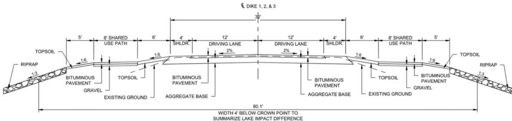
PROPOSED TYPICAL SECTION OPTION 3
