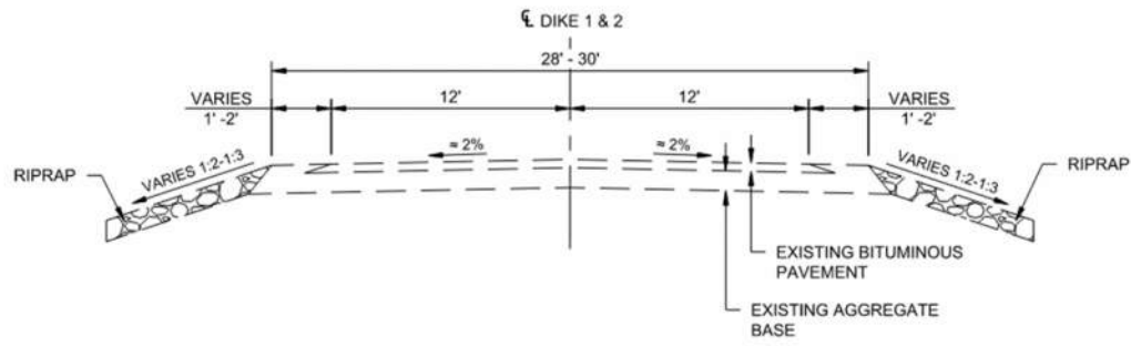
EXISTING TYPICAL SECTION DIKE 1 & 2
